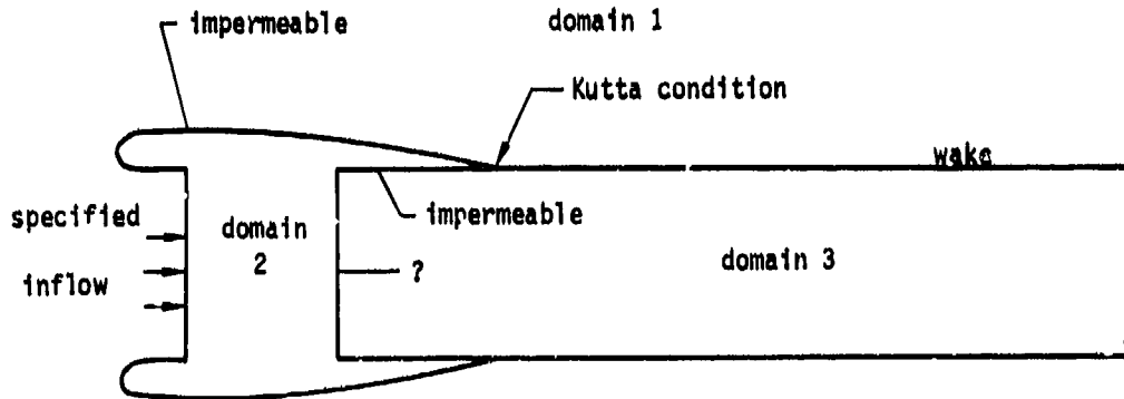
(b) nacelle with controlled inflow and outflow
