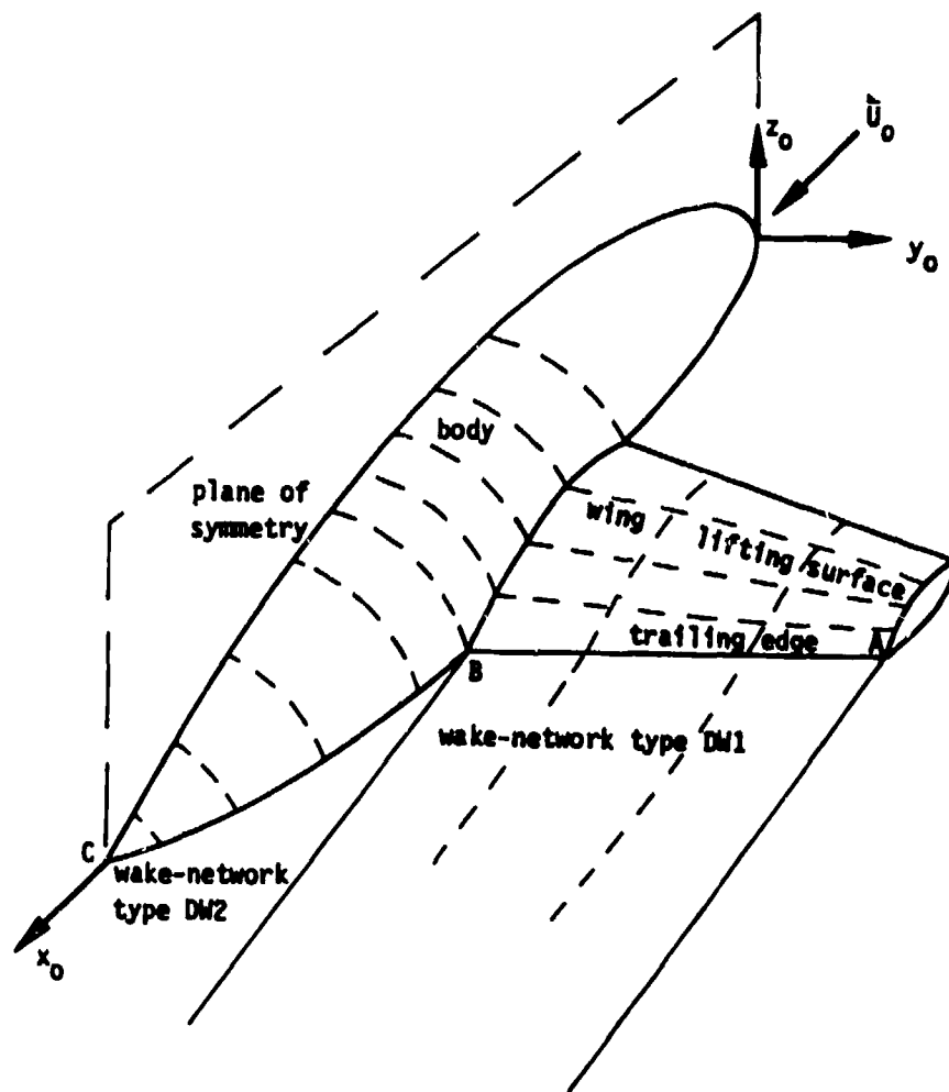
Figure 3.6 - Example of use of wake networks
