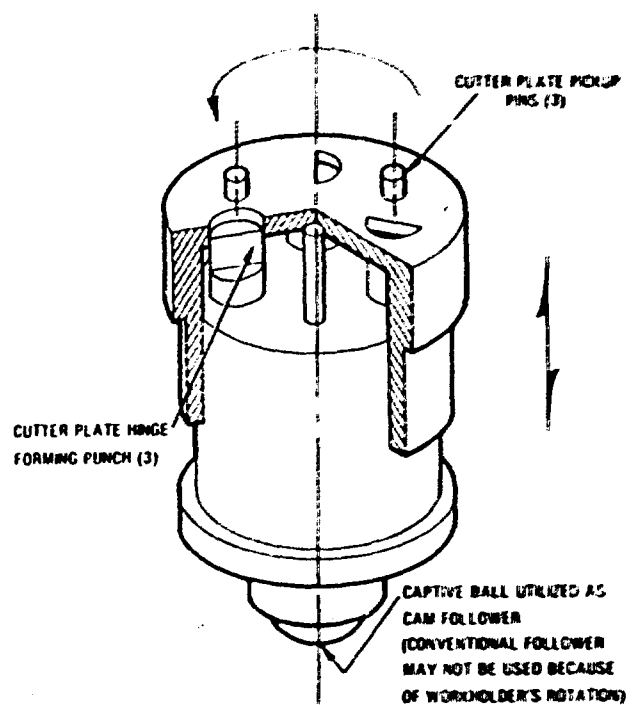
Figure IV-6. Cutter assembly—workholder.
