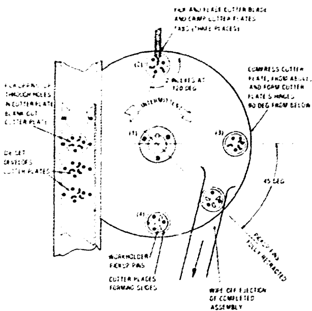
Figure IV-5. Cutter assembly.
