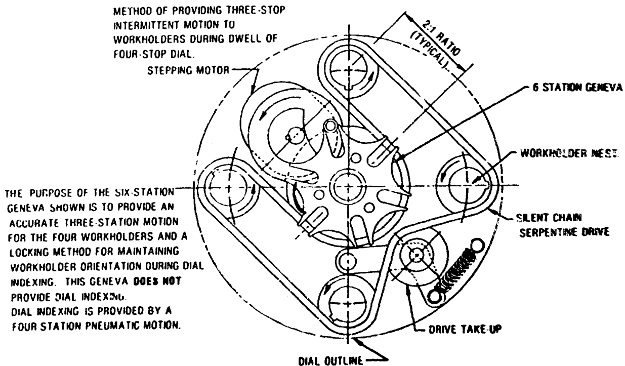
Figure IV-7. Cutter assembly workholder mechanics.
