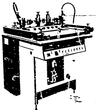
Figure V-13. Screen printer.
