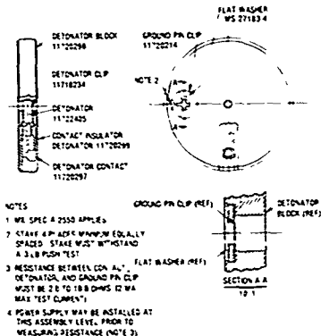
Figure II-3. Detonator block assembly (PN11722620) for XMS87E2/M724 fuze.
