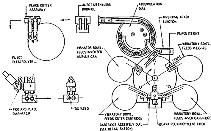
Figure IV-4. Mechanized ampule assembly.
