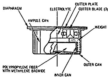
Figure IV-3. Ampule assembly.
