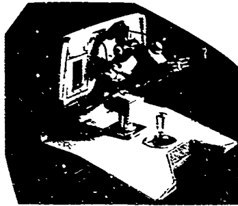
Figure VII-17. TC wire bonder.
