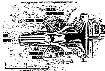
Figure IV-18. Fluidic generator for environmental sensor.
