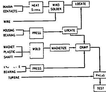
Figure IV-19. Turbine alternator process flow chart.
