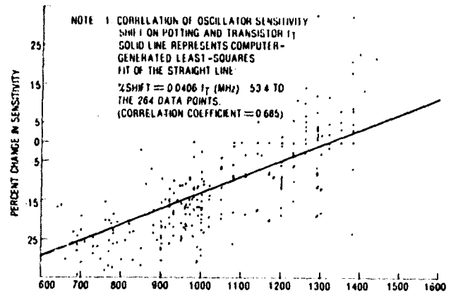
Figure VIII-9. Correlation between sensitivity change after potting and transistor f_T data obtained from HDL.
