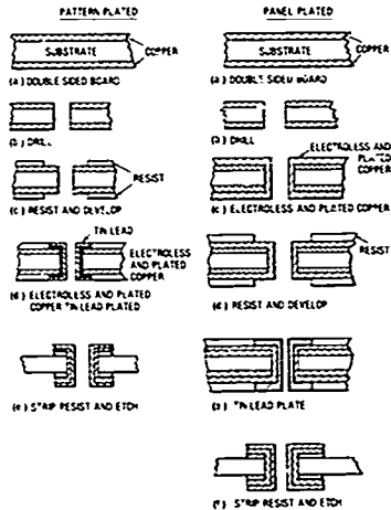
Figure V-2. Plated-through holes.
