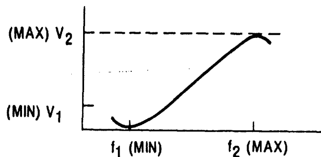
Figure VIII-8. Discriminator output.
