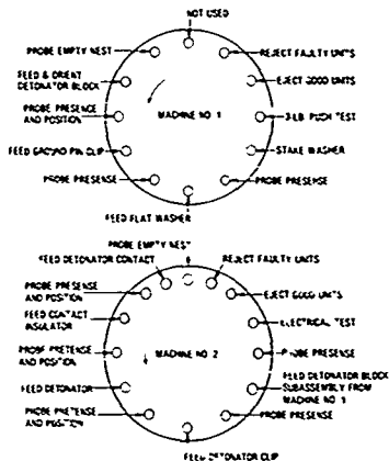
Figure 11-4. Operations for automatic assembly and test of PN 11722620.
