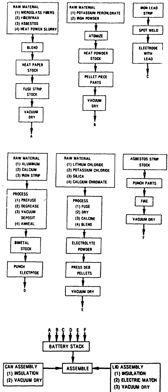
Figure IV-14. Thermal battery assembly.
