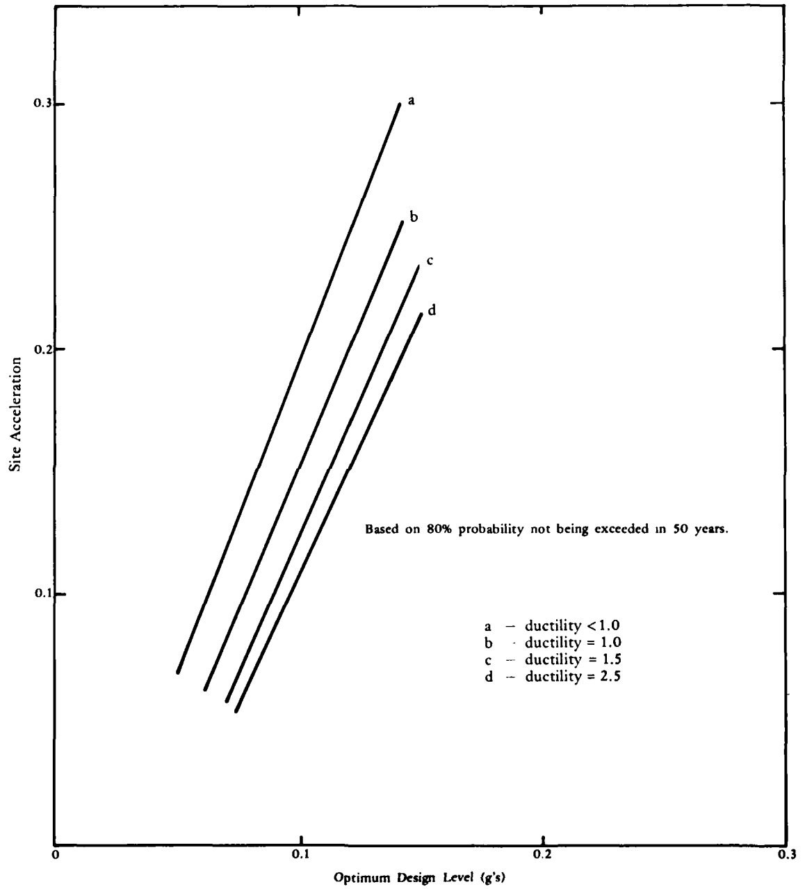
Figure 25. Design acceleration discounting future damage.
