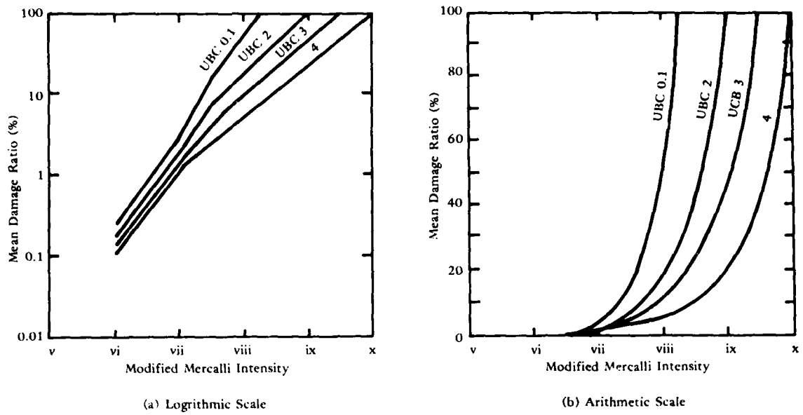
Figure 1. Damage estimate for different design strategies (after Ref. 10).
