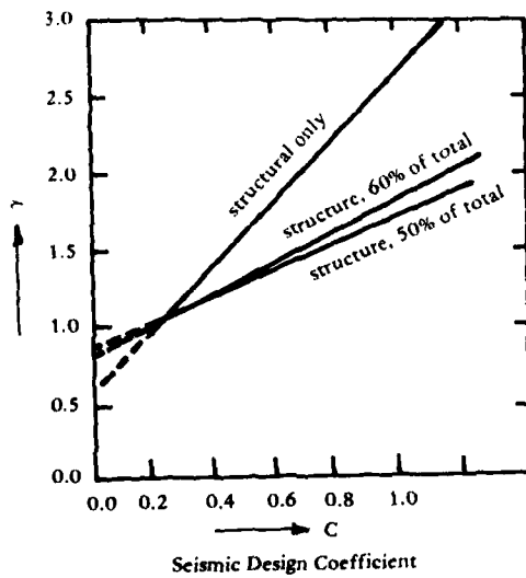
(a) Steel frame.
