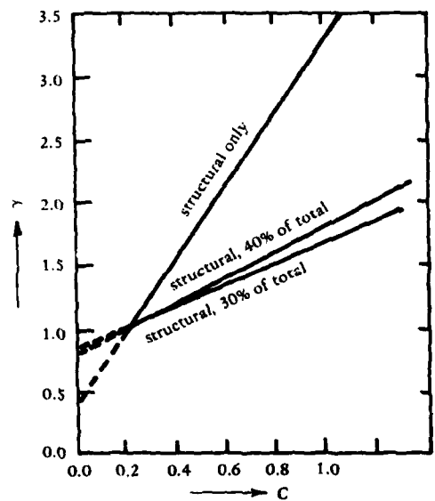
(b) Reinforced concrete ( N=5 , n=\infty in both directions, no aseismic shear walls)
