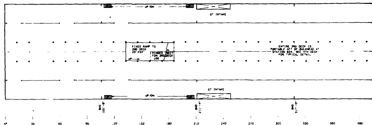
3RD DECK (CAR DECK) 58' ABL
