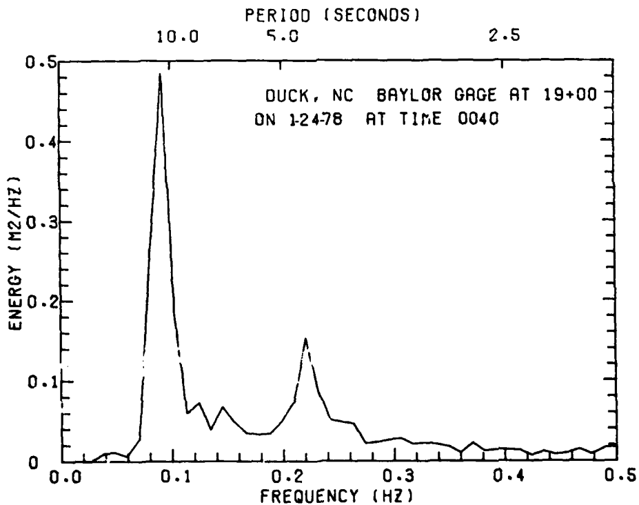
Figure 32. Example of spectrum plot.
