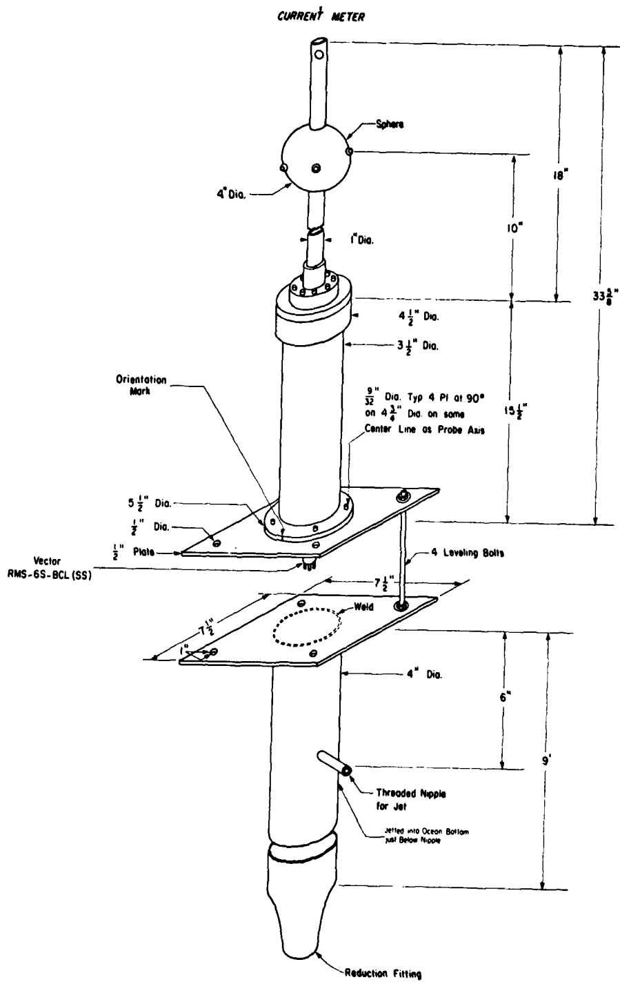
Figure 9. Current meter installation.
