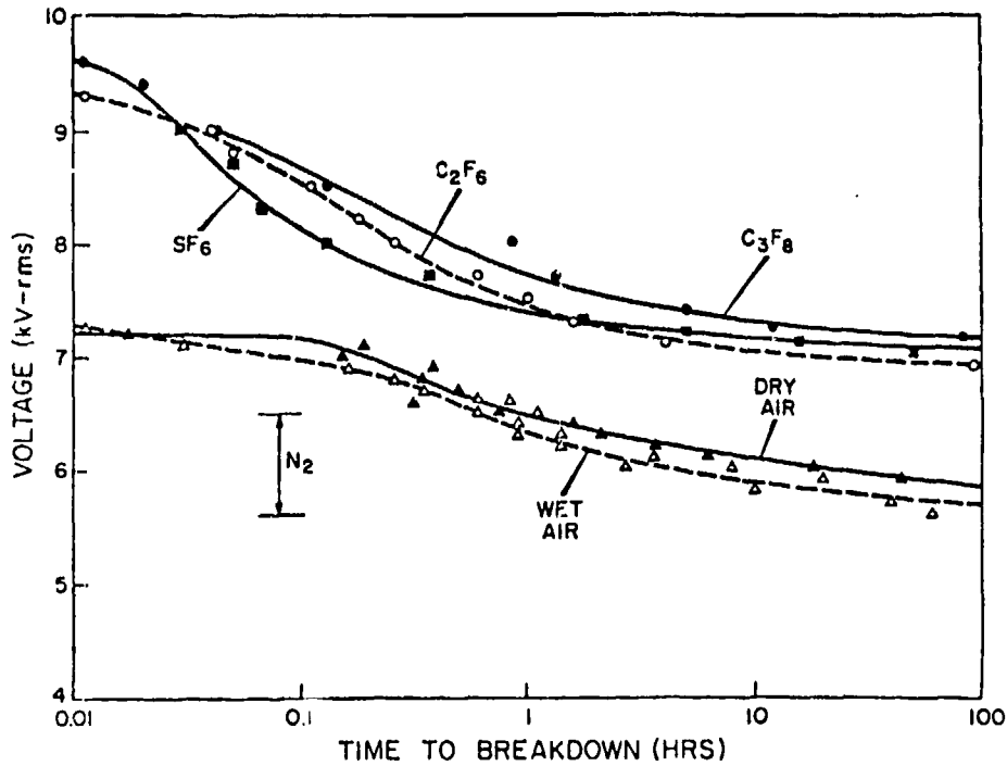
Fig. 5 - Voltage endurance functions for 0.635-cm thickness PZT ceramic in various insulator gases
