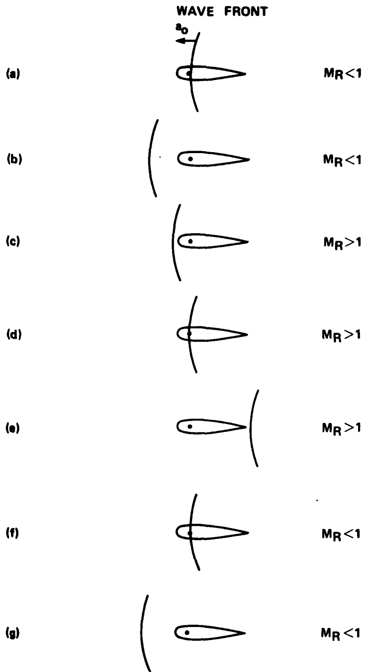
Figure 18. Relative position between wavefront and blade.
