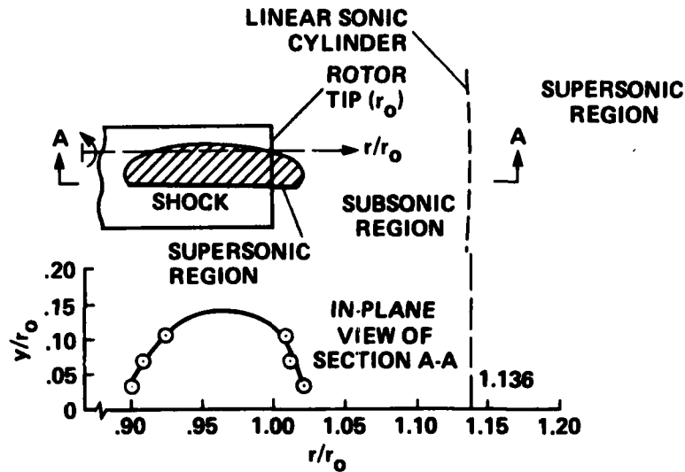
Figure 5. Top and aft views of shock boundaries of a rotor, M_{tip} = 0.88 .
