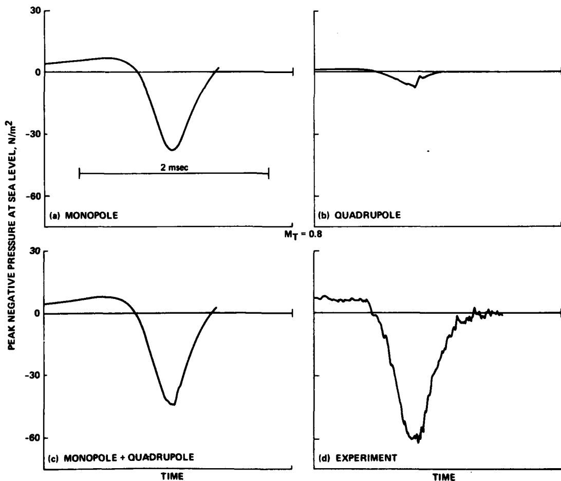
Figure 11. Theory-experiment comparison, M_{tip} = 0.8 .
