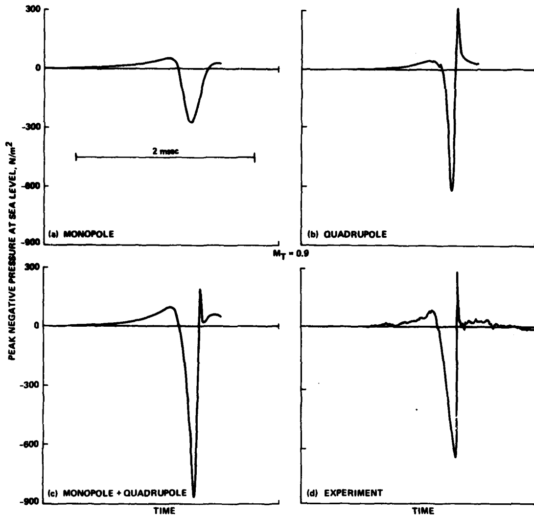
Figure 13. Theory-experiment comparison, M_{tip} = 0.90 .
