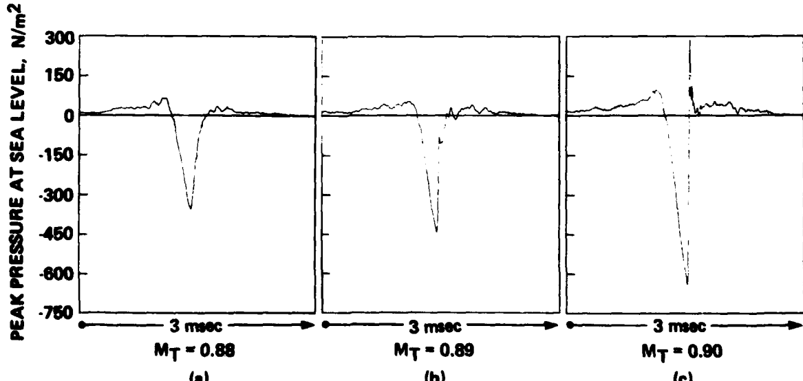
Figure 3. Waveform transition; the development of a radiating discontinuity, in-plane, r/D = 1.5 , M_{tip} = 0.9 .
