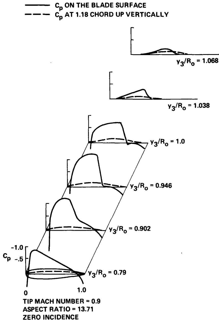
Figure 7. C_p distribution on the blade surface and at 1.18 chords up, aspect ratio = 13.7, NACA 0012, near zero angle of attack, M_{tip} = 0.9 .
