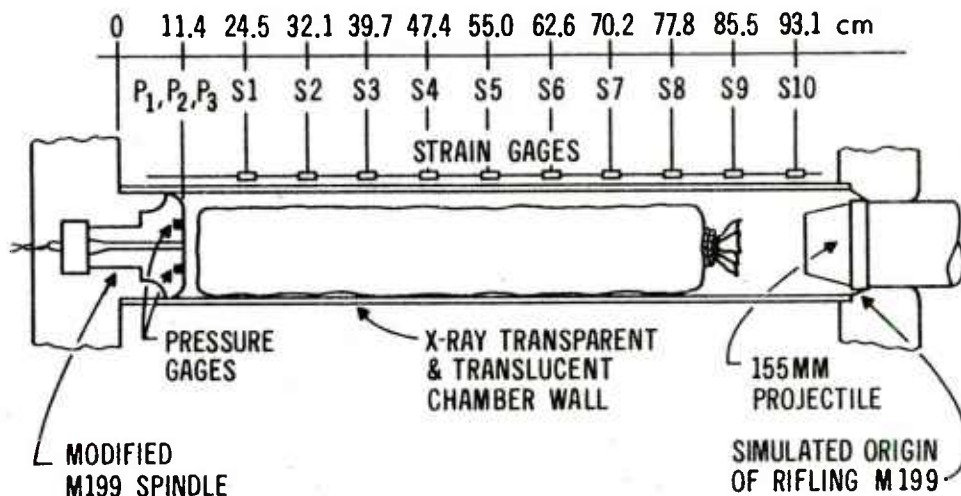
Figure 20. Schematic of 155-mm Fiberglass Chamber
