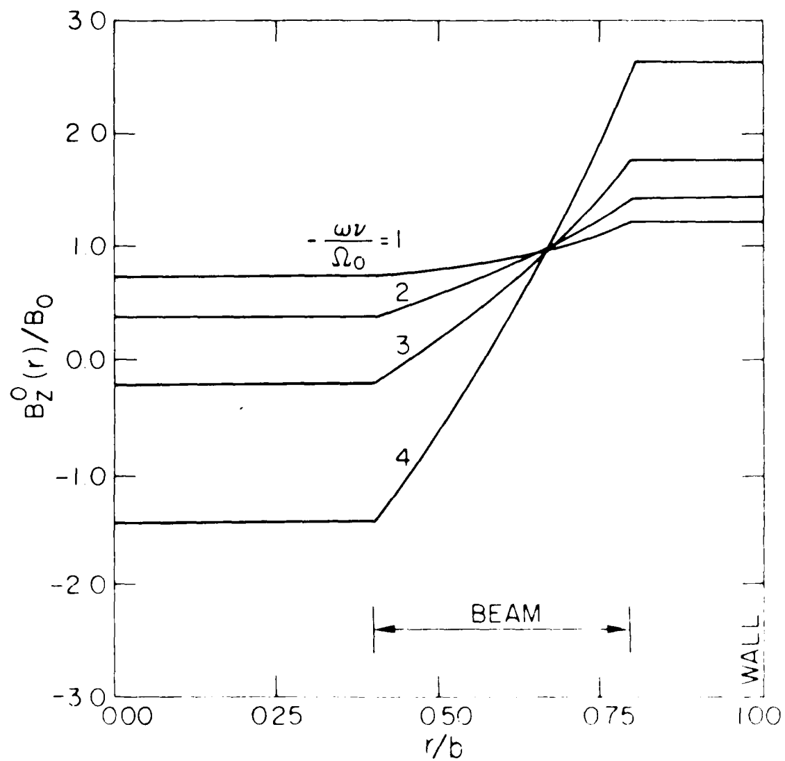
Figure 9 - Equilibrium magnetic field profiles for various values of the parameter -\frac{\omega v}{\Omega_0} . The ratios a/b and a_1/b are equal to 0.8 and 0.4 respectively.
