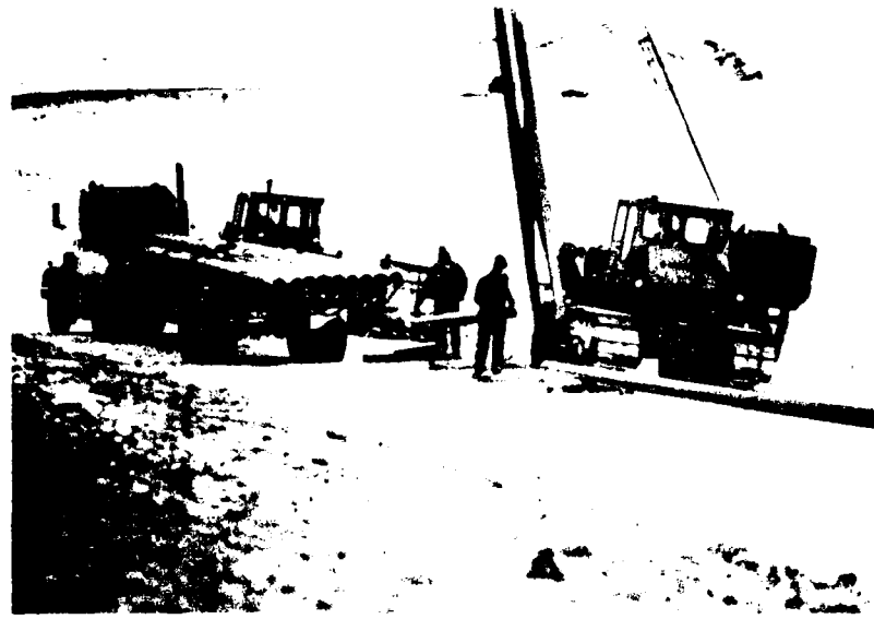
Figure 23. Stringing the pipe on the gasoline snow pad.
