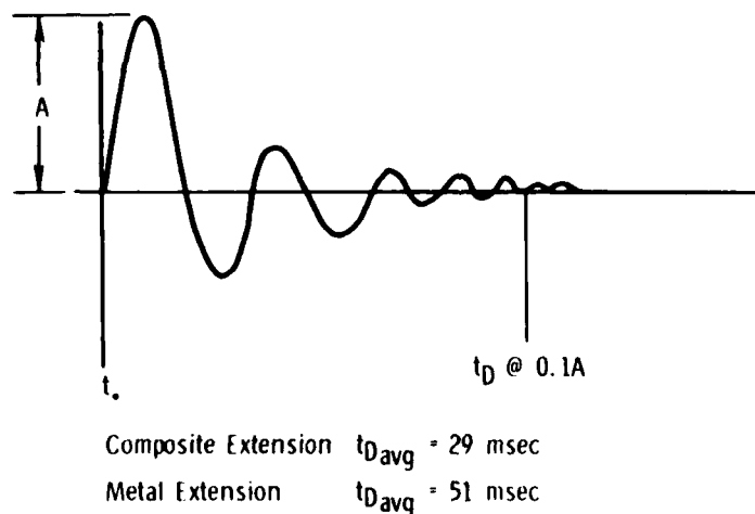
Figure 12. DAMPING HISTORY
