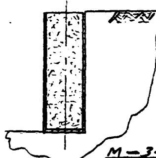
M-3- EARTH-FILLED FRP-PIPE OR RECT. BOX WALL
