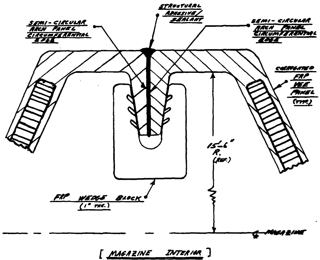
FIGURE 5.3 CONNECTION BETWEEN ADJACENT ARCH PANEL EDGES
