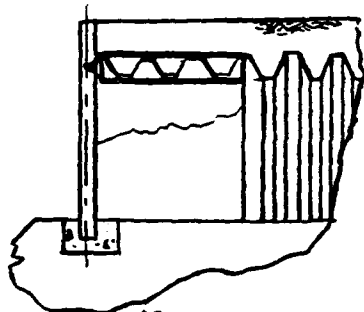
M-4- SEMI-CIRC. ARCH END PANEL WITH FRP SHEETS RODED TO FORM BOX CURVED FOR FR WALL SUPPORT
