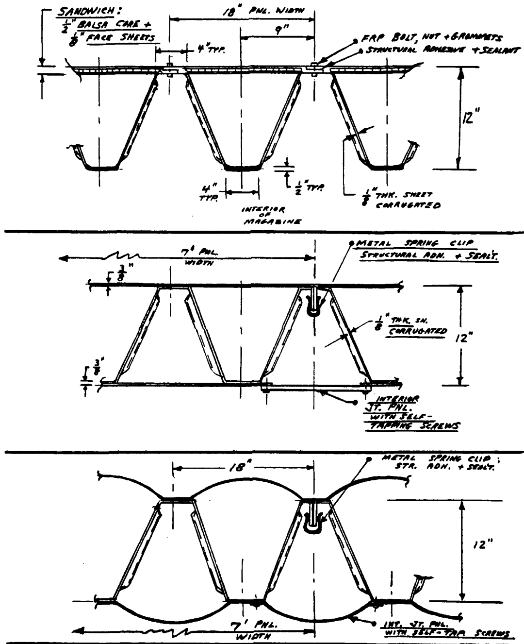
FIGURE 4.2 SH 3 OF 4 ALTERNATES TO SECTION A-A ON SH. 2
