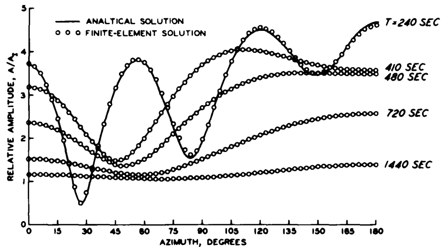
Figure 5. Comparison of finite-element solution with analytical solution
