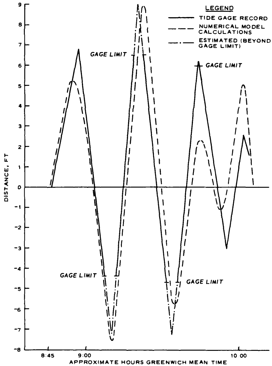
Figure 7. 1964 tsunami at Kahului, Maui
