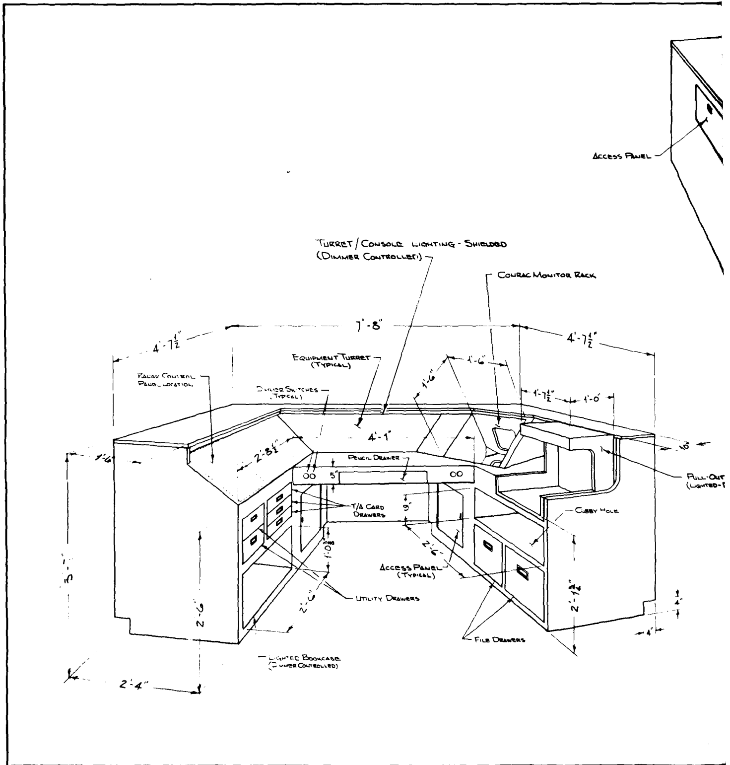
FIGURE 11. SCHEMATIC OF BRADLEY TRACON WING
