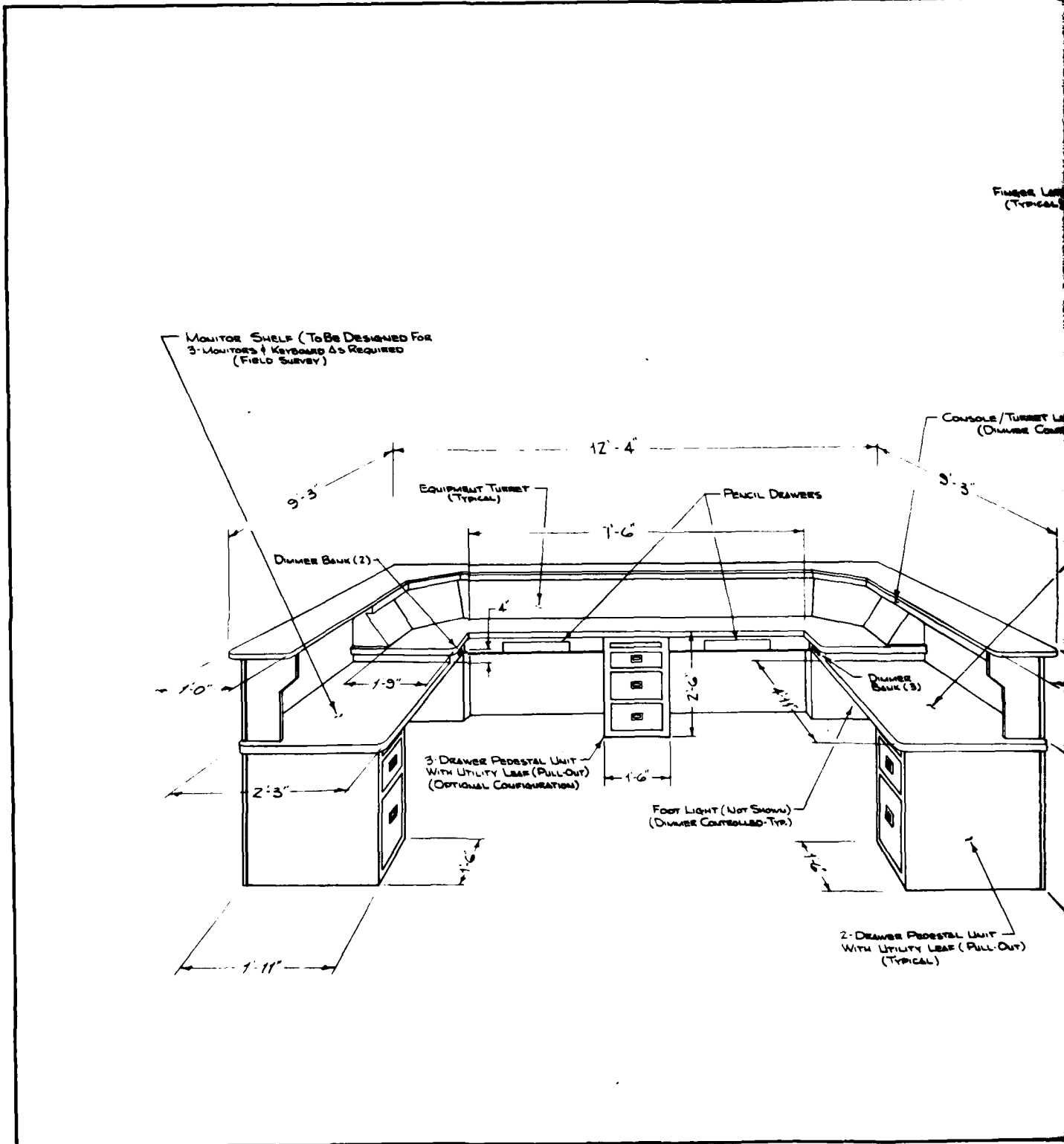
FIGURE 17. SCHEMATIC OF LARGE "U" SHAPE D
