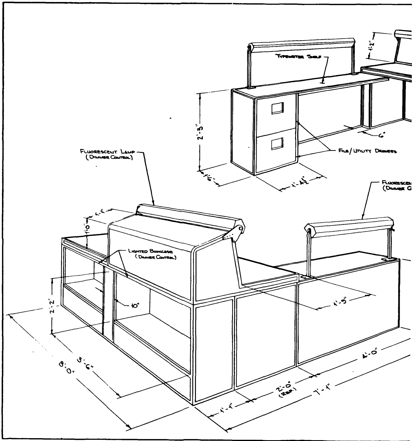
FIGURE 13. SCHEMATIC OF ALL METAL "L" SHA
