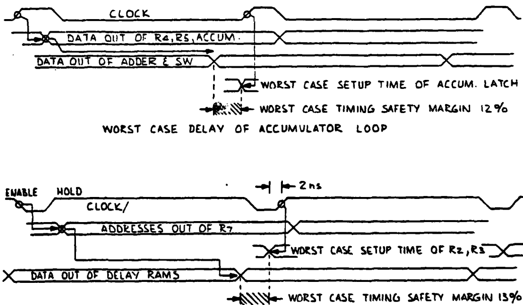
Figure 3-1. Delay and Coefficient RAM Outputs
