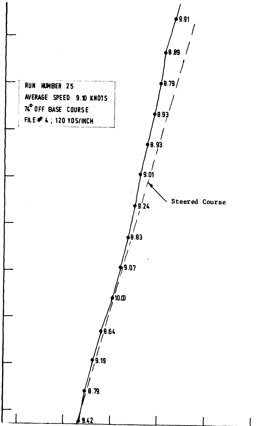
Figure 35 - Ship Course Deviation as Determined by Mini-Ranger (Run 25)
