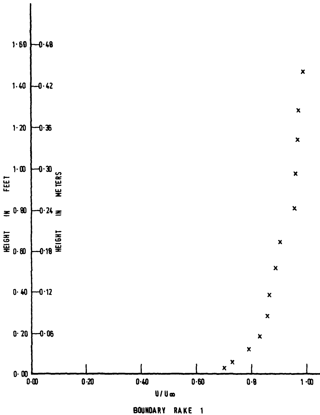
Figure 53 - Non-Dimensional Boundary Layer Velocity Profile of Rake 1
