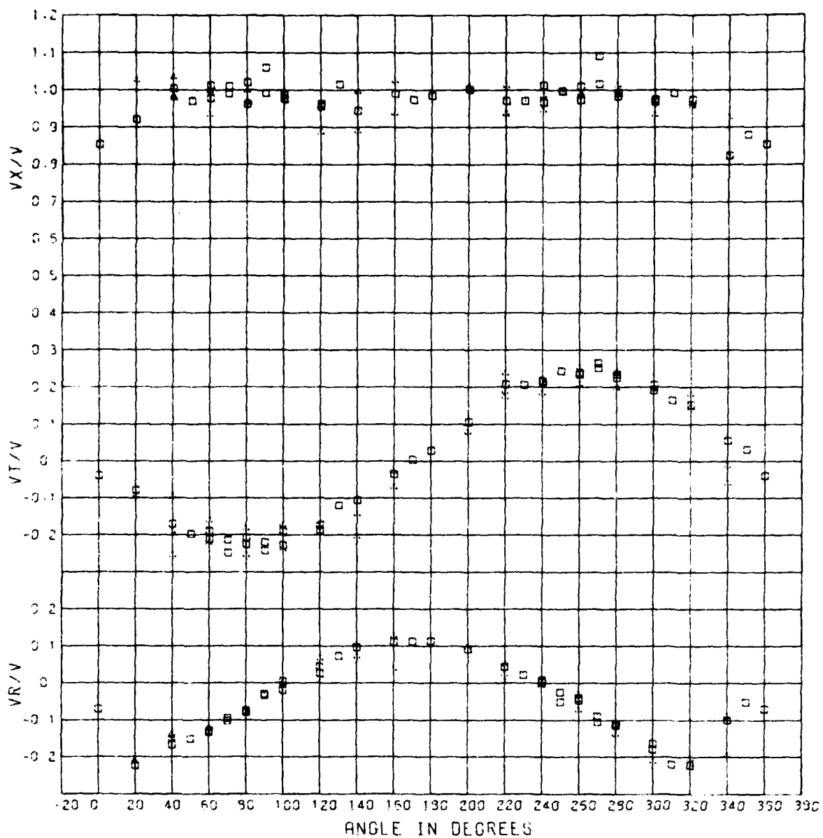
▲ VELOCITY COMPONENT RATIOS FOR RUNS 12-33, STBD FORWARD RAKES □ VELOCITY COMPONENT RATIOS FOR RUNS 34-51, STBD FORWARD RAKES (Forward Plane on Shaft Without Propeller) 0.417 RAD.
