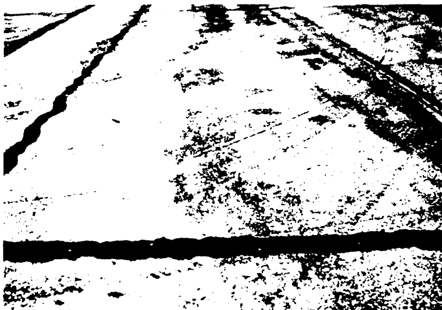
Figure B-31. Low severity joint reflection cracking, filled crack
