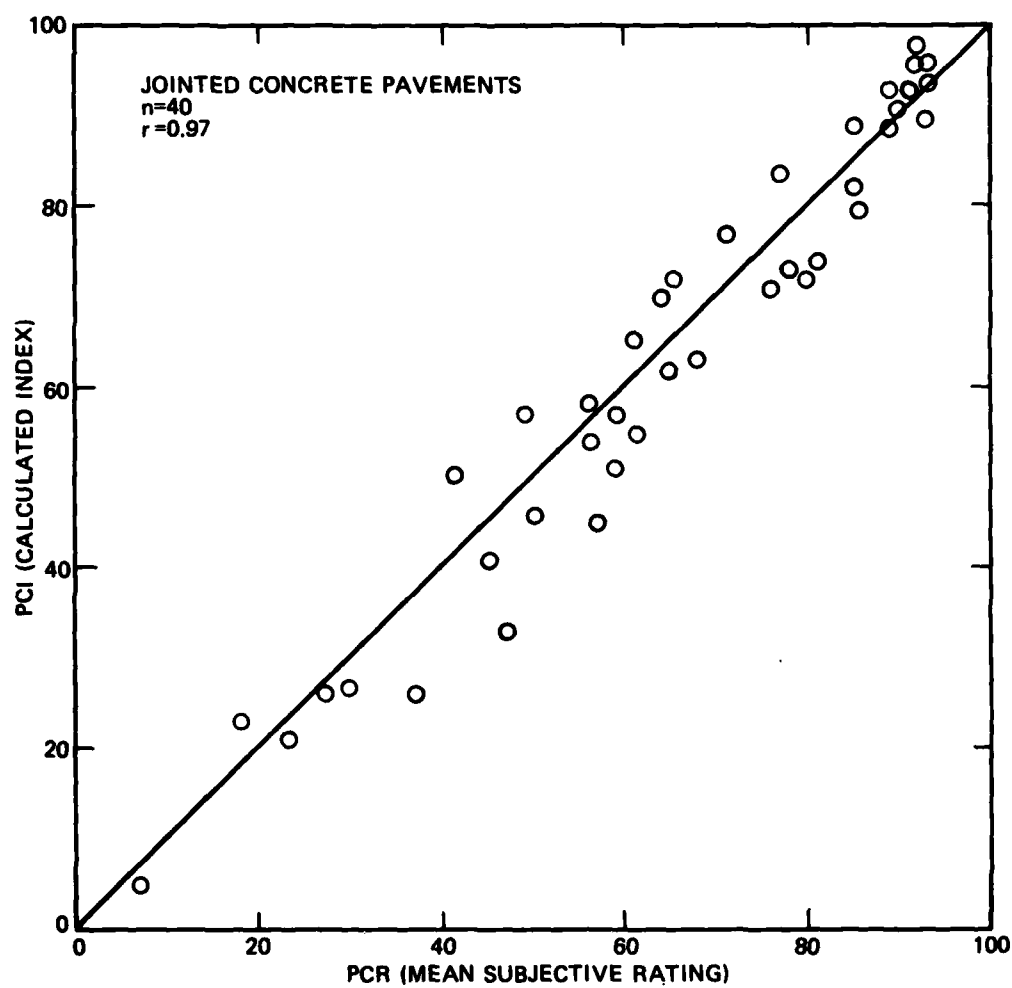
Figure 6. Correlation between PCR and PCI for jointed rigid pavement sections surveyed
