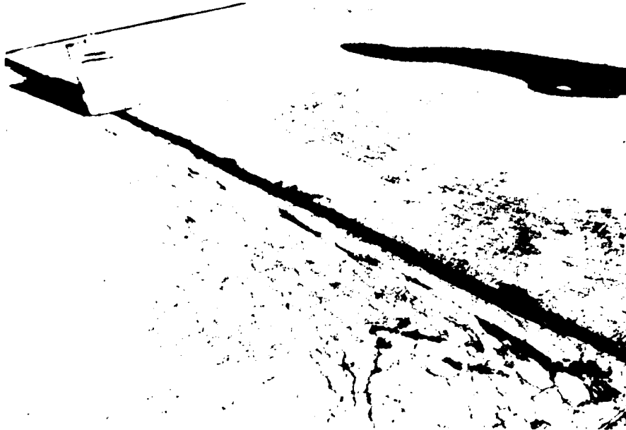
Figure B-90. High severity "D" cracking (This condition exists over more than one-quarter of the slab.)
