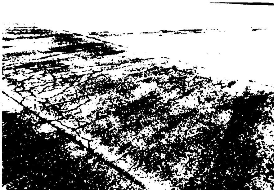
Figure B-8. Medium severity alligator cracking, approaching high severity, case 2
