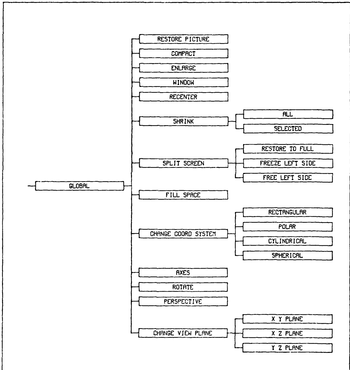
FIGURE 4.13. THE STAGING MODIFY PICTURE TREE
