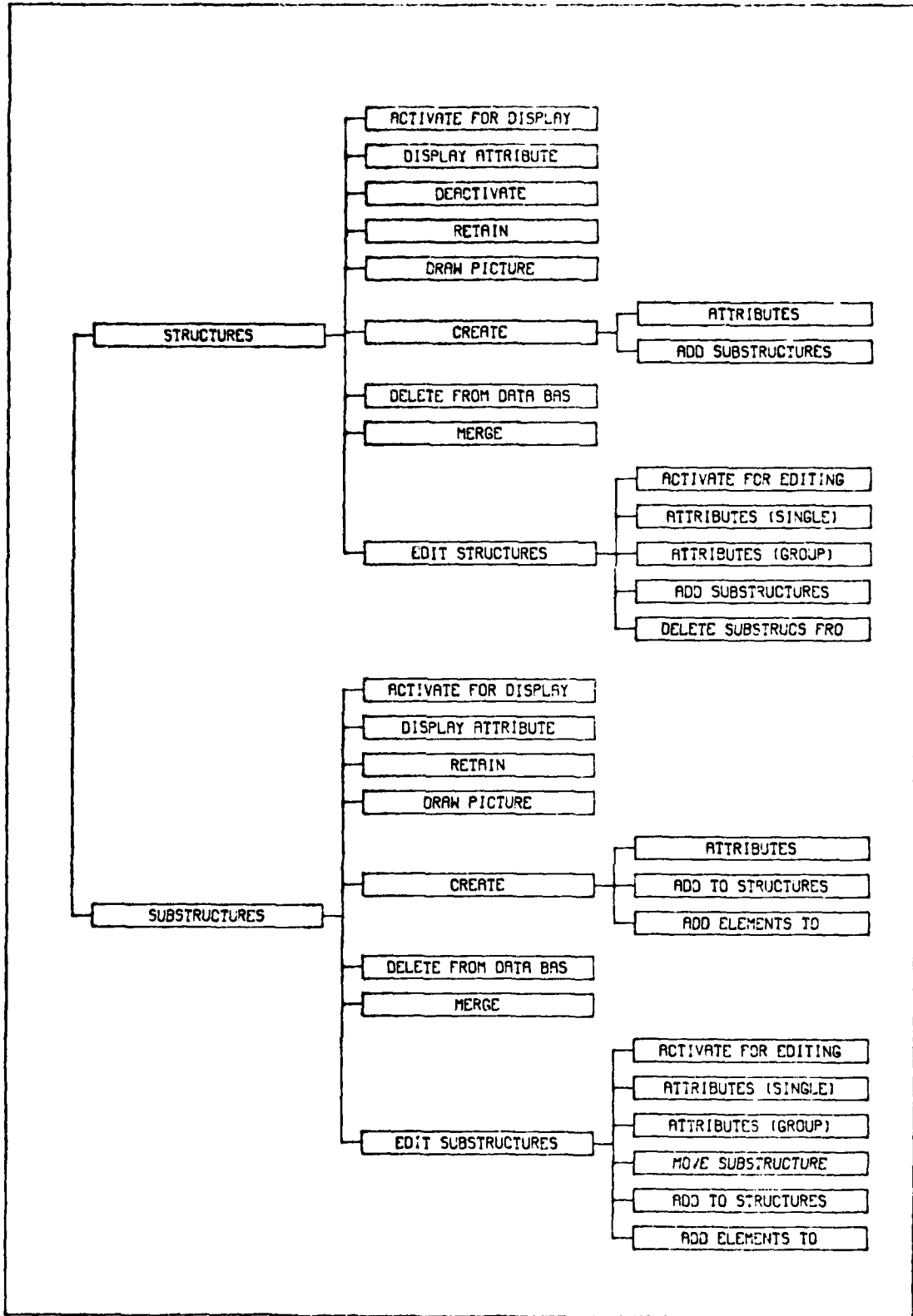
FIGURE 5.2.a. THE STAGING EDIT TREE
