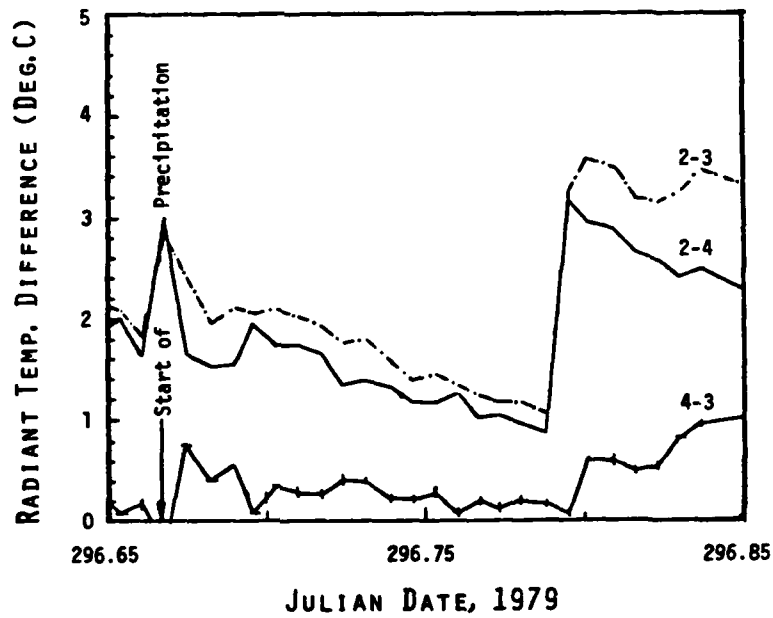
Figure 6. Radiant temperature differences determined from the data of Figure 5.
