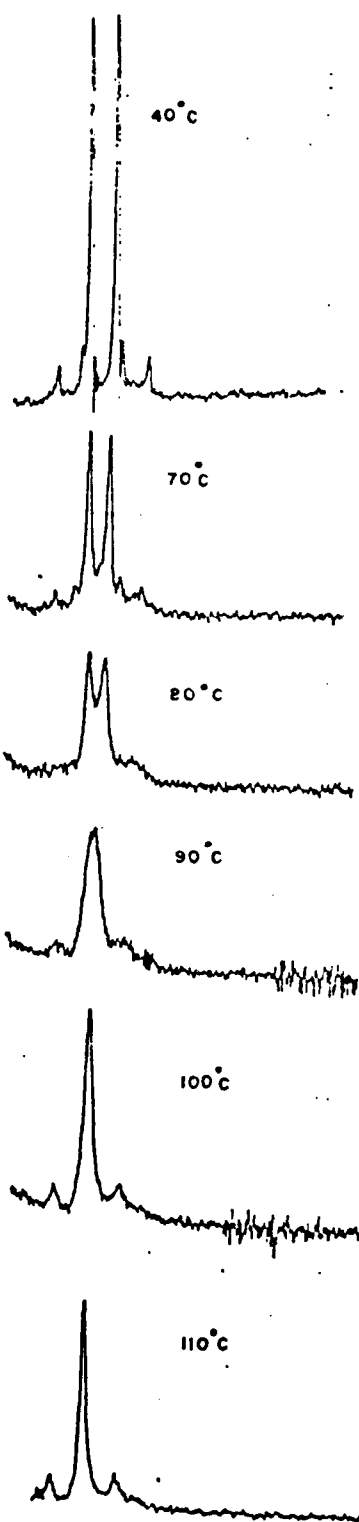
Figure 1. Variable temperature proton NMR spectrum of lithium 1,1-dicyclopentadienyl-1-bromo-2,3,4,5-tetraphenylstannole in toluene at 60 MHz.
