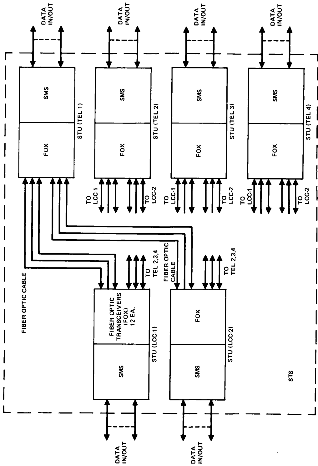
Figure 2. Signal transfer system functional block diagram.
