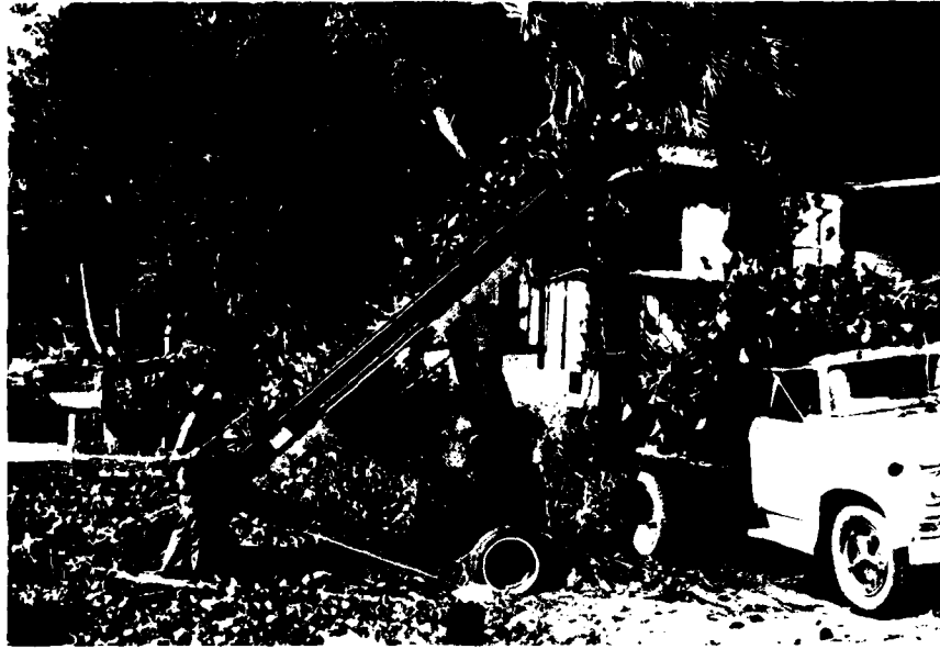
a. Side view of wheel-mounted aquatic plant removal conveyor-elevator system in operation
