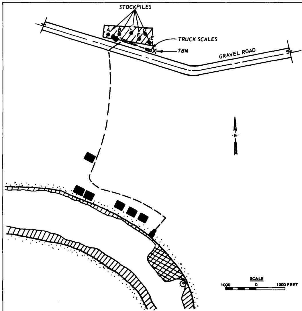
Figure 21. Layout of hyacinth disposal test stockpiles
