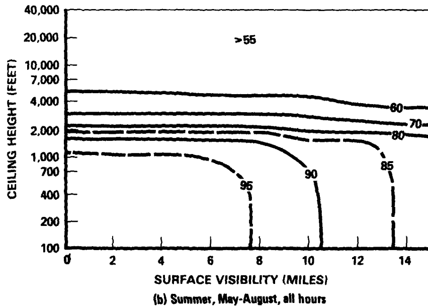
Fig. 21—Percent Frequency that Concurrent Ceiling and Visibility Values Are Equaled or Exceeded at Kirkenes
