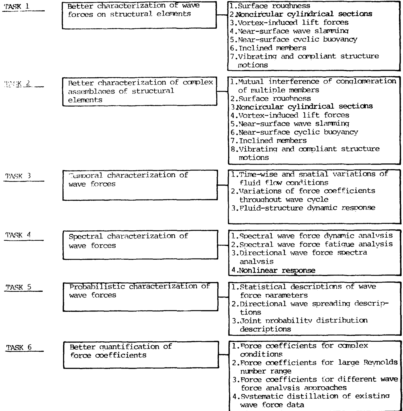
FIGURE 5.2 RESEARCH NEEDS FOR IMPROVING AND EXPANDING THE MORISON EQUATION
