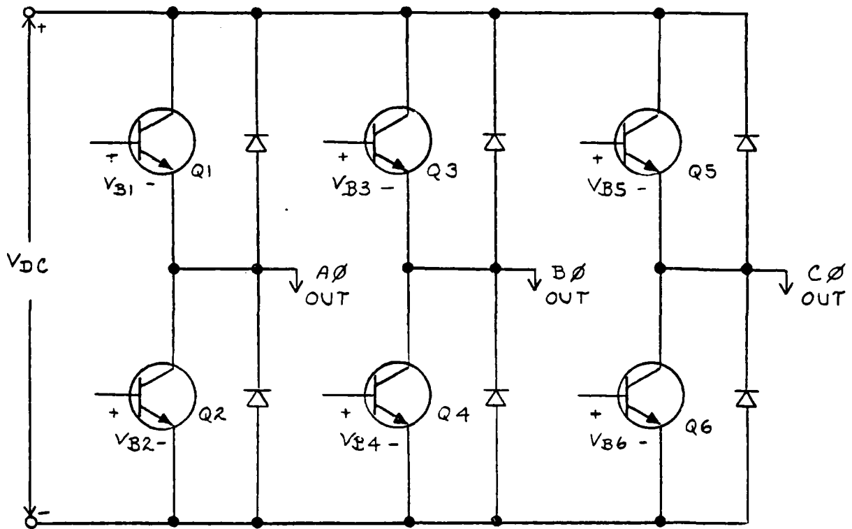
FIGURE 3-4A BASIC INVERTER
