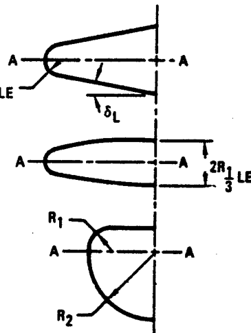
FIGURE 20 INPUT FOR NAMLIST LARWB - LOW ASPECT RATIO WING, WING-BODY INPUT
