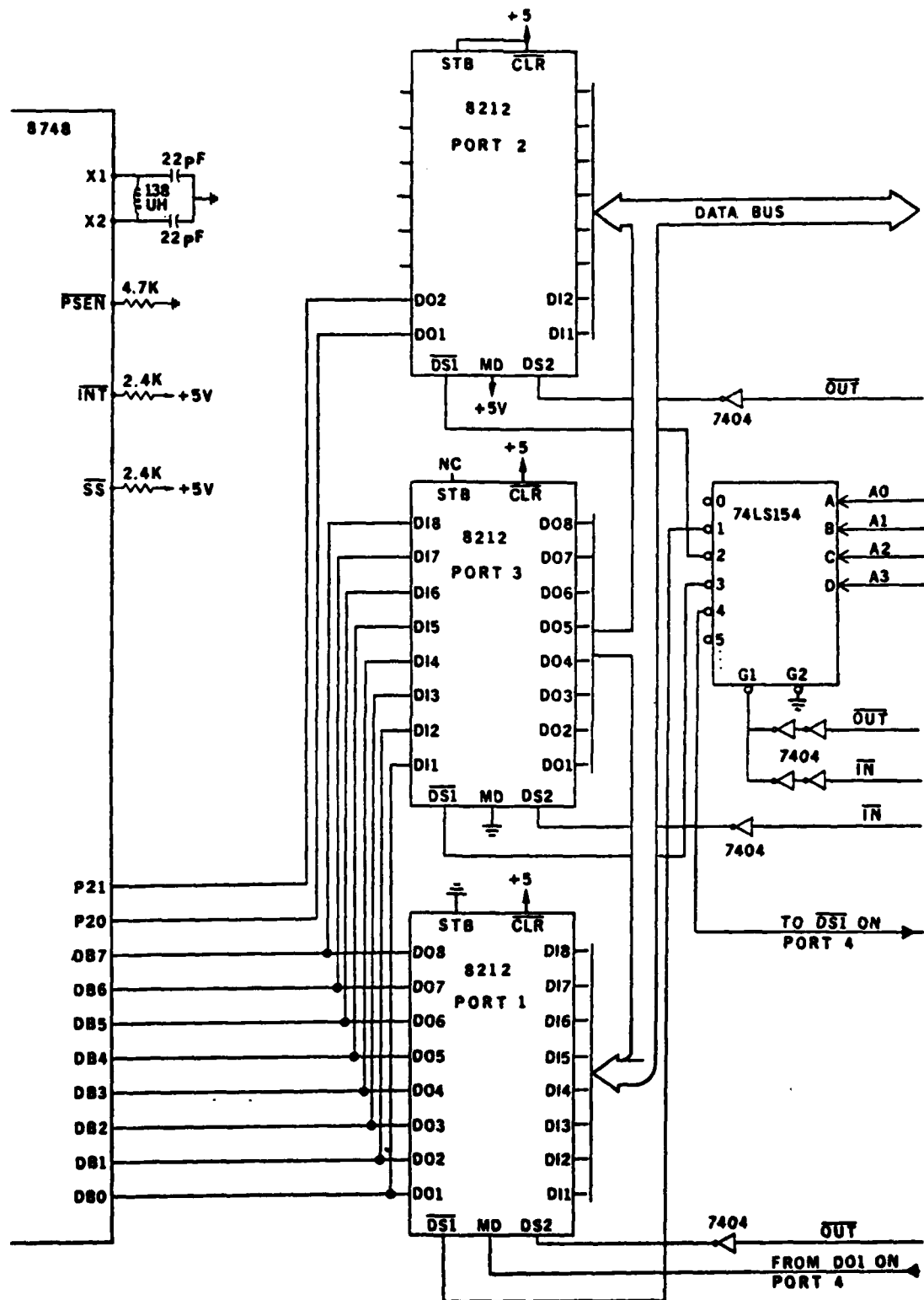
Figure 8 - Programmer Schematic
