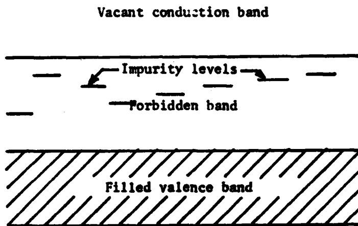
FIGURE 4. Band picture of solids.
