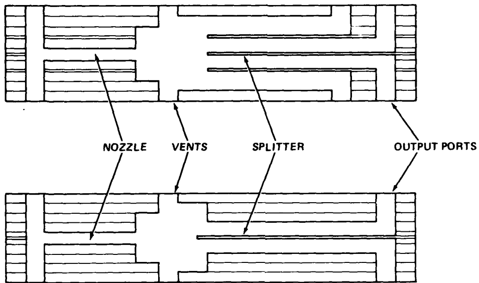
Figure 35. Vertically laminated fluidic amplifiers (after C. D. O'Neal, U.S. Patent 3,468,331, 23 September 1969).
