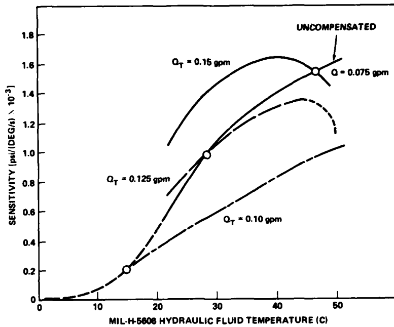
Figure 29. Temperature compensation of laminar jet angular rate sensor (LJARS): normalized splitter length = 20, supply width = 0.75 mm, aspect ratio = 2.5, and shunt resistance = 7 × LJARS supply resistance.
