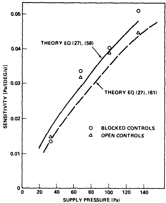
Figure 51. Experimental sensitivity as function of supply pressure.
