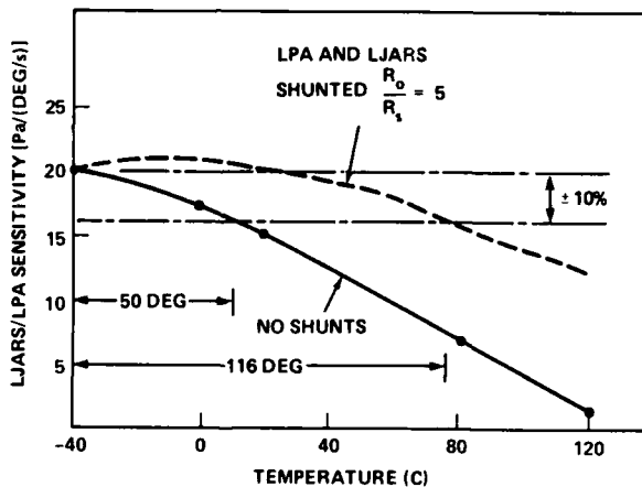
Figure 31. Temperature compensation by capillary shunt resistance of subsystem of laminar jet angular rate sensor (LJARS) and laminar proportional amplifier (LPA).
