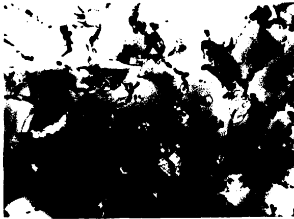
FIGURE 7 DARK ROD-LIKE PHASE IS \text{CO}_2\text{Al}_9 WHICH SEGREGATED AT GRAIN BOUNDARIES IN AL-8.4ZN-2.5MG-1.0CU-0.8 CO ALLOY AFTER HOT COMPACTION AT 700°F (371°C)
