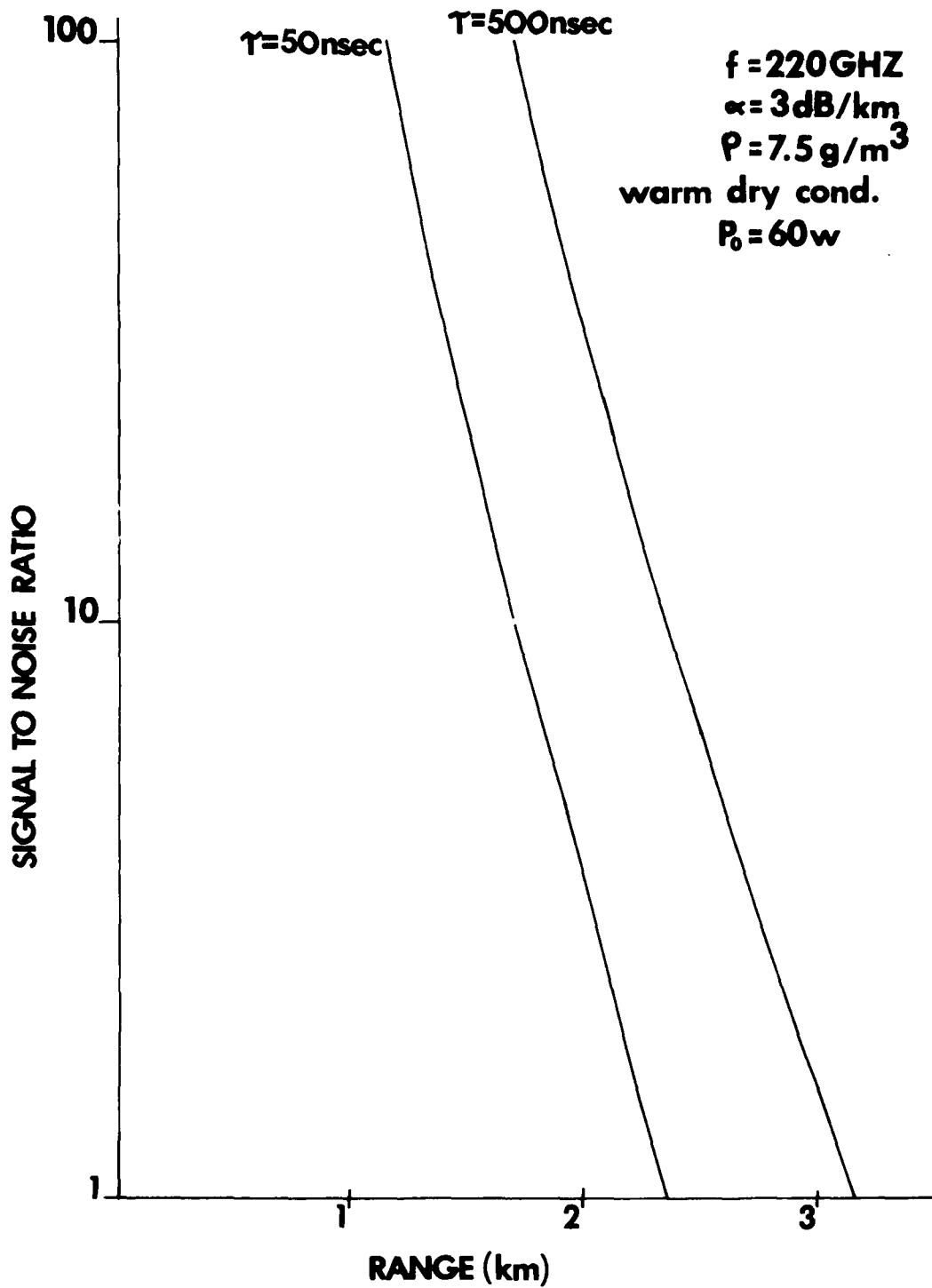
Figure 1-3. Calculated Range of 220 GHz Radar System Under Warm Dry Conditions.
