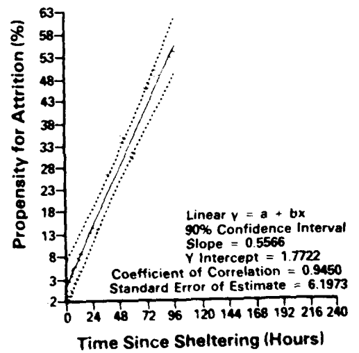
Figure 2-2. Graphs of the general attrition rate equations.
