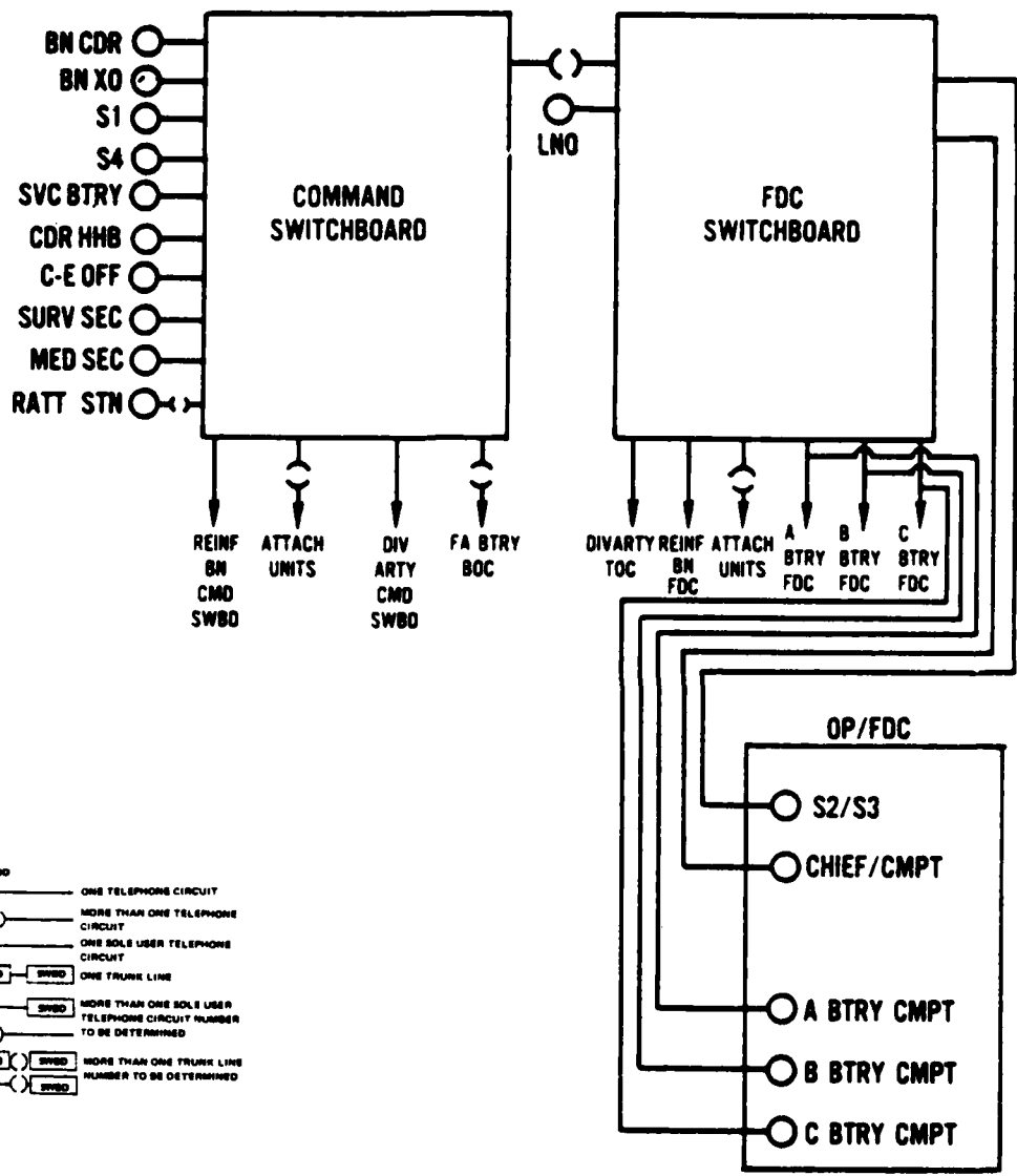
TELEPHONE AND CIRCUIT DISTRIBUTION DIAGRAM GENERAL SUPPORT BATTALION
