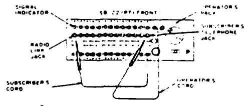
B SWITCHBOARD CONNECTIONS FOR SUBSCRIBER-RADIO LINE
