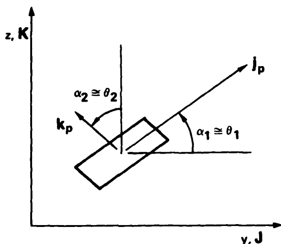
Figure 7.- Projection of the local cross-section principal axes on the y-z plane.
