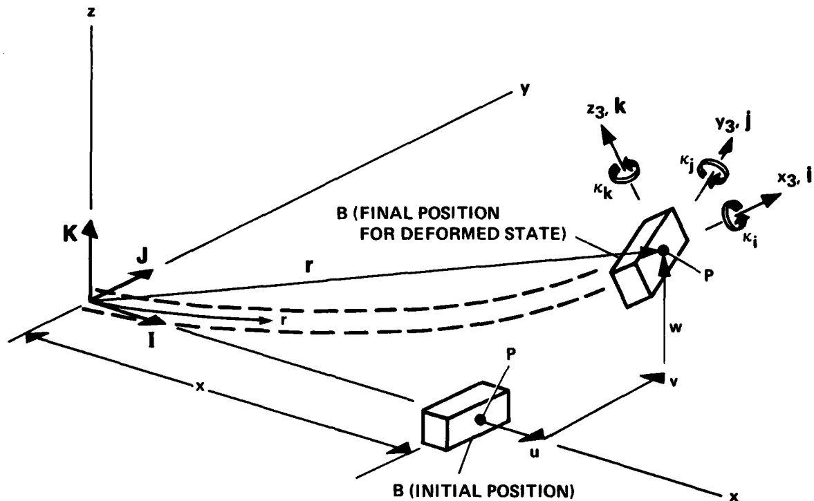
Figure 2.- Deformed-beam geometry.
