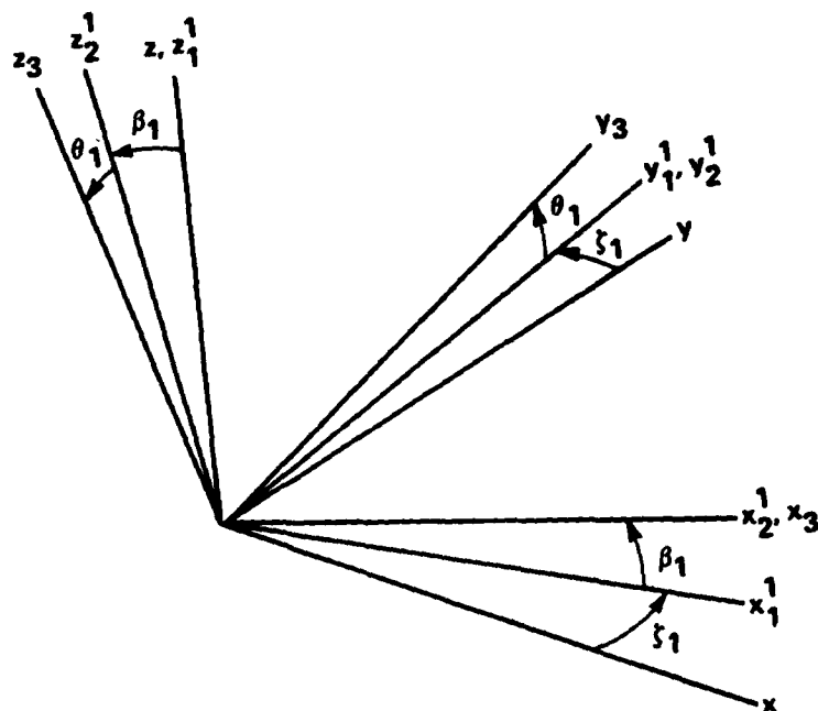
Figure 3.- The angles \xi_1 , \beta_1 , \theta_1 and respective axes of rotation.
