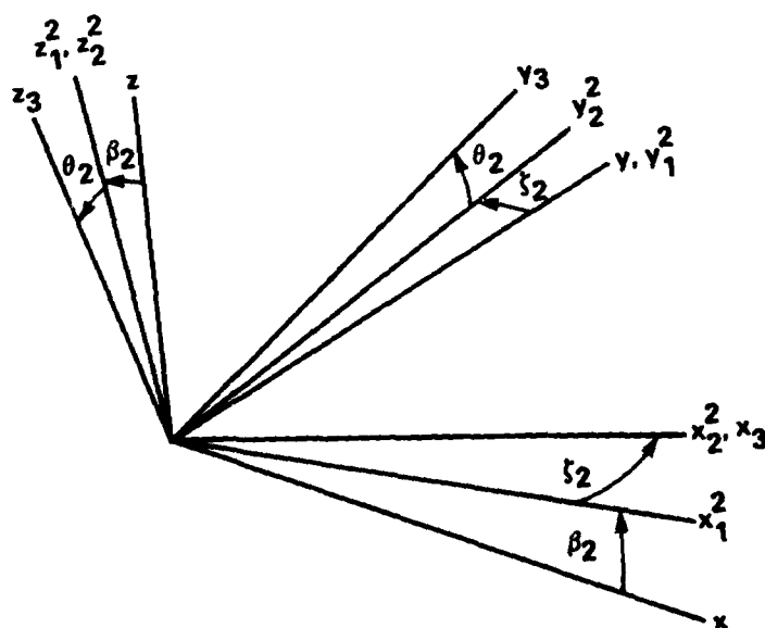
Figure 4.- The angles \beta_2 , \xi_2 , \theta_2 and respective axes of rotation.
