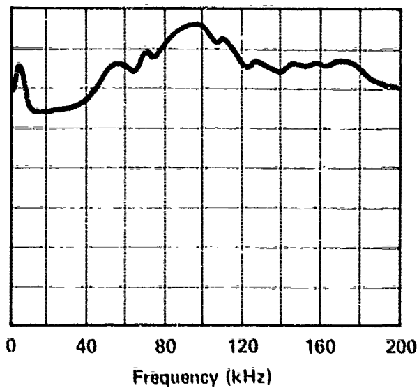
RELIEF VALVE - CIRCLE SEAL P10-776 INLET PRESSURE - 1500 PSI RETURN PRESSURE - 500 PSI FLOW TO VALVE - 9 GPM B-502
