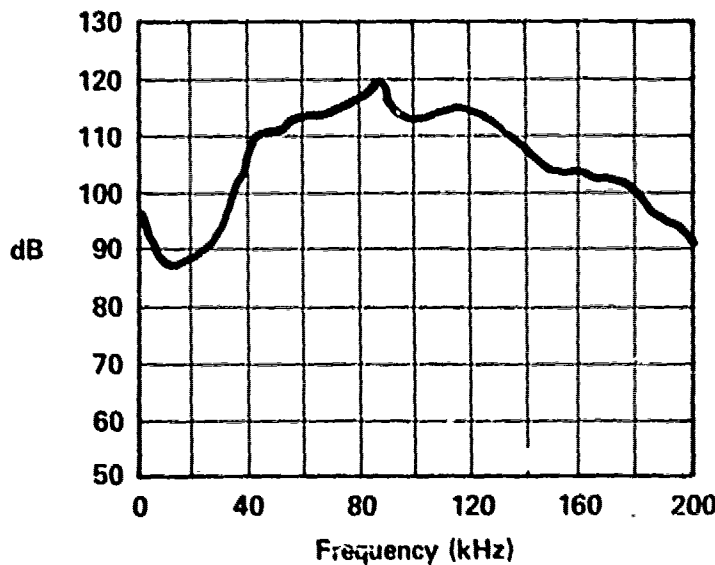
RELIEF VALVE - FLUID CONTROLS 1A-32 INLET PRESSURE - 1000 PSI RETURN PRESSURE - 0 PSI FLOW TO VALVE - 15 GPM B-103
