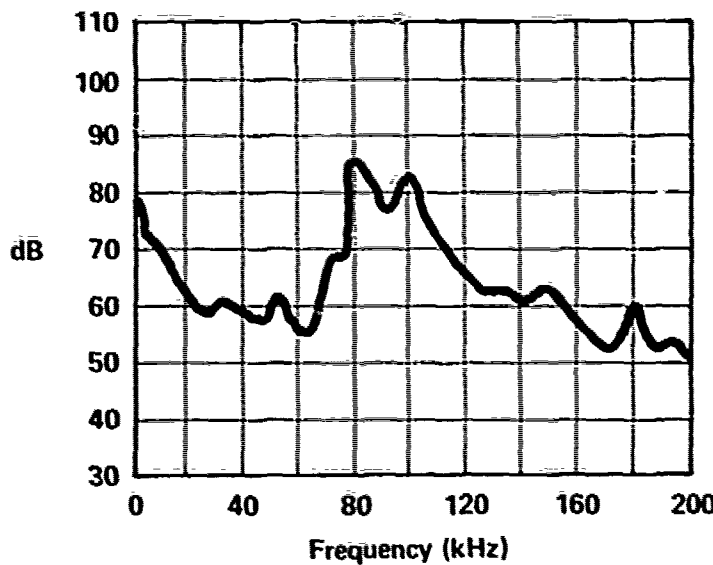
SERVO VALVE & MOTOR - MOOG 74 & WSI INLET PRESSURE - 1500 PSI C 1 PRESSURE - 1350 PSI C 2 PRESSURE - 700 PSI RETURN PRESSURE - 500 PSI FLOW TO VALVE/MOTOR - 4.6 GPM MOTOR RPM - 246 RPM DISK DIAMETER - 35.75 IN F-207
