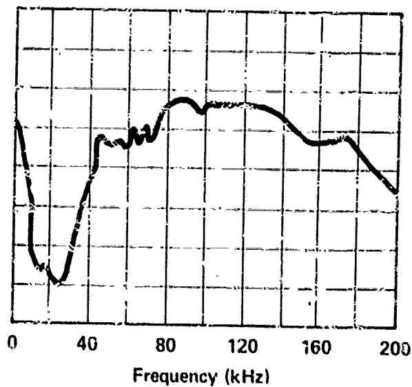
RELIEF VALVE - REPUBLIC RG70 INLET PRESSURE - 1000 PSI RETURN PRESSURE - 0 PSI FLOW TO VALVE - 10 GPM B-402
