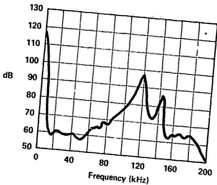
RELIEF VALVE - VICKERS INLET PRESSURE - 1000 PSI RETURN PRESSURE - 0 PSI FLOW TO VALVE - 5 GPM B-308
