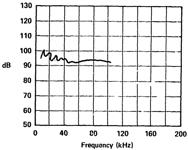
MOTOR - LAMINA MOTOR RPM - 300 RPM DISK DIAMETER - 22.625 IN TESTED AT KU TREE RESERVOIR C-201
