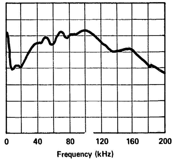
SERVO VALVE - MOOG 74 INLET PRESSURE - 1000 PSI C 1 /C 2 PRESSURE - 500 PSI RETURN PRESSURE - 0 PSI FLOW TO VALVE - 7.4 GPM E-104
