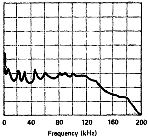
RELIEF VALVE - VICKERS INLET PRESSURE - 1450 PSI RETURN PRESSURE - 450 PSI FLOW TO VALVE - 20 GPM B-306
