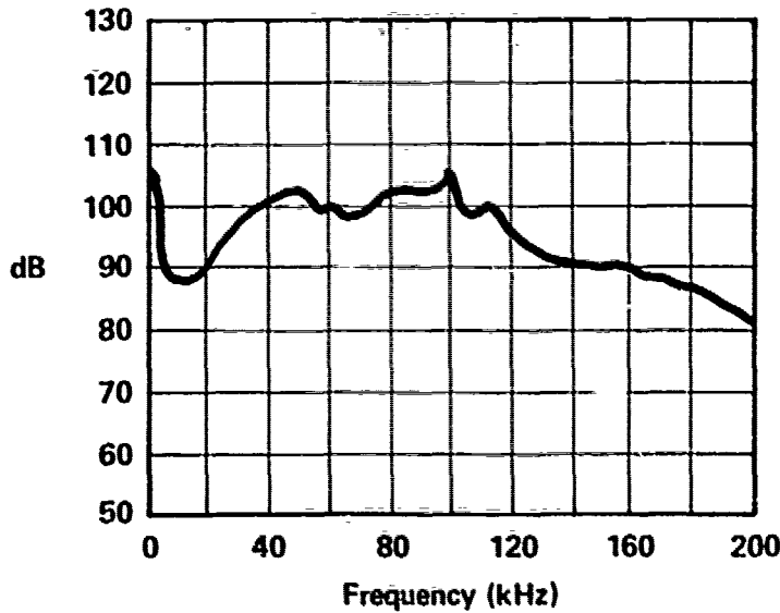
SERVO VALVE & MOTOR - OLSEN & NUTRON INLET PRESSURE - 1000 PSI C 1 PRESSURE - 900 PSI C 2 PRESSURE - 100 PSI RETURN PRESSURE - 0 PSI FLOW TO VALVE/MOTOR - 5.2 GPM MOTOR RPM - 450 RPM DISK DIAMETER - 24 IN F-103
