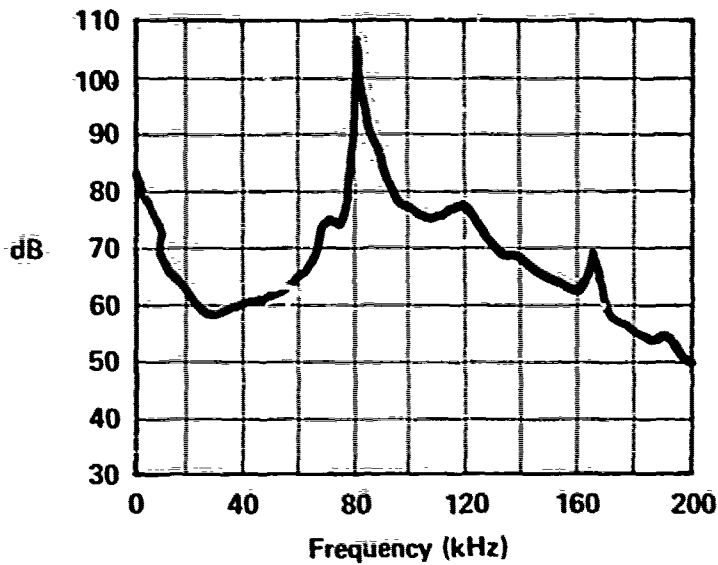
SERVO VALVE & MOTOR - MOOG 74 & WSI INLET PRESSURE - 1500 PSI C 1 PRESSURE - 1150 PSI C 2 PRESSURE - 800 PSI RETURN PRESSURE - 500 PSI FLOW TO VALVE/MOTOR - 3.2 GPM MOTOR RPM - 180 RPM DISK DIAMETER - 35.75 IN F-205
