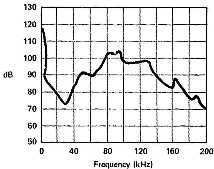
SERVO VALVE - MOOG 74 INLET PRESSURE - 1500 PSI C 1 /C 2 PRESSURE - 1000 PSI RETURN PRESSURE - 500 PSI FLOW TO VALVE - 3.2 GPM E-107
