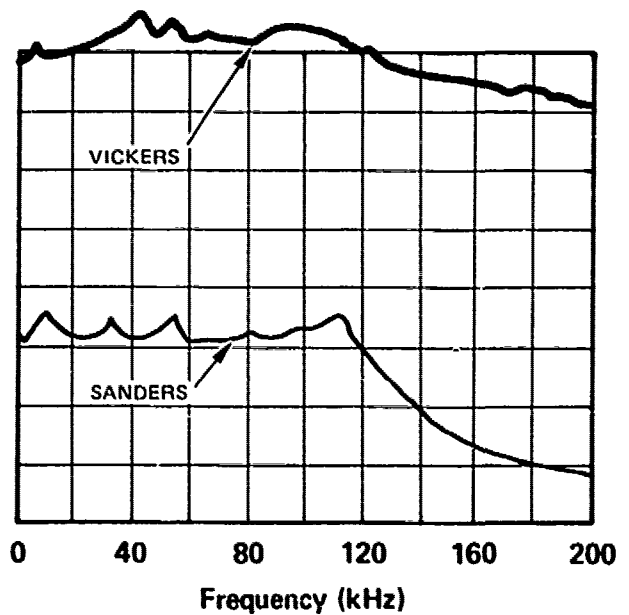
FLOW - 20 GPM G-108
