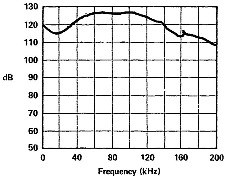
RELIEF VALVE - FLUID CONTROLS 1AR-41 INLET PRESSURE - 1000 PSI RETURN PRESSURE - 0 PSI FLOW TO VALVE - 15 GPM B-203
