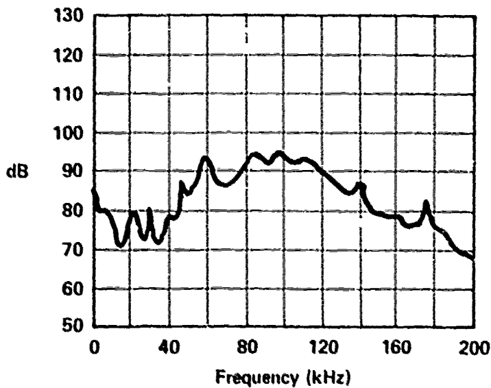
RELIEF VALVE - VICKERS INLET PRESSURE - 1300 PSI RETURN PRESSURE - 300 PSI FLOW TO VALVE - 20 GPM B-303
