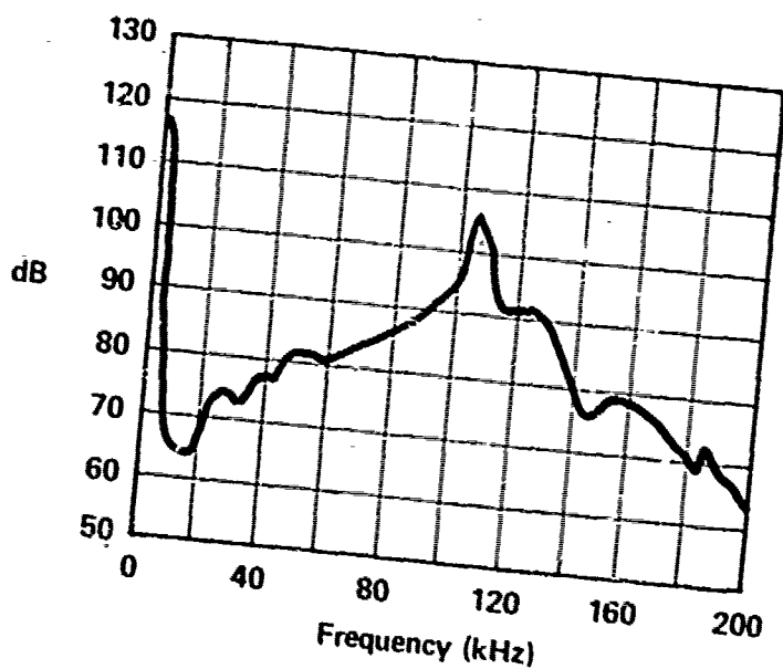
RELIEF VALVE - VICKERS INLET PRESSURE - 1000 PSI RETURN PRESSURE - 0 PSI FLOW TO VALVE - 15 GPM B-310
