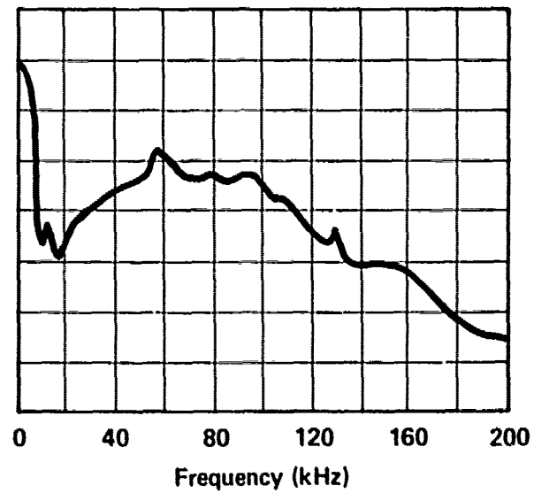
SERVO VALVE - MOOG 35 INLET PRESSURE - 1500 PSI C 1 /C 2 PRESSURE - 1000 PSI RETURN PRESSURE - 500 PSI FLOW TO VALVE - 4 GPM E-204
