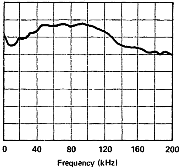
RELIEF VALVE - FLUID CONTROLS 1AR-41 INLET PRESSURE - 1000 PSI RETURN PRESSURE - 0 PSI FLOW TO VALVE - 10 GPM B-202
