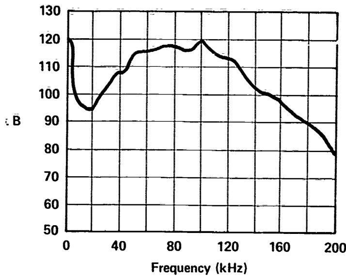
RELIEF VALVE - FLUID CONTROLS 1AR-41 INLET PRESSURE - 1500 PSI RETURN PRESSURE - 500 PSI FLOW TO VALVE - 5 GPM B-204
