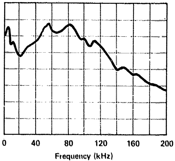
RELIEF VALVE - CIRCLE SEAL P10-776 INLET PRESSURE - 1500 PSI RETURN PRESSURE - 1000 PSI FLOW TO VALVE - 9 GPM B-504
