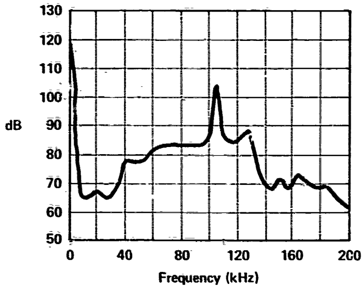
RELIEF VALVE - VICKERS INLET PRESSURE - 1500 PSI RETURN PRESSURE - 500 PSI FLOW TO VALVE - 15 GPM B-314
