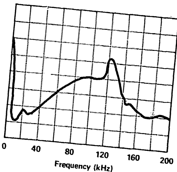
RELIEF VALVE - VICKERS INLET PRESSURE - 1000 PSI RETURN PRESSURE - 0 PSI FLOW TO VALVE - 10 GPM B-309
