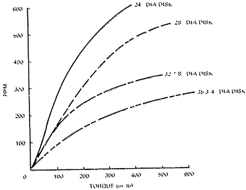
Figure 13. Disk data (rpm vs torque)
