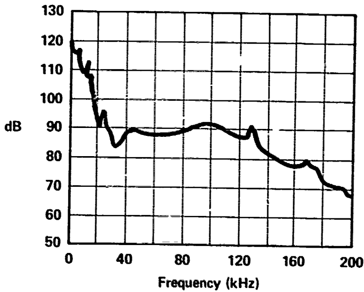
OUTPUT PRESSURE - 1000 PSI D-503
