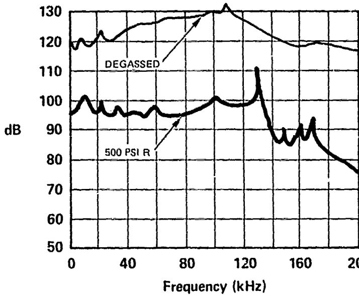
FLOW - 15 GPM B-338
