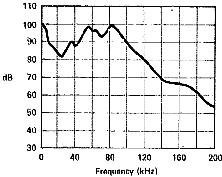
RELIEF VALVE - CIRCLE SEAL P10-776 INLET PRESSURE - 1000 PSI RETURN PRESSURE - 500 PSI FLOW TO VALVE - 9 GPM B-503
