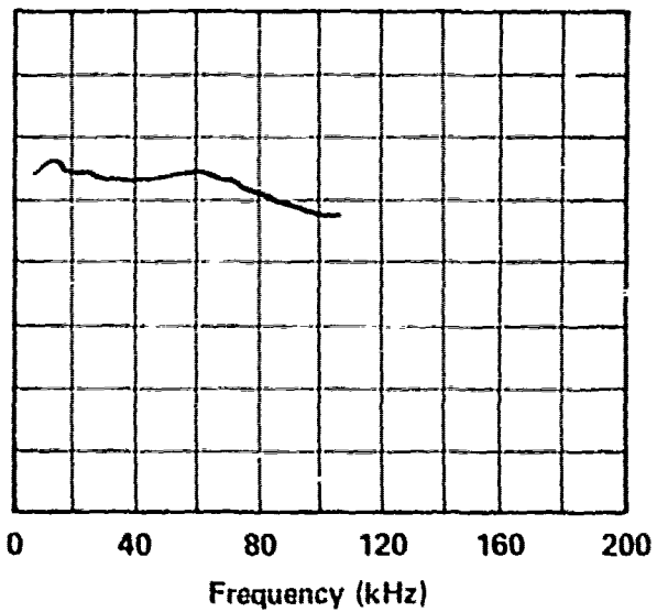
MOTOR - LAMINA MOTOR RPM - 450 RPM DISK DIAMETER - 22.625 IN TESTED AT KU TREE RESERVOIR C-202
