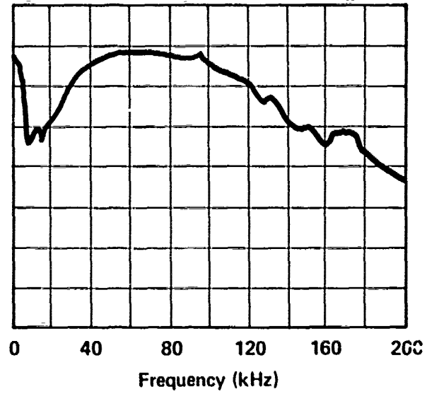
SERVO VALVE - MOOG 35 INLET PRESSURE - 1000 PSI C 1 /C 2 PRESSURE - 500 PSI RETURN PRESSURE - 0 PSI FLOW TO VALVE - 6 GPM E-202
