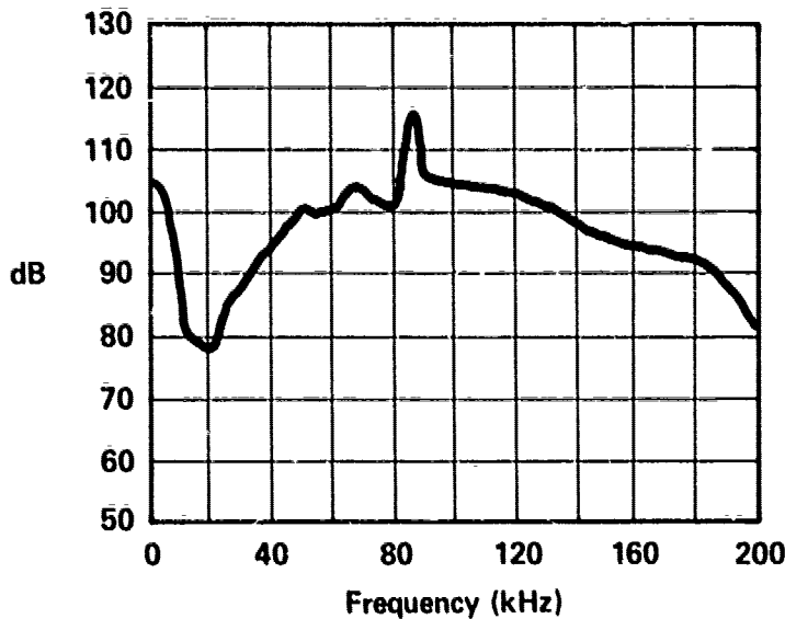
SERVO VALVE - MOOG 74 INLET PRESSURE - 1000 PSI C 1 /C 2 PRESSURE - 500 PSI RETURN PRESSURE - 0 PSI FLOW TO VALVE - 1.8 GPM E-101
