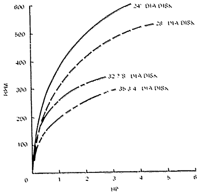
Figure 14. Disk data (rpm vs hp)
