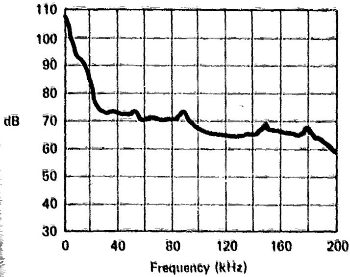
PUMP - RACINE SUPERVANE OUTPUT PRESSURE - 1000 PSI OUTPUT FLOW - 10 GPM DRIVE MOTOR - GE MOTOR @ 1750 RPM DRIVE COUPLING - DELRIN DIRECT DRIVE D-403
