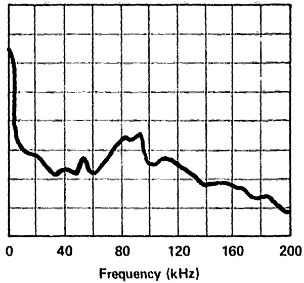
SERVO VALVE - MOOG 74 INLET PRESSURE - 1500 PSI C 1 /C 2 PRESSURE - 1000 PSI RETURN PRESSURE - 500 PSI FLOW TO VALVE - 0 GPM E-106
