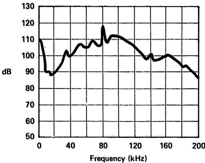
SERVO VALVE - MOOG 74 INLET PRESSURE - 1000 PSI C 1 /C 2 PRESSURE - 500 PSI RETURN PRESSURE - 0 PSI FLOW TO VALVE - 7.2 GPM E-103
