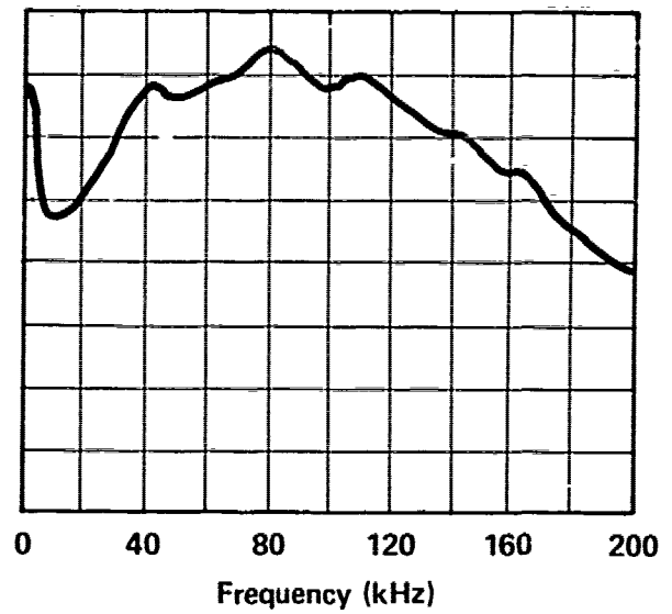
RELIEF VALVE - FLUID CONTROLS 1AR-41 INLET PRESSURE - 1500 PSI RETURN PRESSURE - 500 PSI FLOW TO VALVE - 10 GPM B-205
