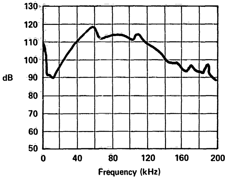
SERVO VALVE - MOOG 35 INLET PRESSURE - 1000 PSI C 1 /C 2 PRESSURE - 500 PSI RETURN PRESSURE - 0 PSI FLOW TO VALVE - 4 GPM E-201
