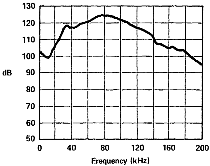
RELIEF VALVE - FLUID CONTROLS 1AR-41 INLET PRESSURE - 1000 PSI RETURN PRESSURE - 0 PSI FLOW TO VALVE - 5 GPM B-201
