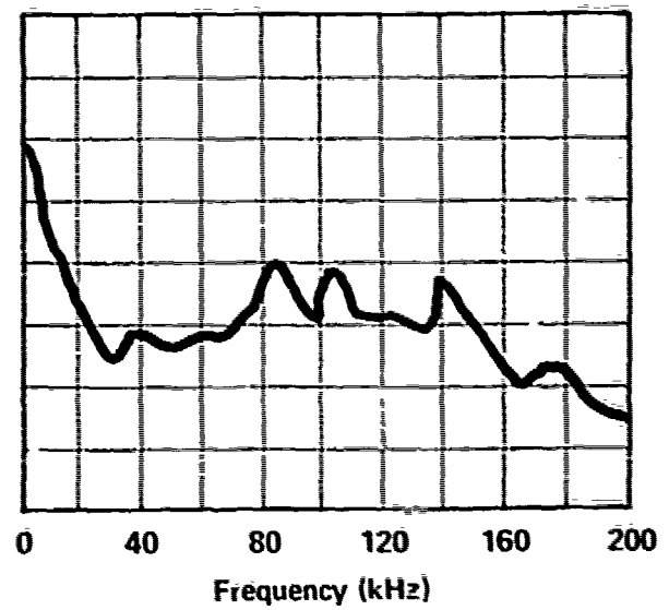
SERVO VALVE & MOTOR - MOOG 74 & WSI INLET PRESSURE - 1500 PSI C 1 PRESSURE - 1450 PSI C 2 PRESSURE - 700 PSI RETURN PRESSURE - 500 PSI FLOW TO VALVE/MOTOR - 5.1 GPM MOTOR RPM - 270 RPM DISK DIAMETER - 35.75 IN F-208
