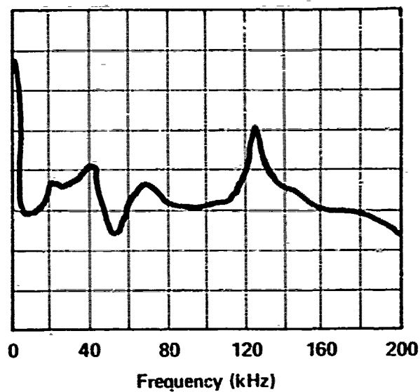
RELIEF VALVE - VICKERS INLET PRESSURE - 1500 PSI RETURN PRESSURE - 500 PSI FLOW TO VALVE - 10 GPM B-313
