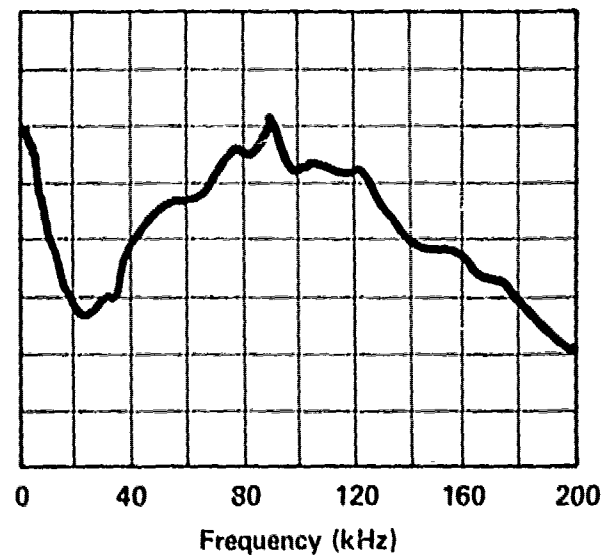
SERVO VALVE - MOOG 74 INLET PRESSURE - 1500 PSI C 1 /C 2 PRESSURE - 1000 PSI RETURN PRESSURE - 500 PSI FLOW TO VALVE - 5.7 GPM E-108
