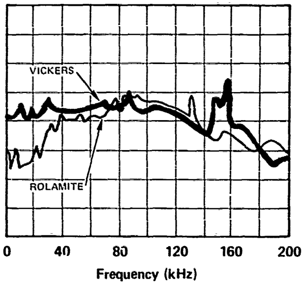
FLOW - 10 GPM G-206
