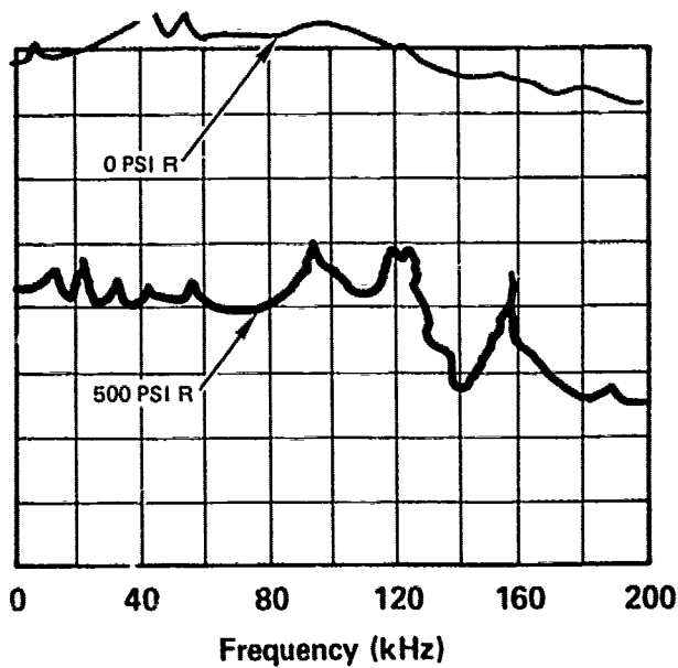
FLOW - 20 GPM B-335
