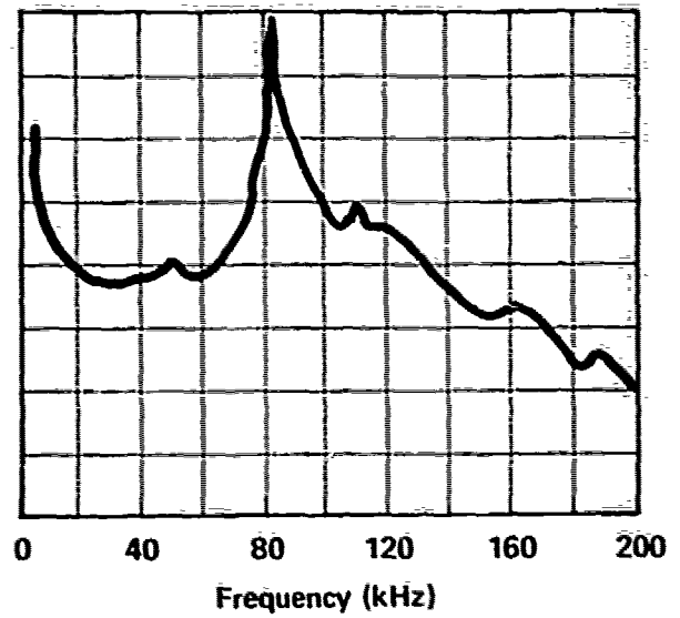
SERVO VALVE & MOTOR - MOOG 74 & WSI INLET PRESSURE - 1500 PSI C 1 PRESSURE - 1200 PSI C 2 PRESSURE - 750 PSI RETURN PRESSURE - 500 PSI FLOW TO VALVE/MOTOR - 3.6 GPM MOTOR RPM - 210 RPM DISK DIAMETER - 35.75 IN F-206
