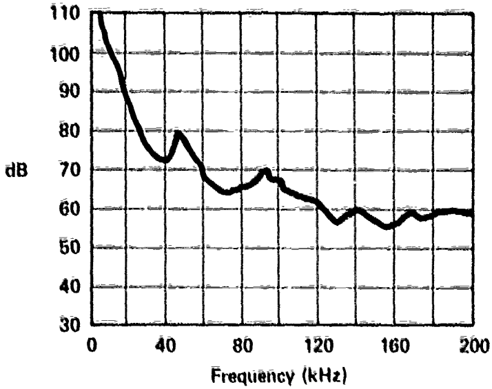
PUMP - RACINE SUPERVANE OUTPUT PRESSURE - 1000 PSI OUTPUT FLOW - 0 GPM DRIVE MOTOR - GE MOTOR @ 1750 RPM DRIVE COUPLING - DELRIN DIRECT DRIVE D-401
