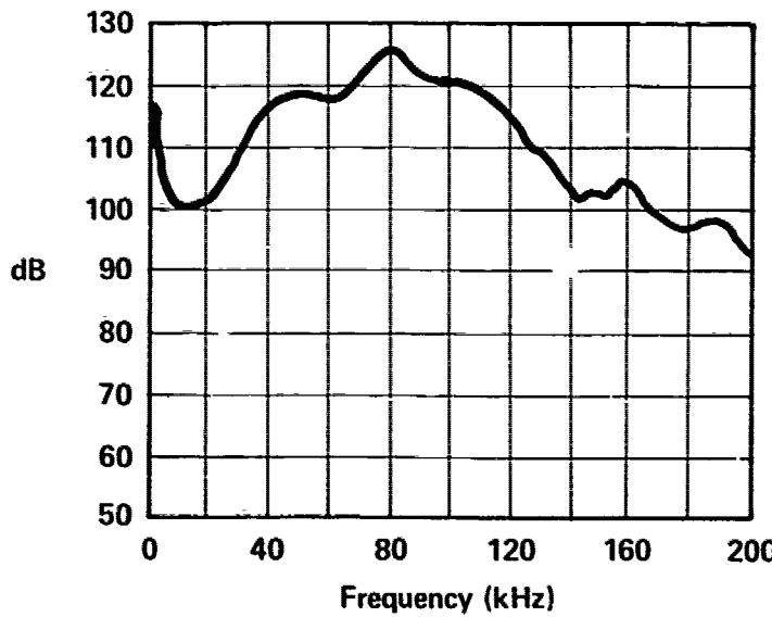
RELIEF VALVE - FLUID CONTROLS 1AR-41 INLET PRESSURE - 1500 PSI RETURN PRESSURE - 500 PSI FLOW TO VALVE - 15 GPM B-206
