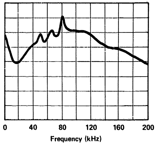
SERVO VALVE - MOOG 74 INLET PRESSURE - 1000 PSI C 1 /C 2 PRESSURE - 500 PSI RETURN PRESSURE - 0 PSI FLOW TO VALVE - 4.7 GPM E-102
