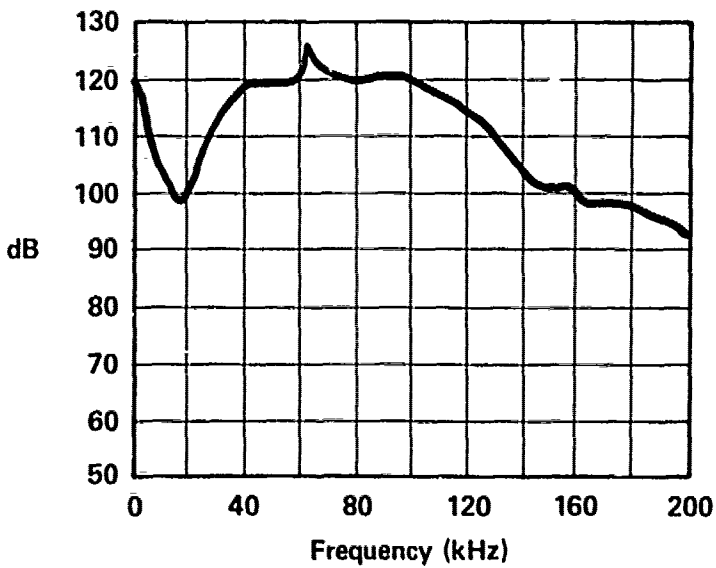
SERVO VALVE - MOOG 35 INLET PRESSURE - 1000 PSI C 1 /C 2 PRESSURE - 500 PSI RETURN PRESSURE - 0 PSI FLOW TO VALVE - 8 GPM E-203
