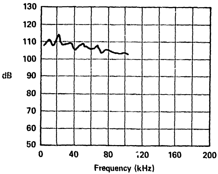
MOTOR - LAMINA MOTOR RPM - 600 RPM DISK DIAMETER - 22.625 IN TESTED AT KU TREE RESERVOIR C-203
