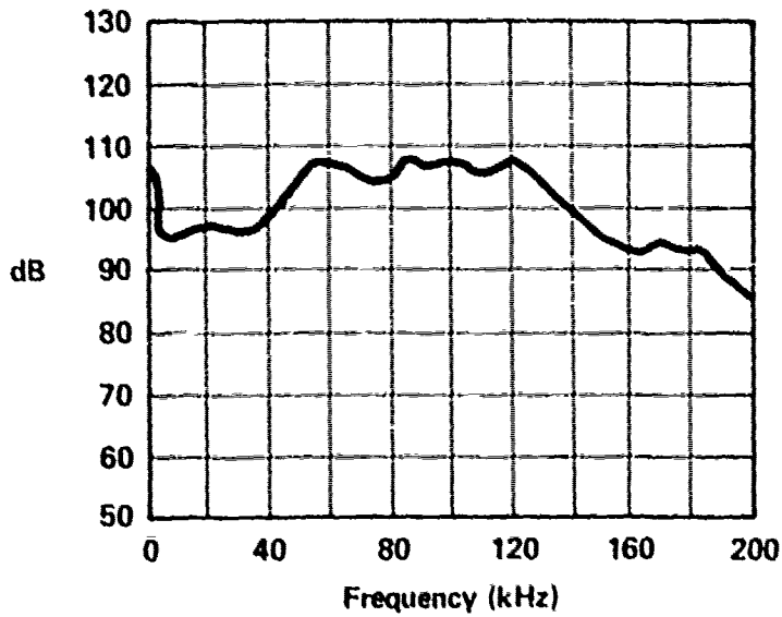
RELIEF VALVE - VICKERS INLET PRESSURE - 1000 PSI RETURN PRESSURE - 0 PSI FLOW TO VALVE - 20 GPM B-301
