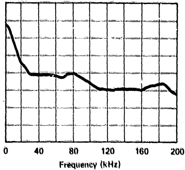
PUMP - RACINE SUPERVANE OUTPUT PRESSURE - 1000 PSI OUTPUT FLOW - 5 GPM DRIVE MOTOR - GE MOTOR @ 1750 RPM DRIVE COUPLING - DELRIN DIRECT DRIVE D-402
