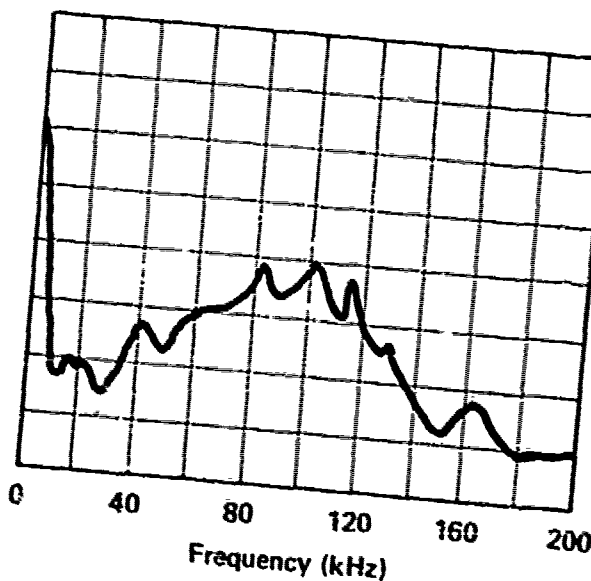
RELIEF VALVE - VICKERS INLET PRESSURE - 1000 PSI RETURN PRESSURE - 0 PSI FLOW TO VALVE - 20 GPM B-311
