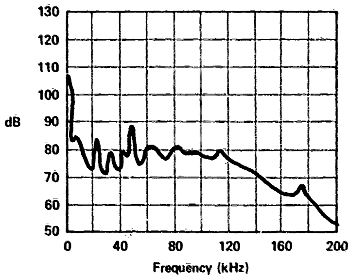
RELIEF VALVE - VICKERS INLET PRESSURE - 1500 PSI RETURN PRESSURE - 500 PSI FLOW TO VALVE - 20 GPM B-307
