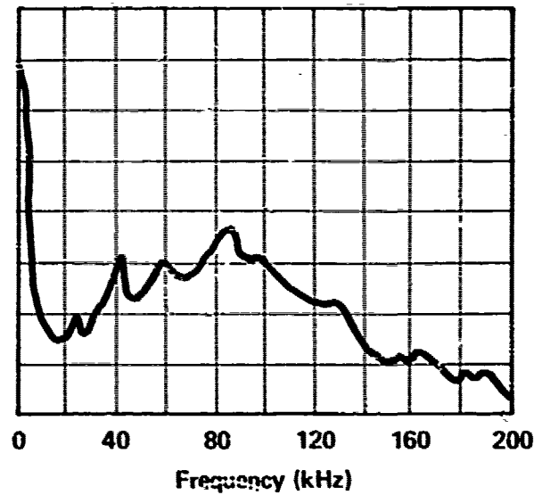
RELIEF VALVE - VICKERS INLET PRESSURE - 1500 PSI RETURN PRESSURE - 500 PSI FLOW TO VALVE - 20 GPM B-315
