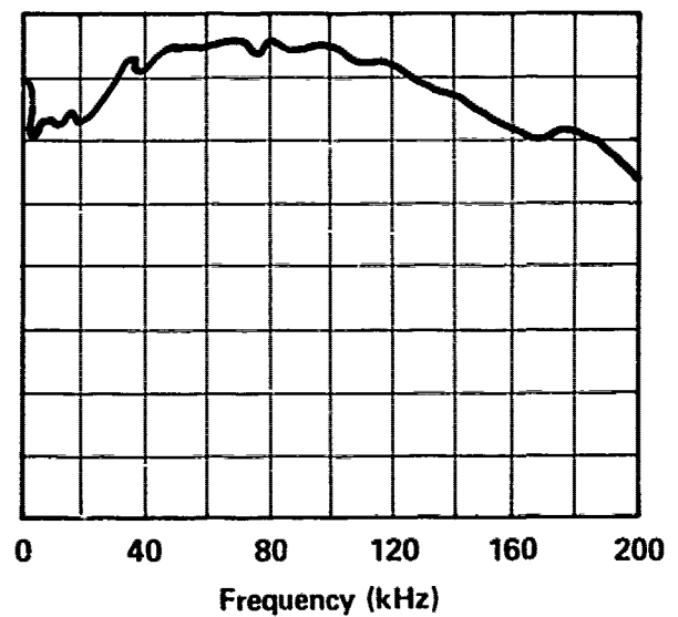
RELIEF VALVE - FLUID CONTROLS 1AR-41 INLET PRESSURE - 1500 PSI RETURN PRESSURE - 500 PSI FLOW TO VALVE - 20 GPM B-207
