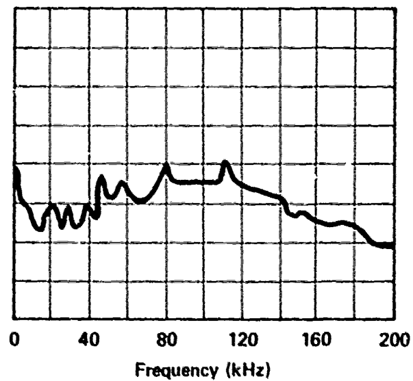
RELIEF VALVE - VICKERS INLET PRESSURE - 1350 PSI RETURN PRESSURE - 350 PSI FLOW TO VALVE - 20 GPM B-304
