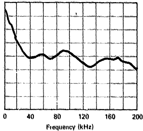
PUMP - RACINE SUPERVANE OUTPUT PRESSURE - 1000 PSI OUTPUT FLOW - 13 GPM DRIVE MOTOR - GE MOTOR @ 1750 RPM DRIVE COUPLING - DELRIN DIRECT DRIVE D-404
