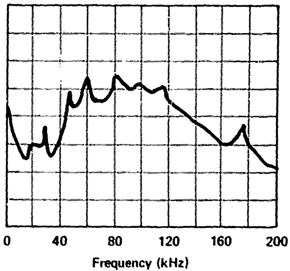
RELIEF VALVE - VICKERS INLET PRESSURE - 1250 PSI RETURN PRESSURE - 250 PSI FLOW TO VALVE - 20 GPM B-302
