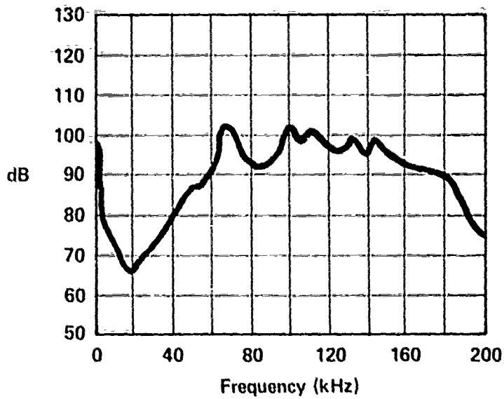
SERVO VALVE - MOOG 74 INLET PRESSURE - 1250 PSI C 1 /C 2 PRESSURE - 750 PSI RETURN PRESSURE - 250 PSI FLOW TO VALVE - 4 GPM E-105
