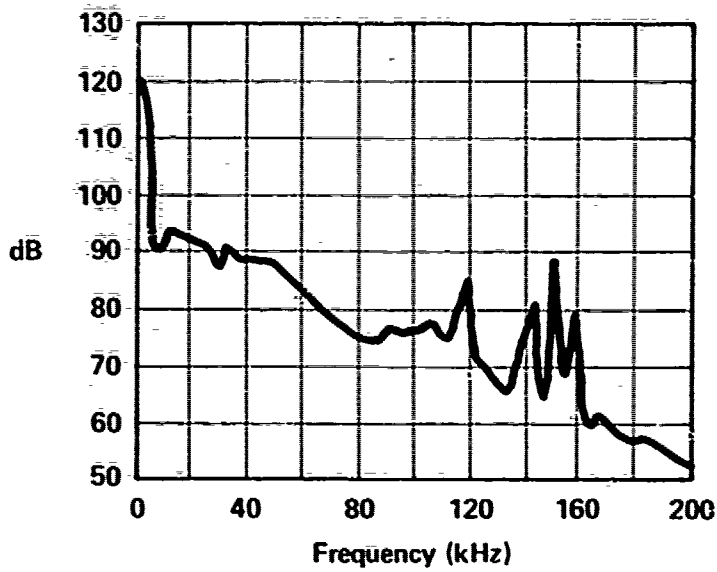
RELIEF VALVE - VICKERS INLET PRESSURE - 1500 PSI RETURN PRESSURE - 500 PSI FLOW TO VALVE - 5 GPM B-312
