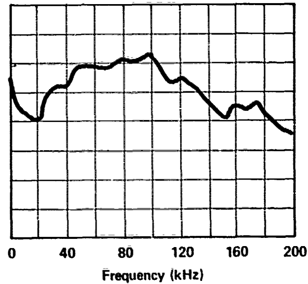
SERVO VALVE & MOTOR - OLSEN & NUTRON INLET PRESSURE - 1450 PSI C 1 PRESSURE - 1350 PSI C 2 PRESSURE - 100 PSI RETURN PRESSURE - 0 PSI FLOW TO VALVE/MOTOR - 7.4 GPM MOTOR RPM - 600 RPM DISK DIAMETER - 24 IN F-104
