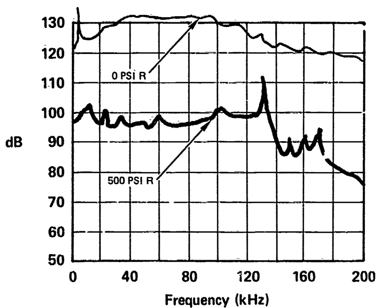
FLOW - 15 GPM B-334
