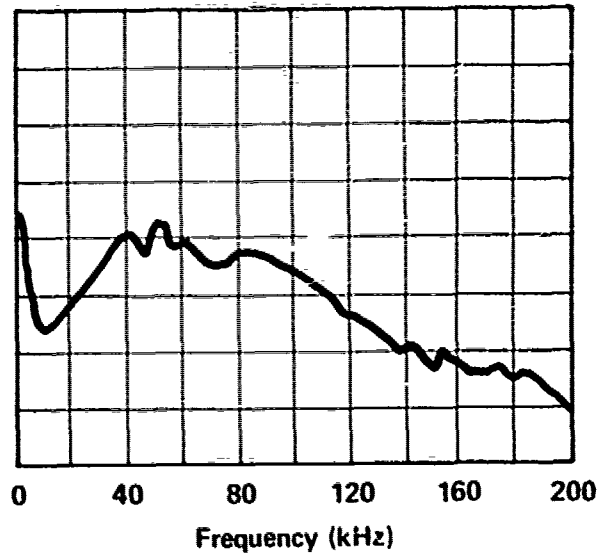
SERVO VALVE & MOTOR - OLSEN & NUTRON INLET PRESSURE - 1000 PSI C 1 PRESSURE - 700 PSI C 2 PRESSURE - 300 PSI RETURN PRESSURE - 0 PSI FLOW TO VALVE/MOTOR - 3.8 GPM MOTOR RPM - 300 RPM DISK DIAMETER - 24 IN F-102
