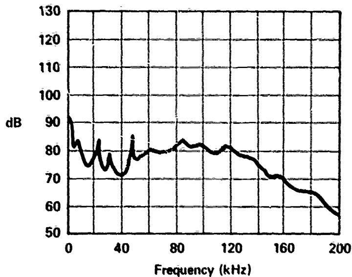
RELIEF VALVE - VICKERS INLET PRESSURE - 1400 PSI RETURN PRESSURE - 400 PSI FLOW TO VALVE - 20 GPM B-305
