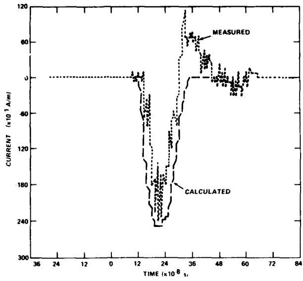
Figure 29. Calculated and measured termination currents, transmission line, configuration II (capacitor 0 V).
