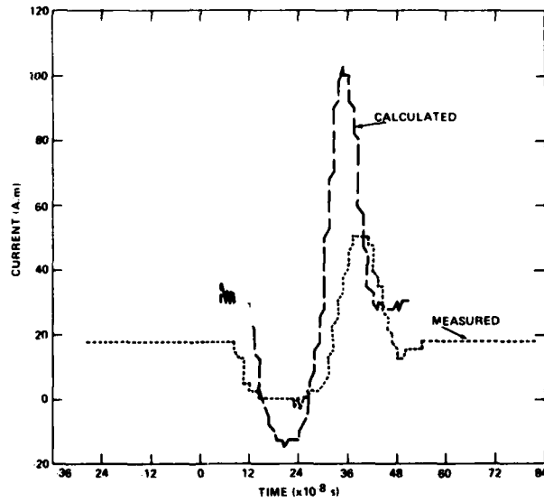
Figure 30. Calculated and measured termination currents, transmission line, configuration III.
