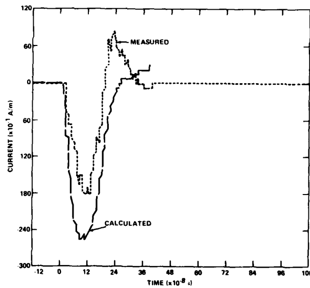
Figure 27. Calculated and measured termination currents, transmission line, configuration I (capacitor 0 V).
