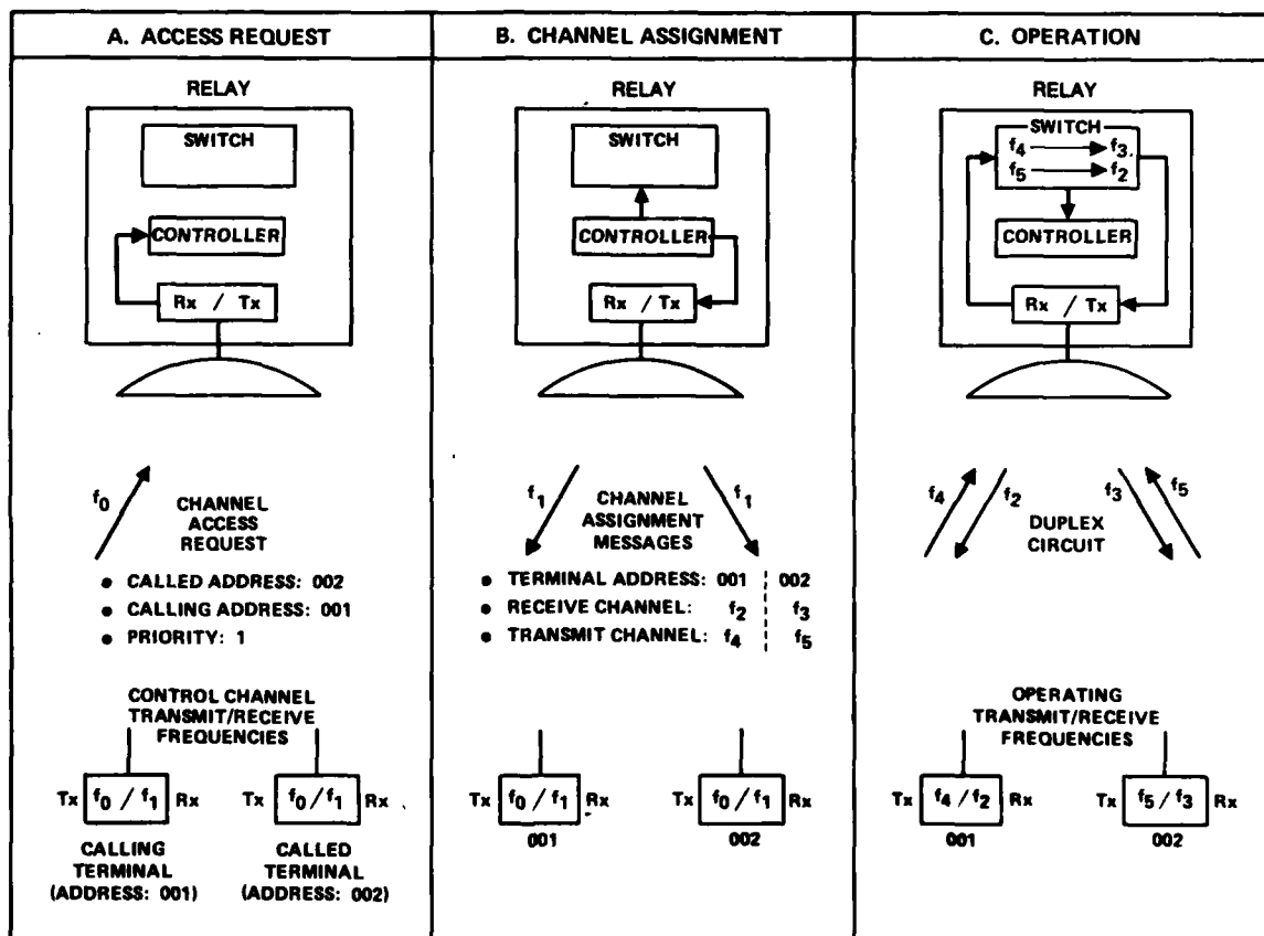
FIGURE 4.1. BASIC STEPS OF SYSTEM OPERATION
