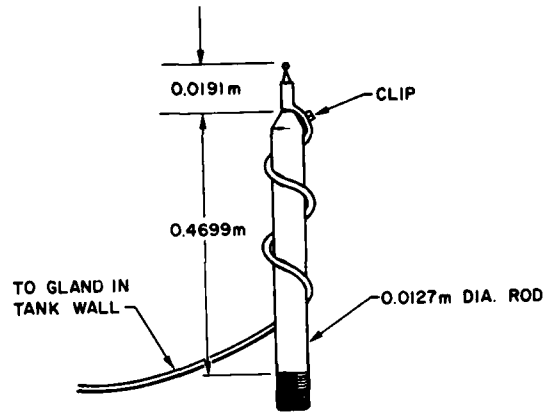
Fig. 3 - Thermocouple fixture
