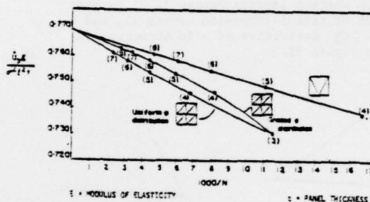
FIGURE 7: CENTRALLY CRACKED PANEL COMPUTED (NORMALIZED) STRAIN ENERGY FOR DIFFERENT p vs. (1000/N)
