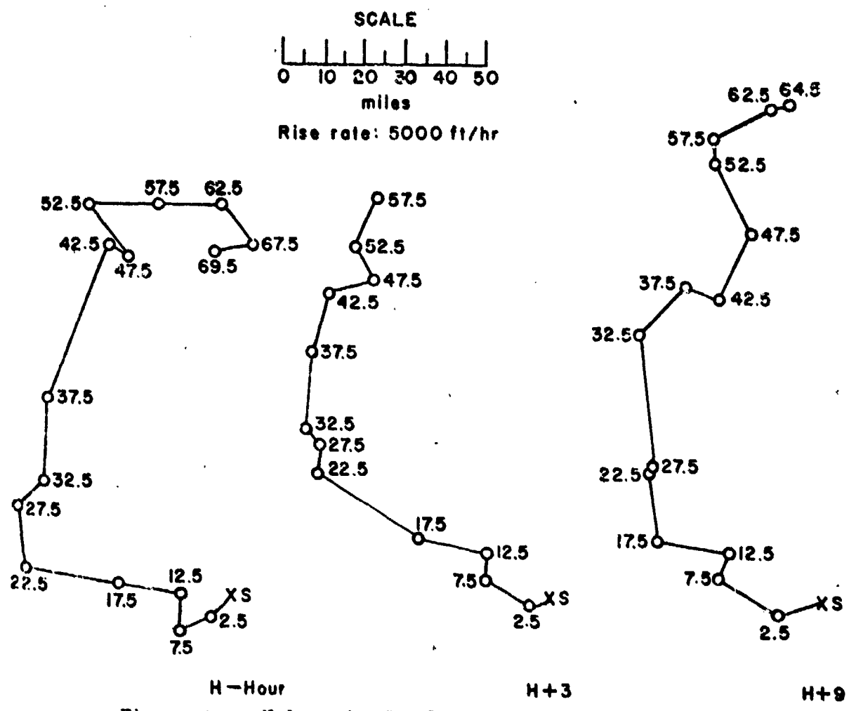
Figure 47. Hodographs for Operation CASTLE -
