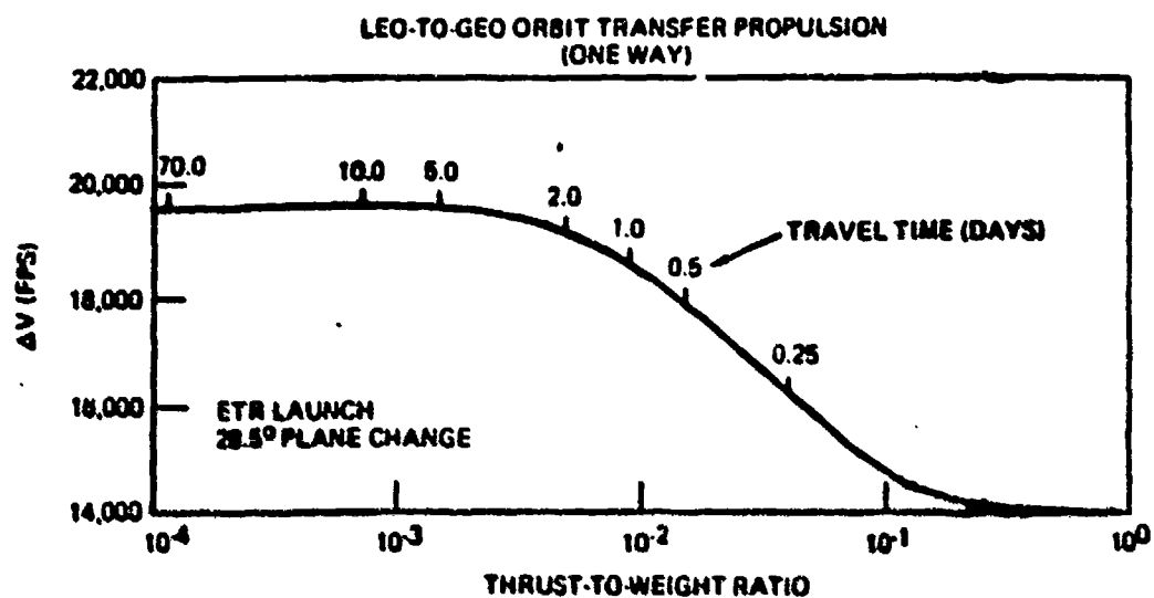
Figure 4. Delta-V Requirements Versus Thrust to Weight
