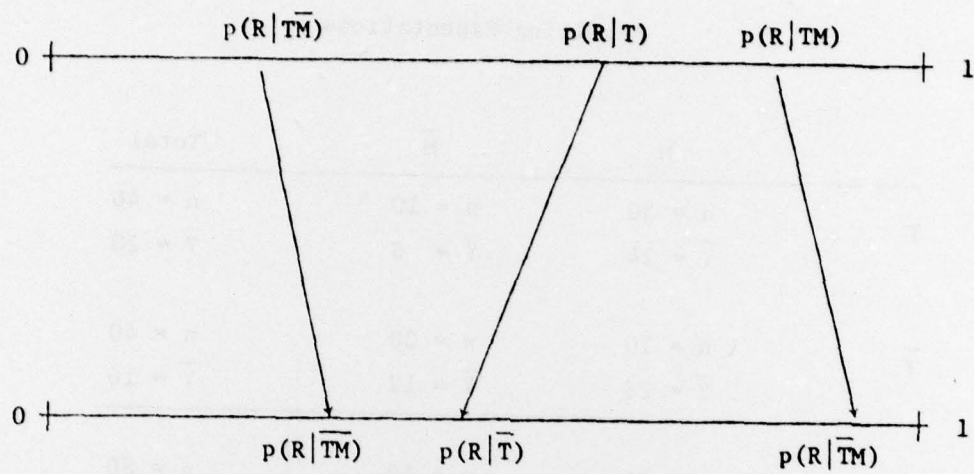
Figure: Simpson's Paradox
