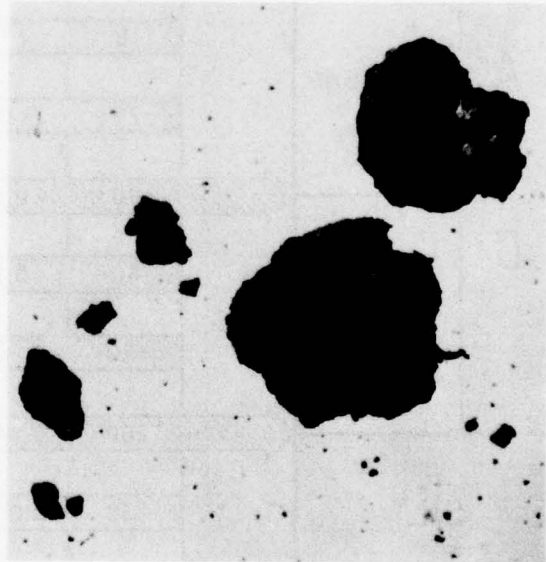
d. Large, irregular glauconite grains.
