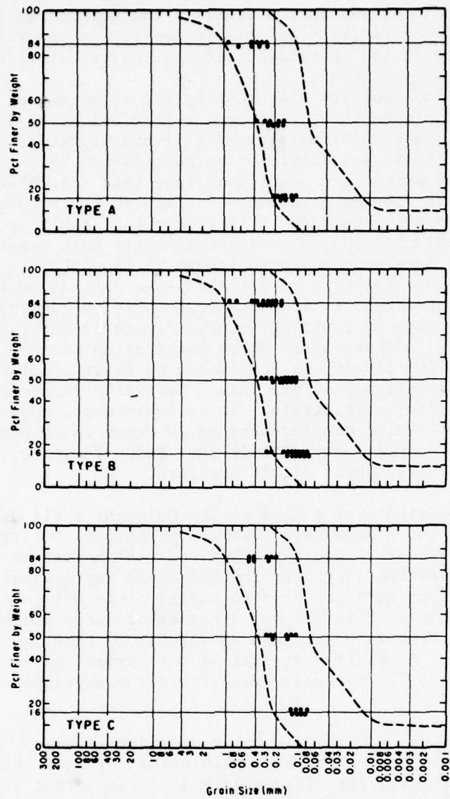
Figure 29. Comparison of fine sand from the study area with sands known to have liquefied under cyclic loading.
