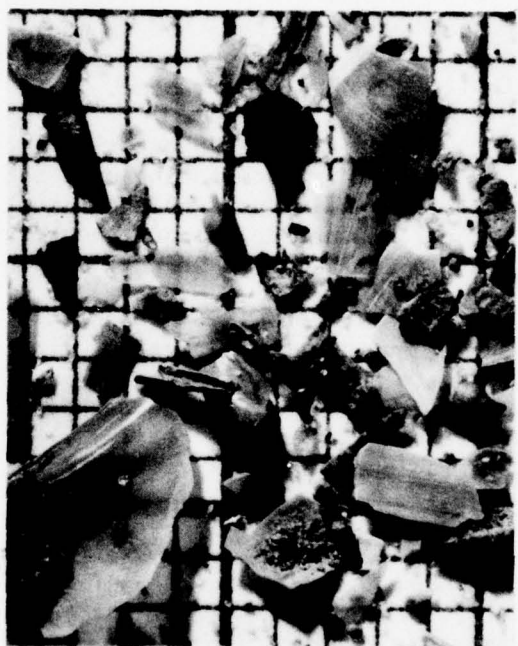
Figure 20. Typical examples of type E, shelly sand and shell hash (grid interval, 1 millimeter).
