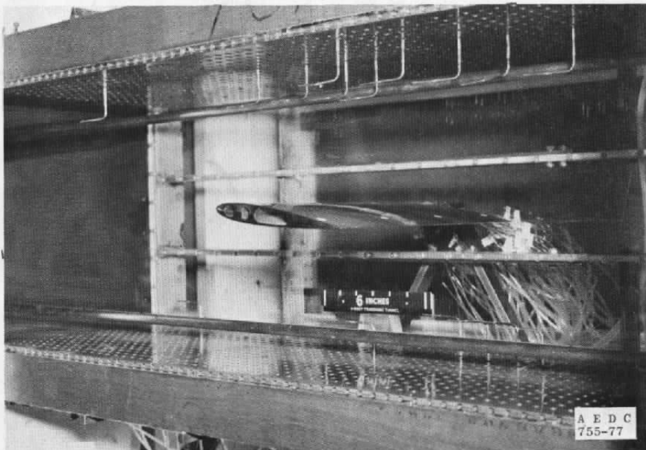
Figure 8. Adaptive-wall test section configuration.
