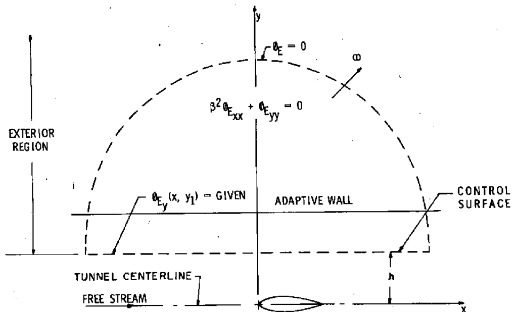
Figure 9. Boundary-value problem of exterior unconfined region.
