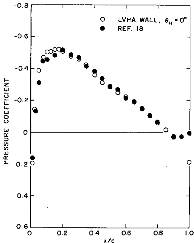
Figure 11. Model surface pressure distribution, M_\infty = 0.65 and \alpha = 0 deg.
