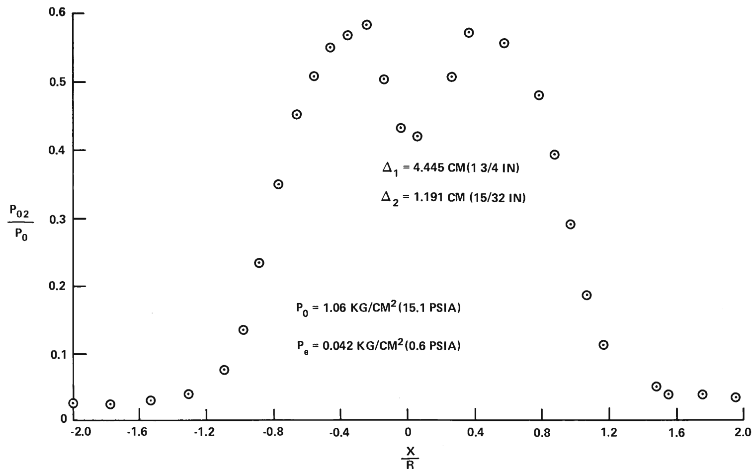
FIGURE 39a. PITOT SURVEY — PITOT-PLATE CONFIGURATION NOZZLE NO. 2 (RUN NO. 42)
