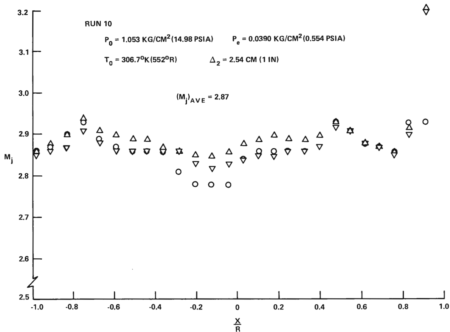
FIGURE 28 FREE JET MACH NO. - NOZZLE NO. 2 (PITOT SURVEY)
