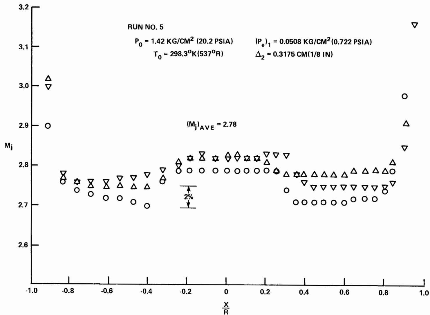
FIGURE 25 FREE JET MACH NO. — NOZZLE NO. 2 (PITOT SURVEY)
