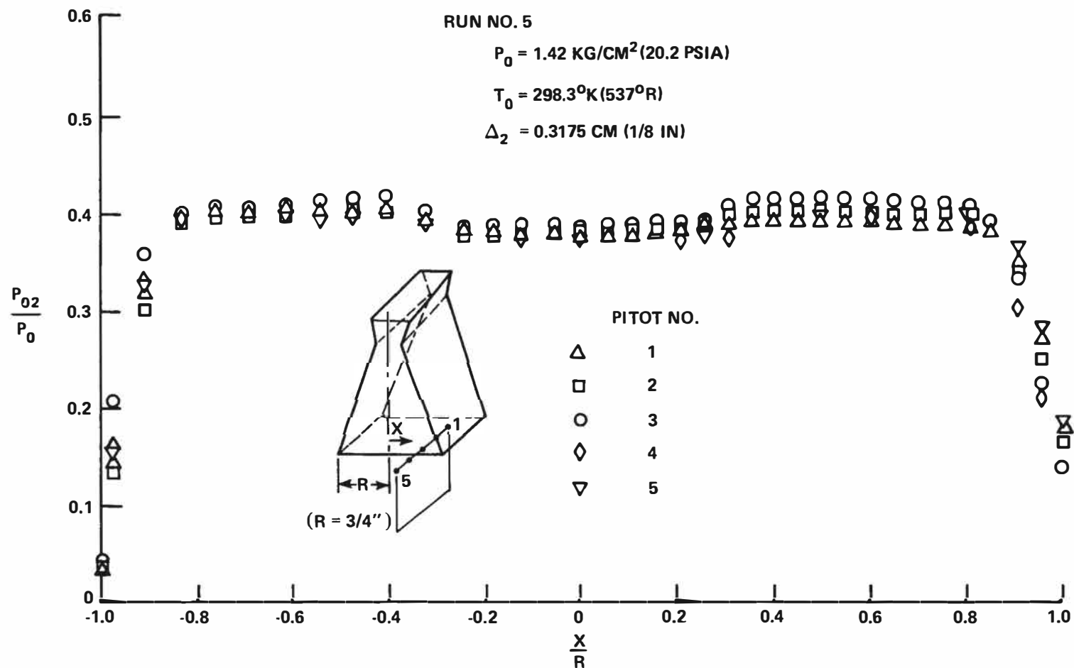
FIGURE 23 PITOT SURVEY - NOZZLE NO. 2
