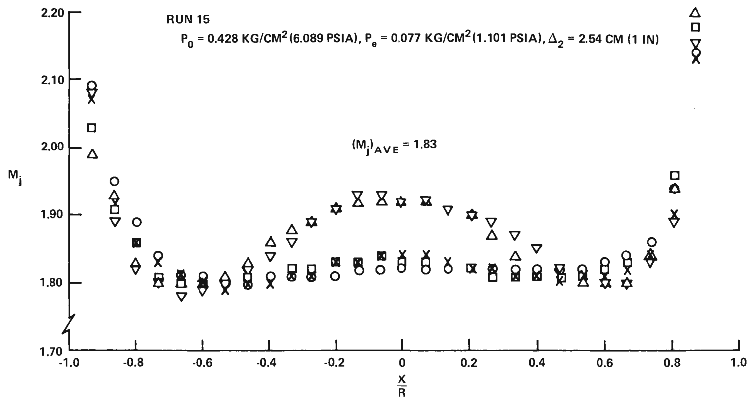
FIGURE 9 FREE JET MACH NO. - NOZZLE NO. 1 (PITOT SURVEY)
