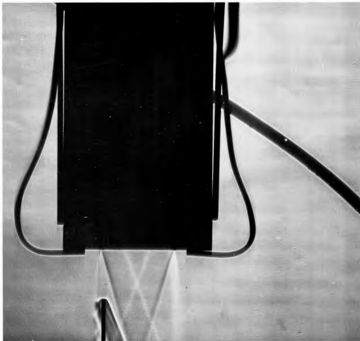
FIGURE 32 SCHLIEREN PHOTOGRAPH OF PITOT SURVEY: NOZZLE NO. 2 (RUN 10)
