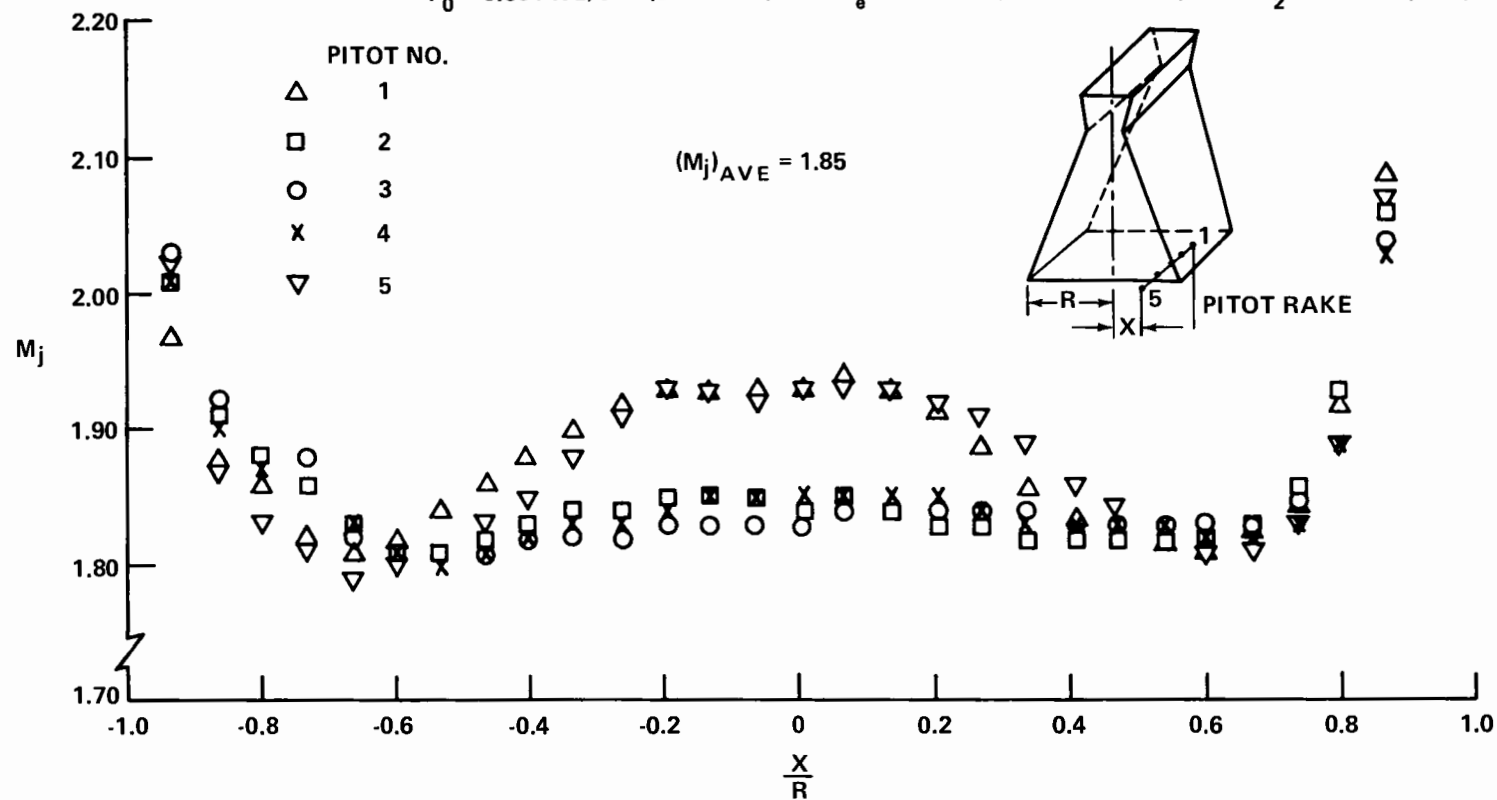
FIGURE 11 FREE JET MACH NO. — NOZZLE NO. 1 (PITOT SURVEY)
