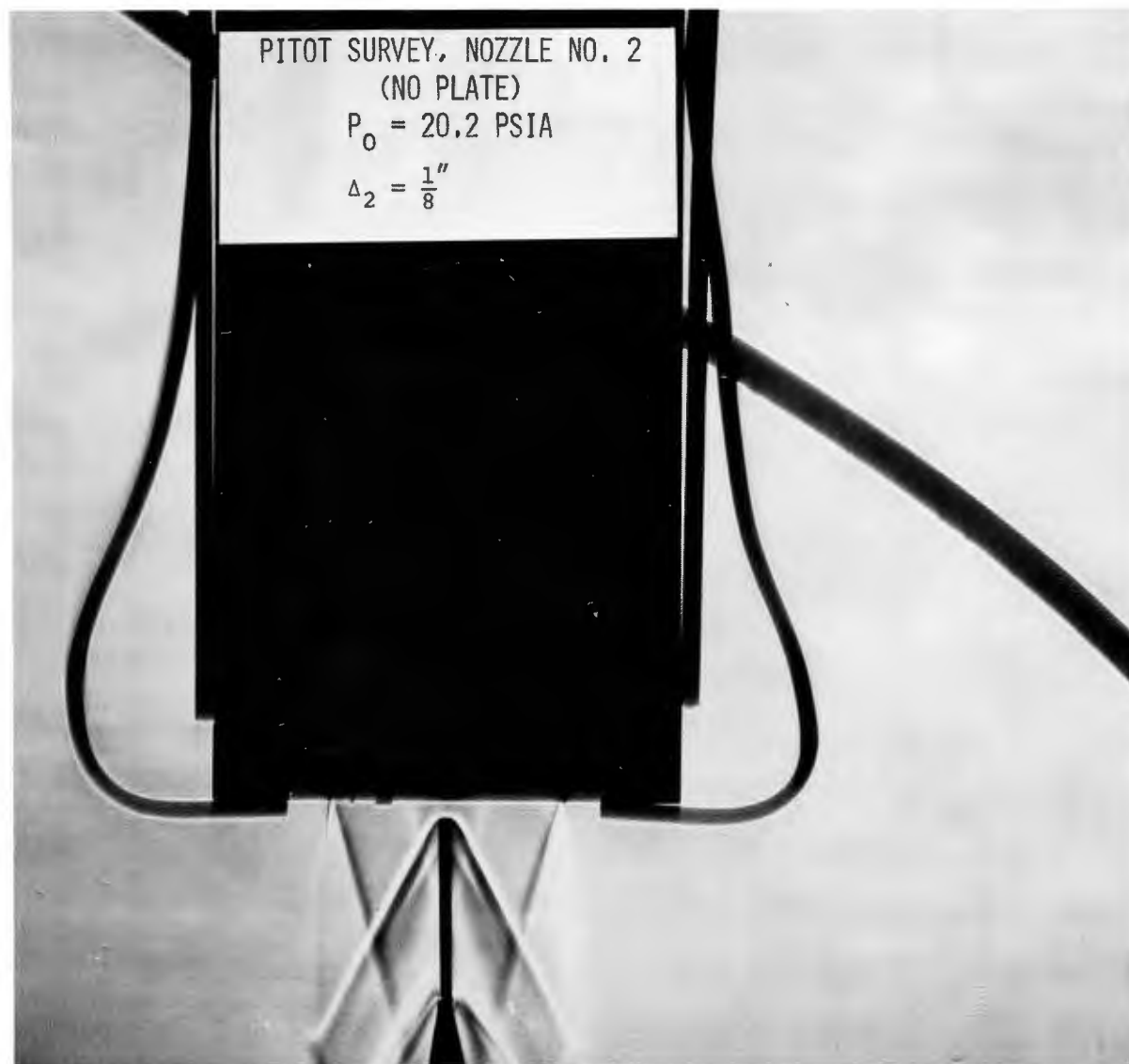
FIGURE 29 SCHLIEREN PHOTOGRAPH OF PITOT SURVEY: NOZZLE NO. 2 (RUN 5)
