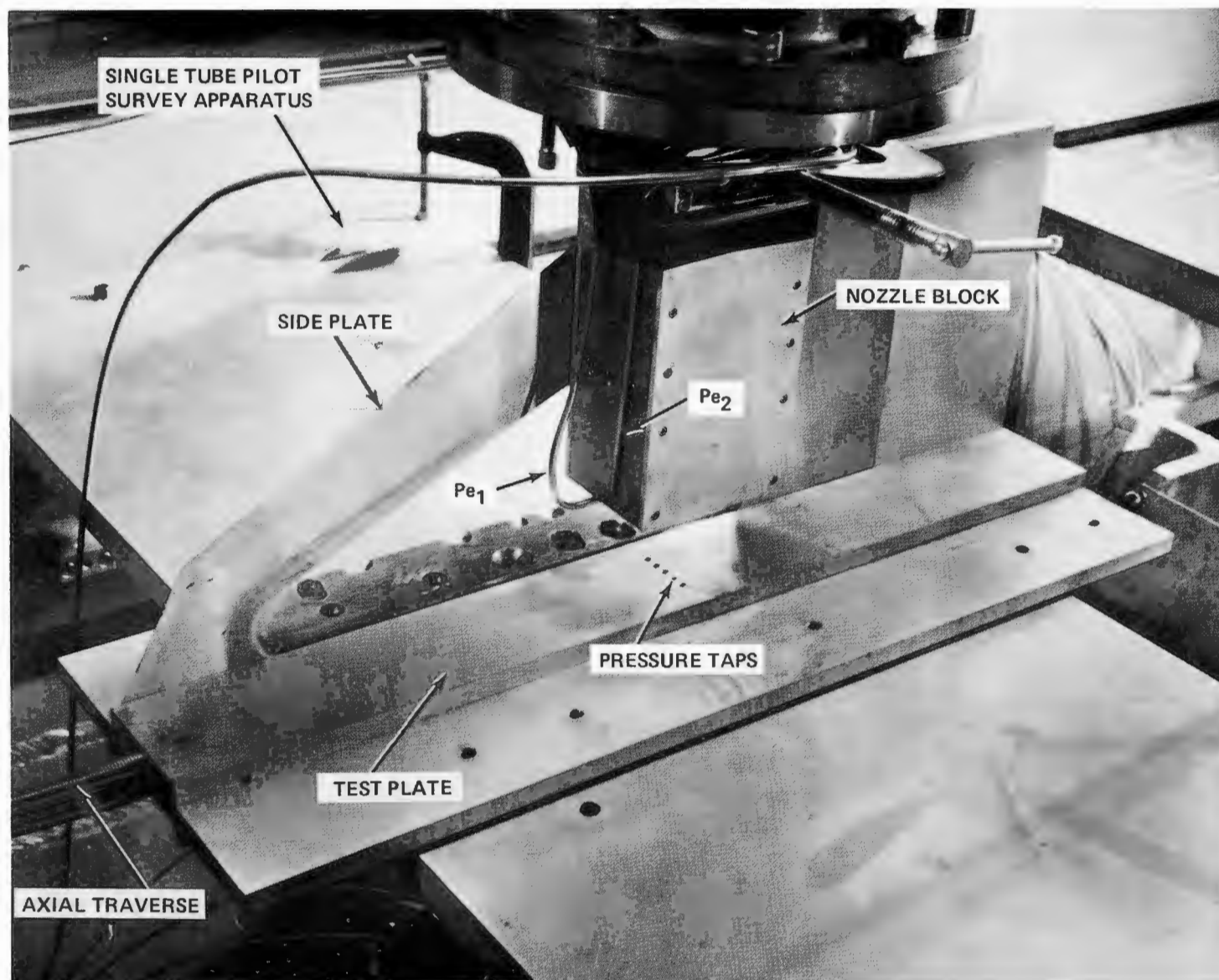
FIGURE 4 a EXPERIMENTAL SETUP
