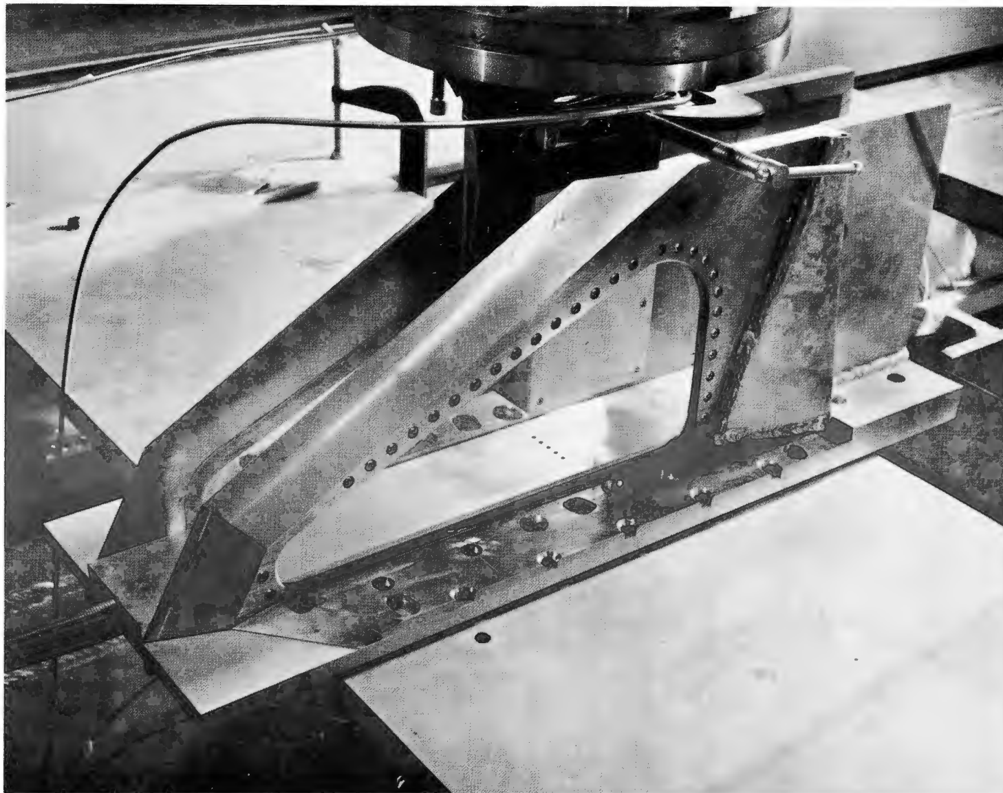
FIGURE 4b THE NOZZLE-PLATE ASSEMBLY FOR IMPINGEMENT FLOW STUDY
