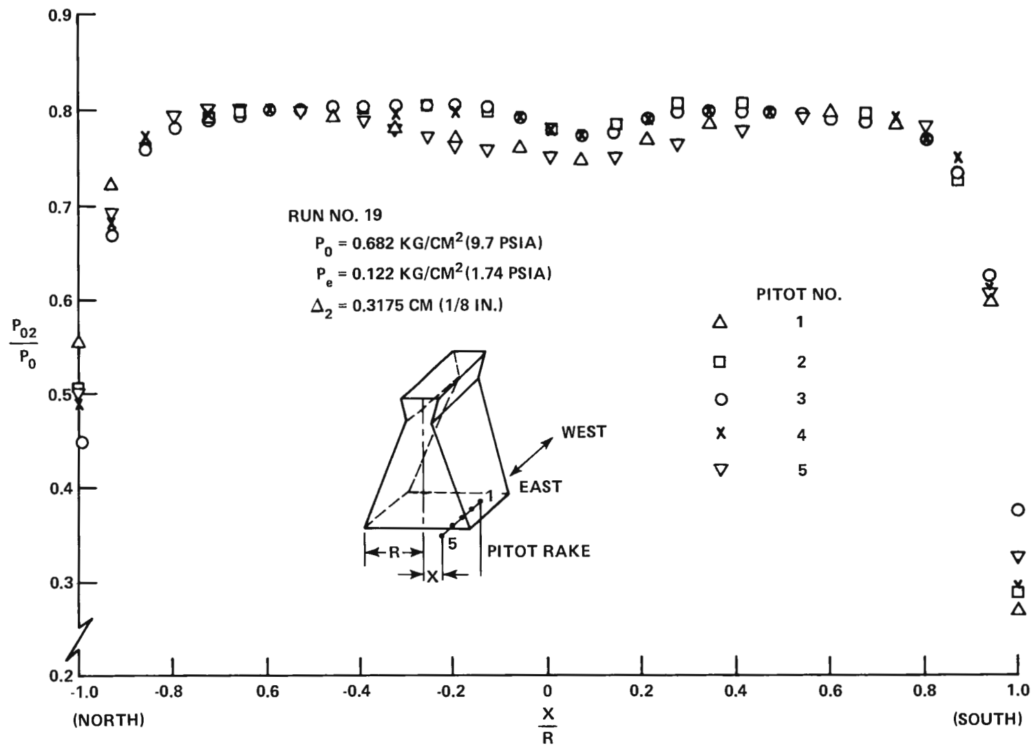
FIGURE 6 PITOT SURVEY - NOZZLE NO. 1
