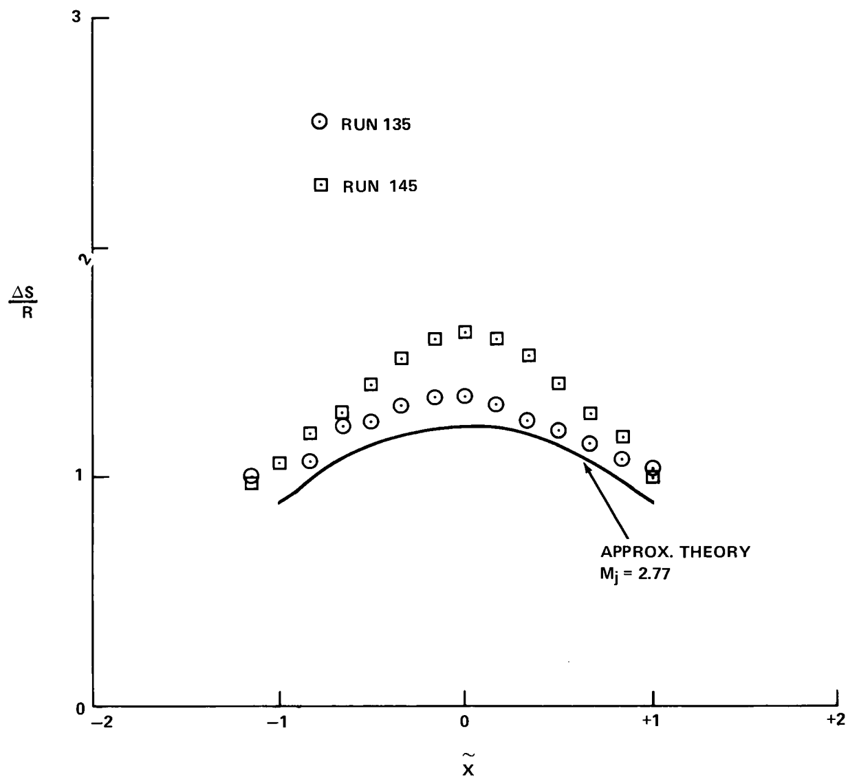
FIGURE 37 SHOCK MEASUREMENTS: NOZZLE NO. 2
