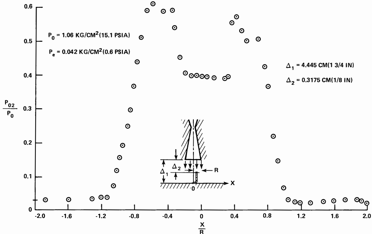
FIGURE 38a. PITOT SURVEY — PITOT-PLATE CONFIGURATION NOZZLE NO. 2 (RUN NO. 40)
