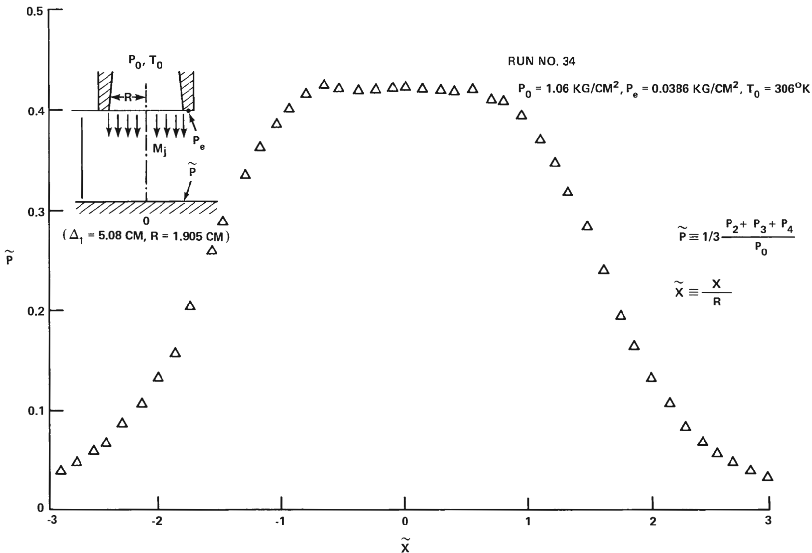
FIGURE 34 SURFACE PRESSURE RESULTS: NOZZLE NO. 2 (NEARLY ISENTROPIC JET)
