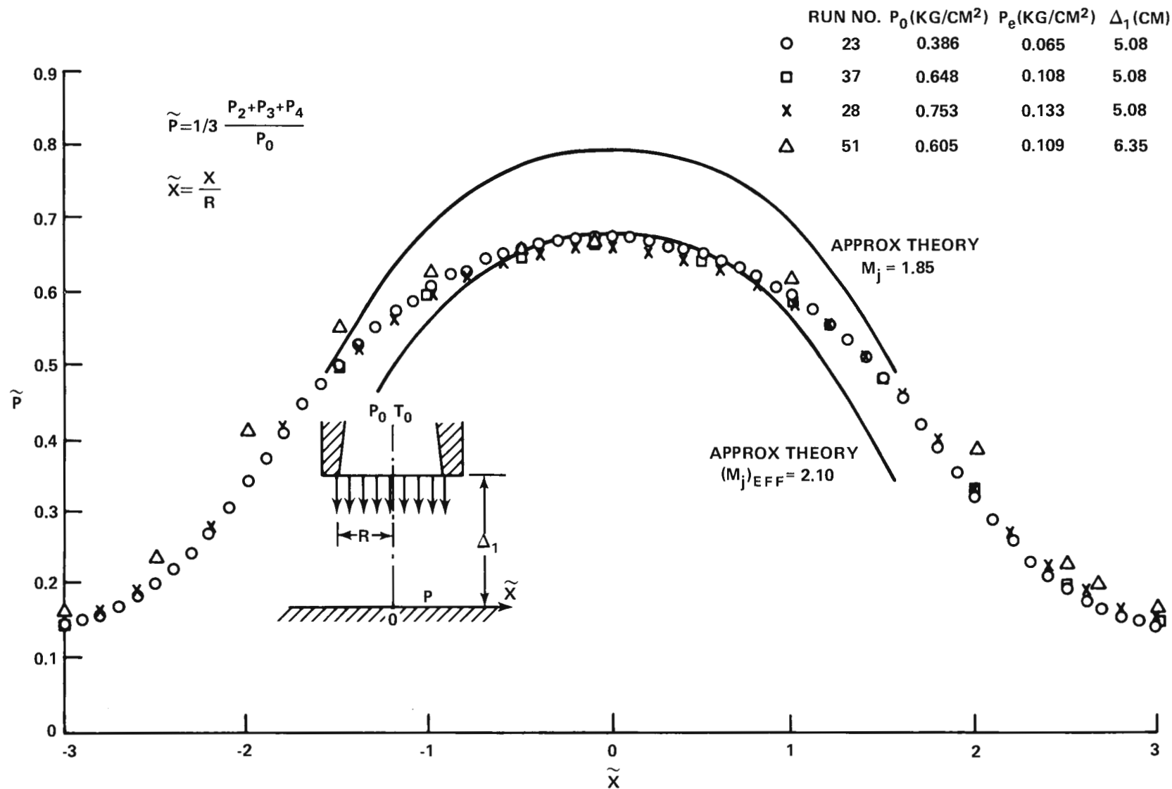
FIGURE 16 SURFACE PRESSURE RESULTS: NOZZLE NO. 1 (NEARLY ISENTROPIC JET)
