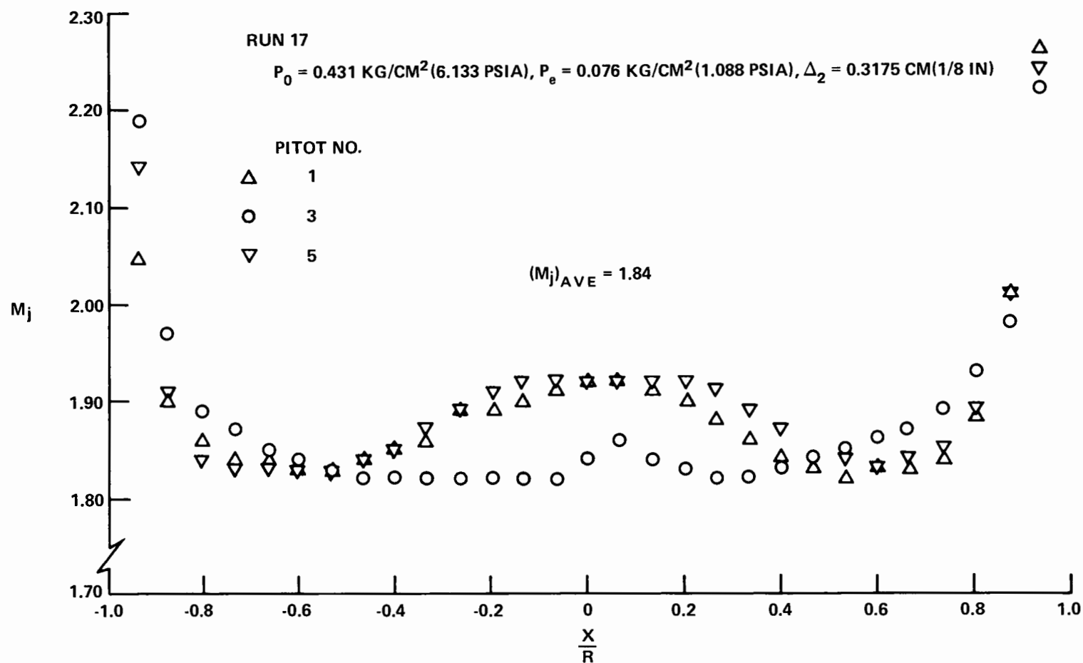
FIGURE 10 FREE JET MACH NO. — NOZZLE NO. 1 (PITOT SURVEY)
