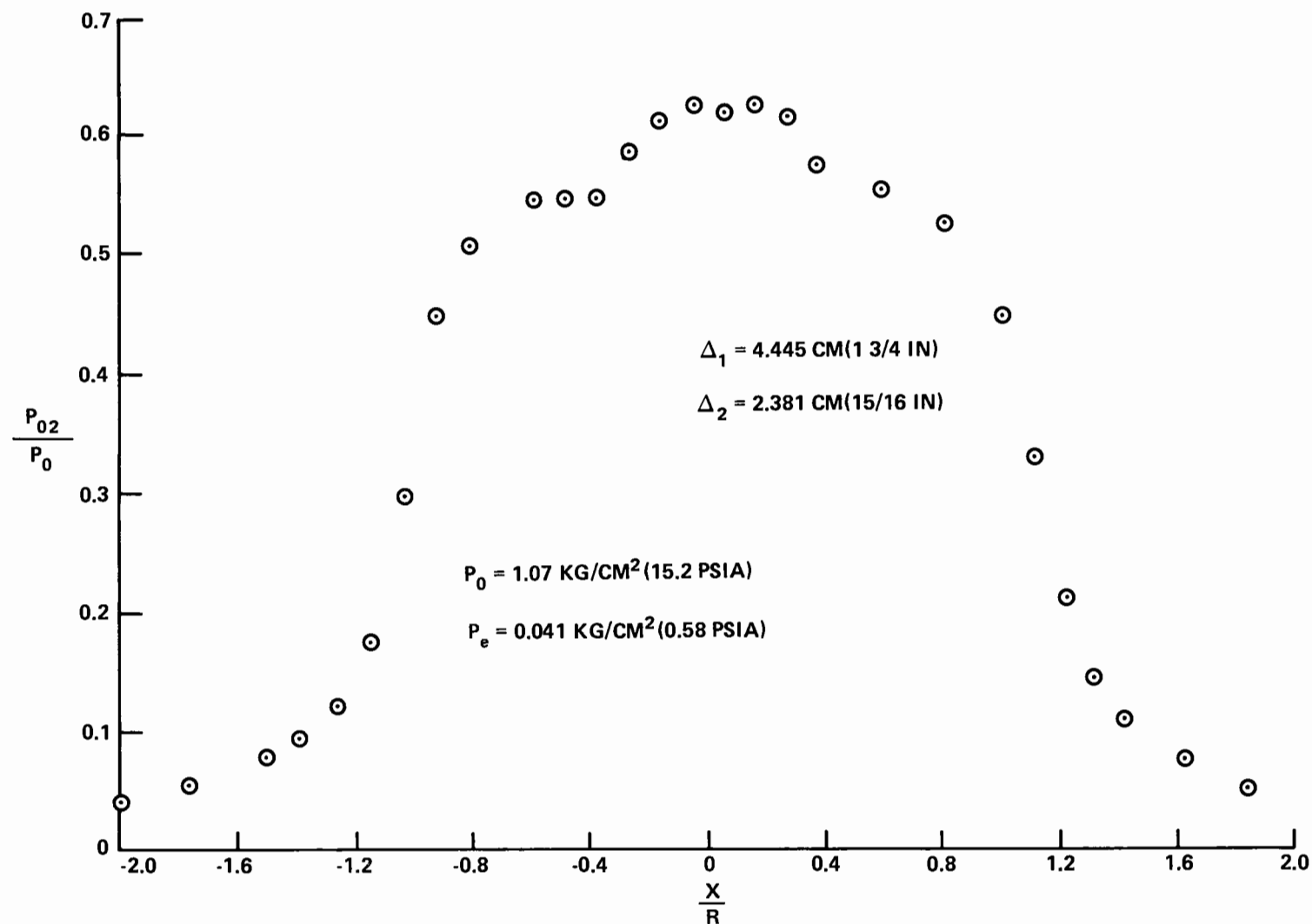
FIGURE 41a. PITOT SURVEY — PITOT -PLATE CONFIGURATION NOZZLE NO. 2 (RUN NO. 44)
