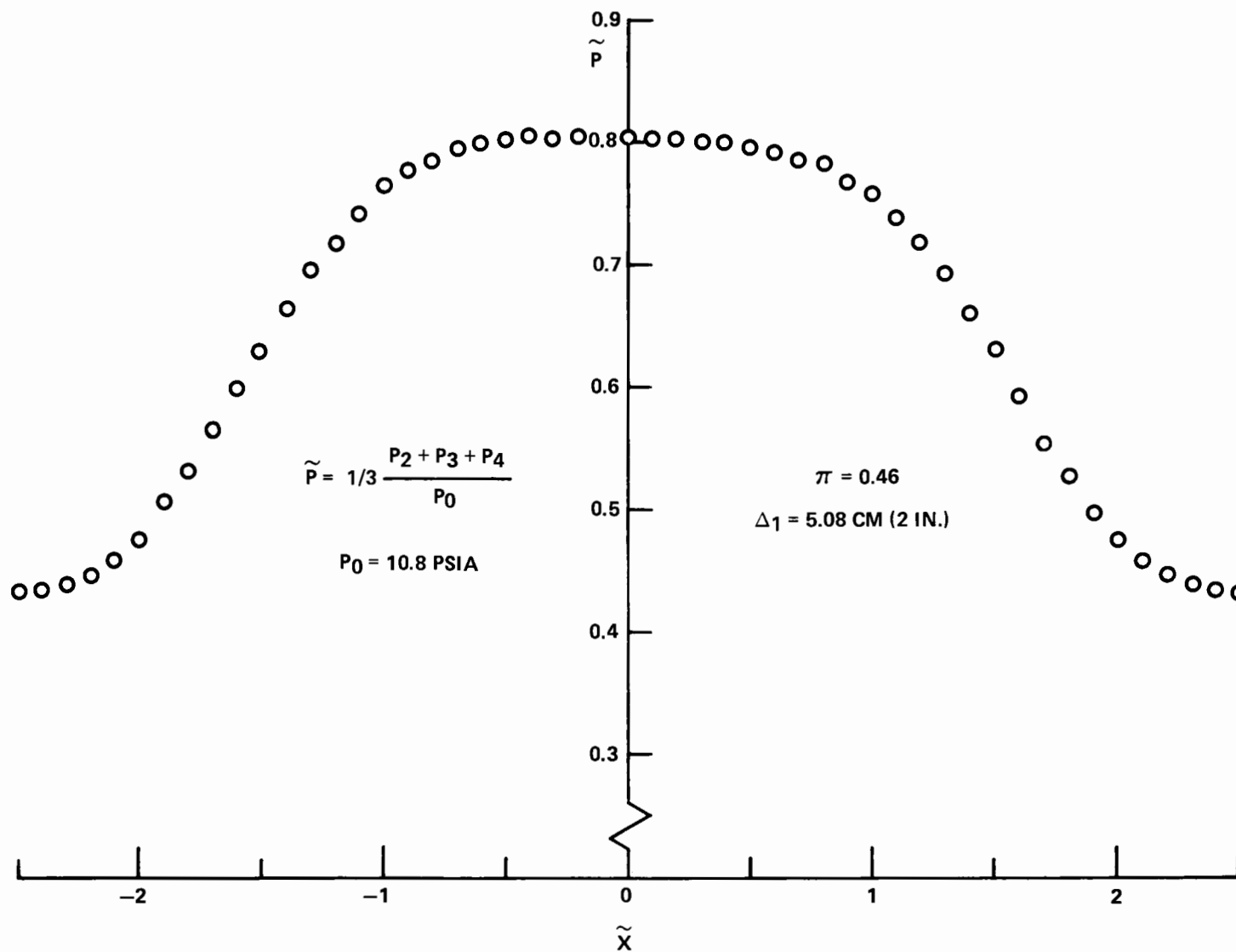
FIGURE 22 SURFACE PRESSURE RESULTS: NOZZLE NO. 1 (OVEREXPANDED JET, \pi = 0.46 )
