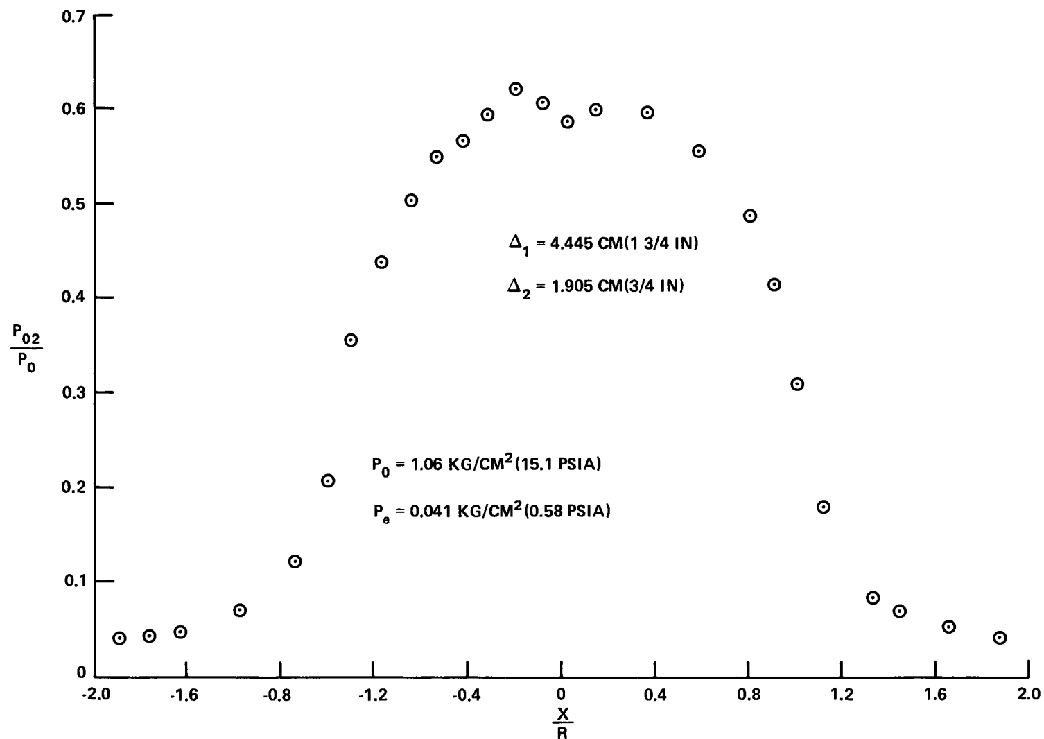
FIGURE 40a. PITOT SURVEY – PITOT-PLATE CONFIGURATION NOZZLE NO. 2 (RUN NO. 43)
