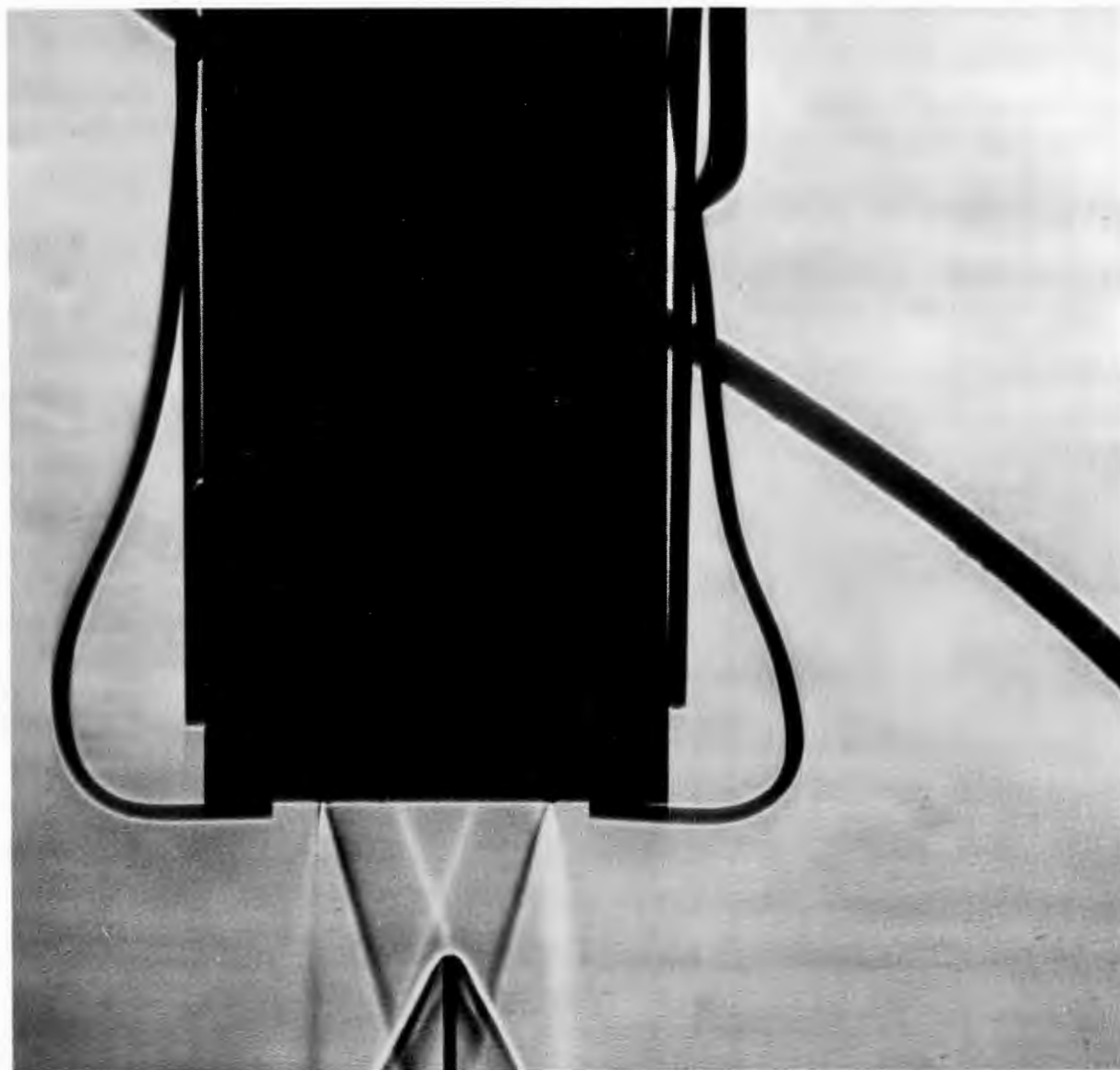
FIGURE 31 SCHLIEREN PHOTOGRAPH OF PITOT SURVEY: NOZZLE NO. 2 (RUN 9)
