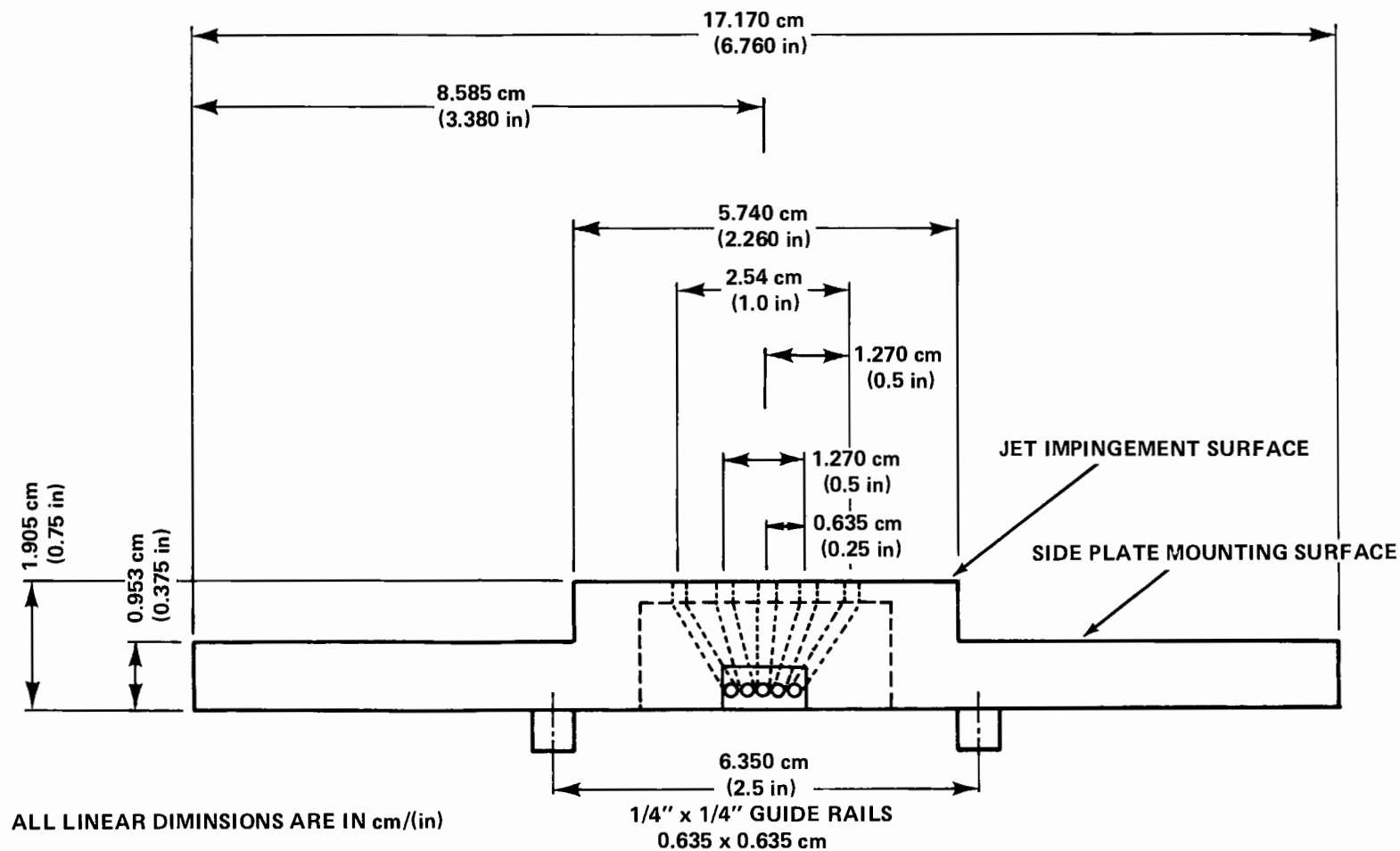
FIGURE 3 END VIEW OF SLIDING FLAT PLATE (WITHOUT SIDE PLATES) SHOWING STATIC SURFACE PRESSURE TAPS(0.0625 OD STAINLESS STEEL TUBING).
