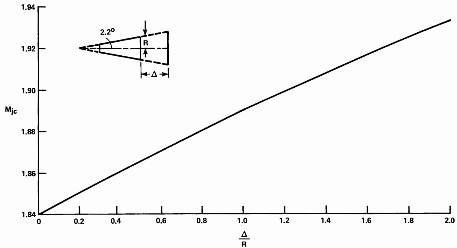
FIGURE 43 MACH NO. CORRECTION - NOZZLE NO. 1
