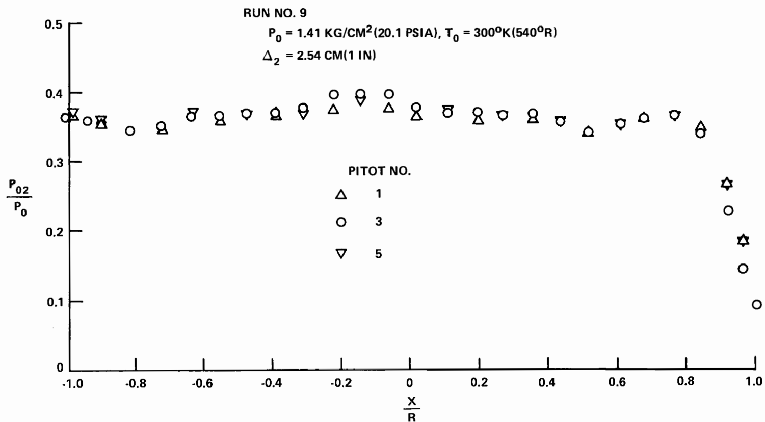
FIGURE 24 PITOT SURVEY - NOZZLE NO. 2
