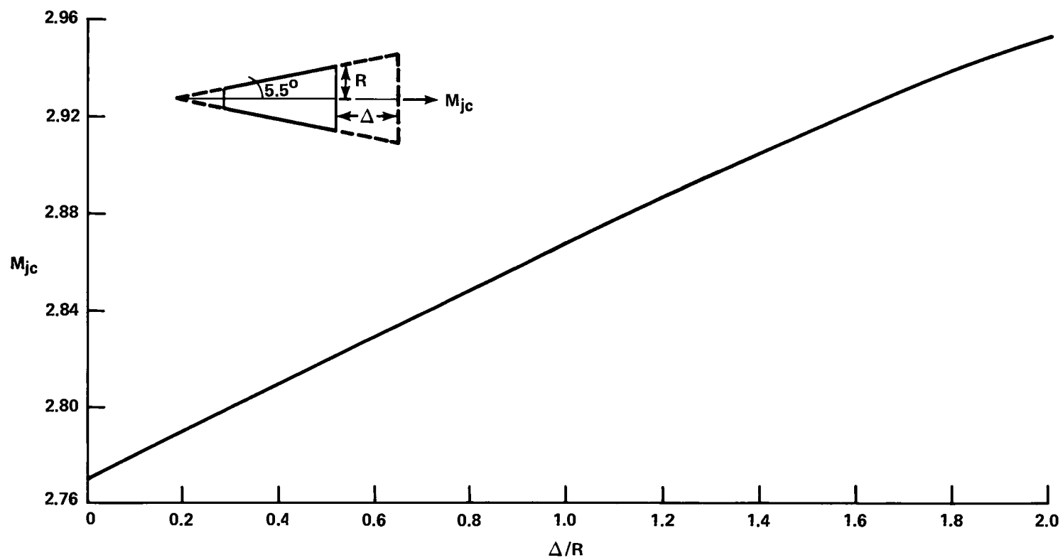
FIGURE 44 MACH NO. CORRECTION — NOZZLE NO. 2
