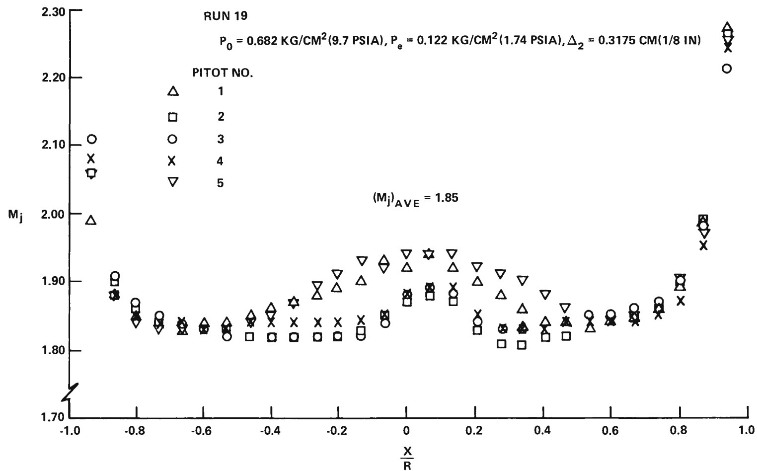
FIGURE 8 FREE JET MACH NO. — NOZZLE NO. 1 (PITOT SURVEY)
