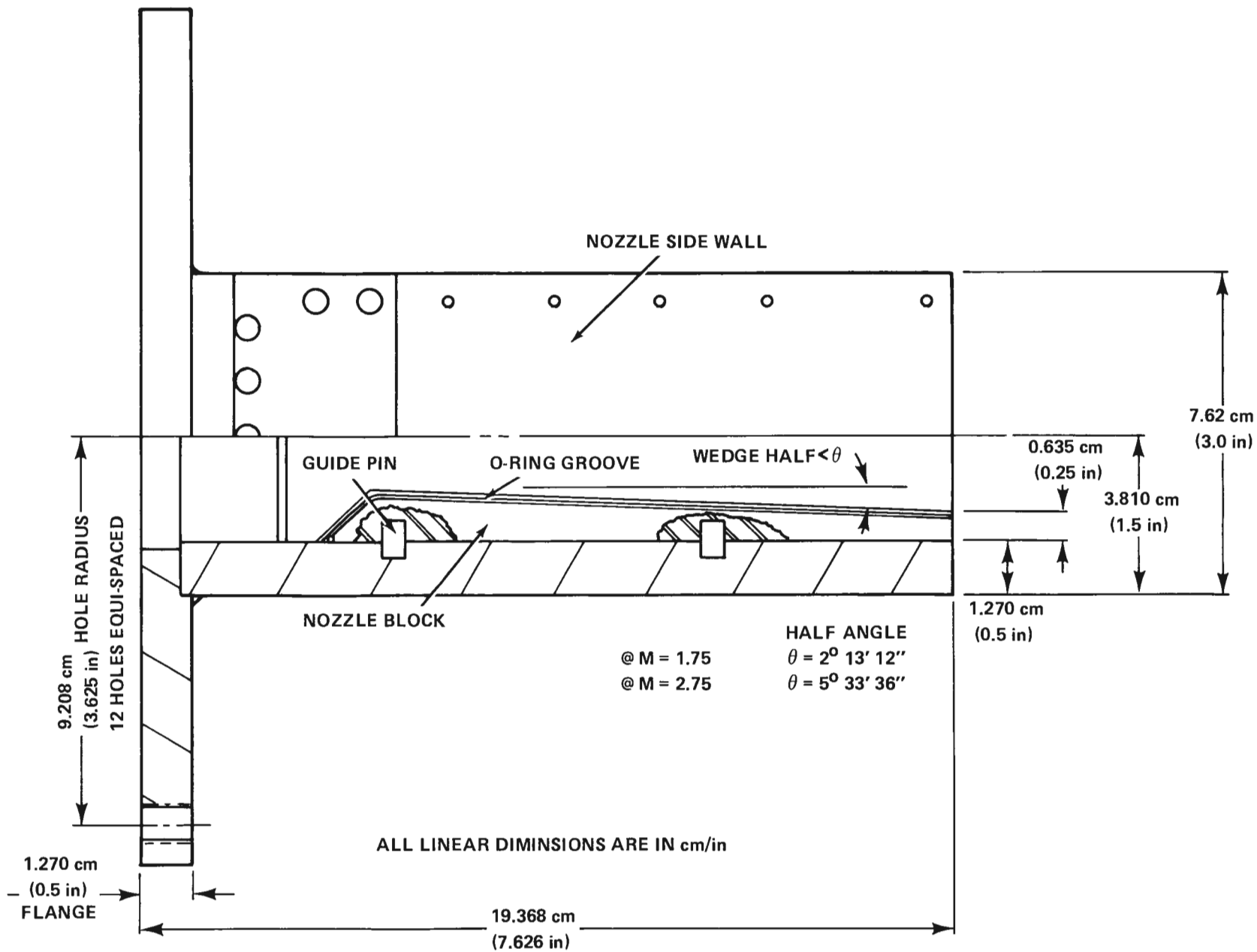
FIGURE 2 SKETCH OF NOZZLE BLOCK HOLDER SHOWING THE HALF-SECTIONED SIDE VIEW OF THE M = 1.75 NOZZLE BLOCK
