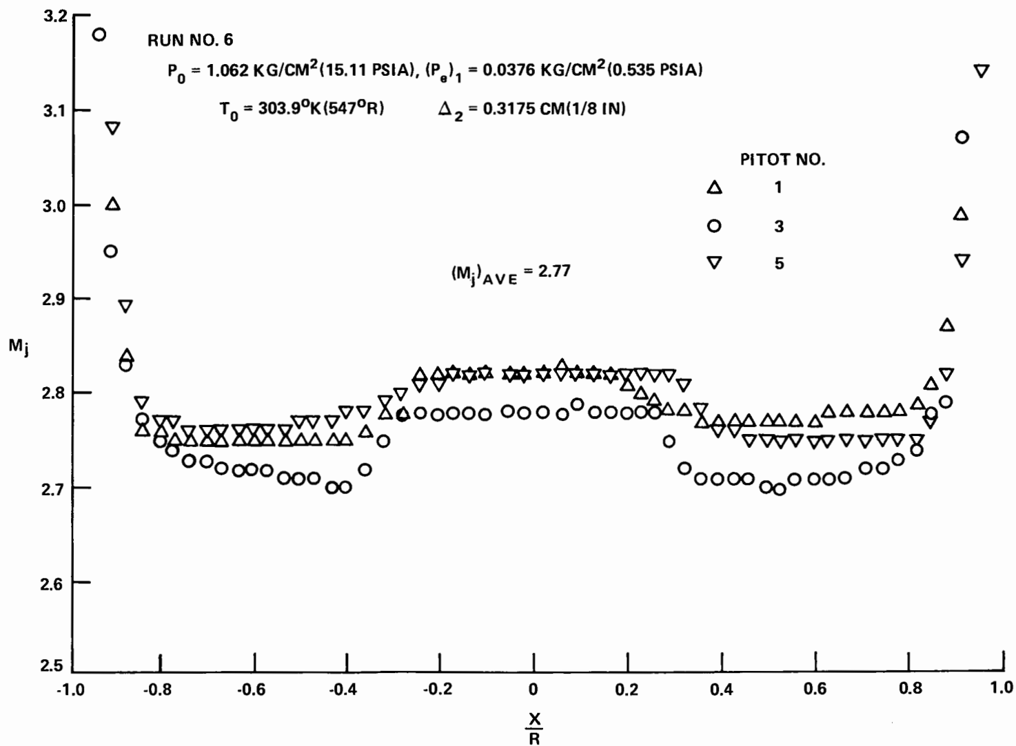
FIGURE 26 FREE JET MACH NO. - NOZZLE NO. 2 (PITOT SURVEY)
