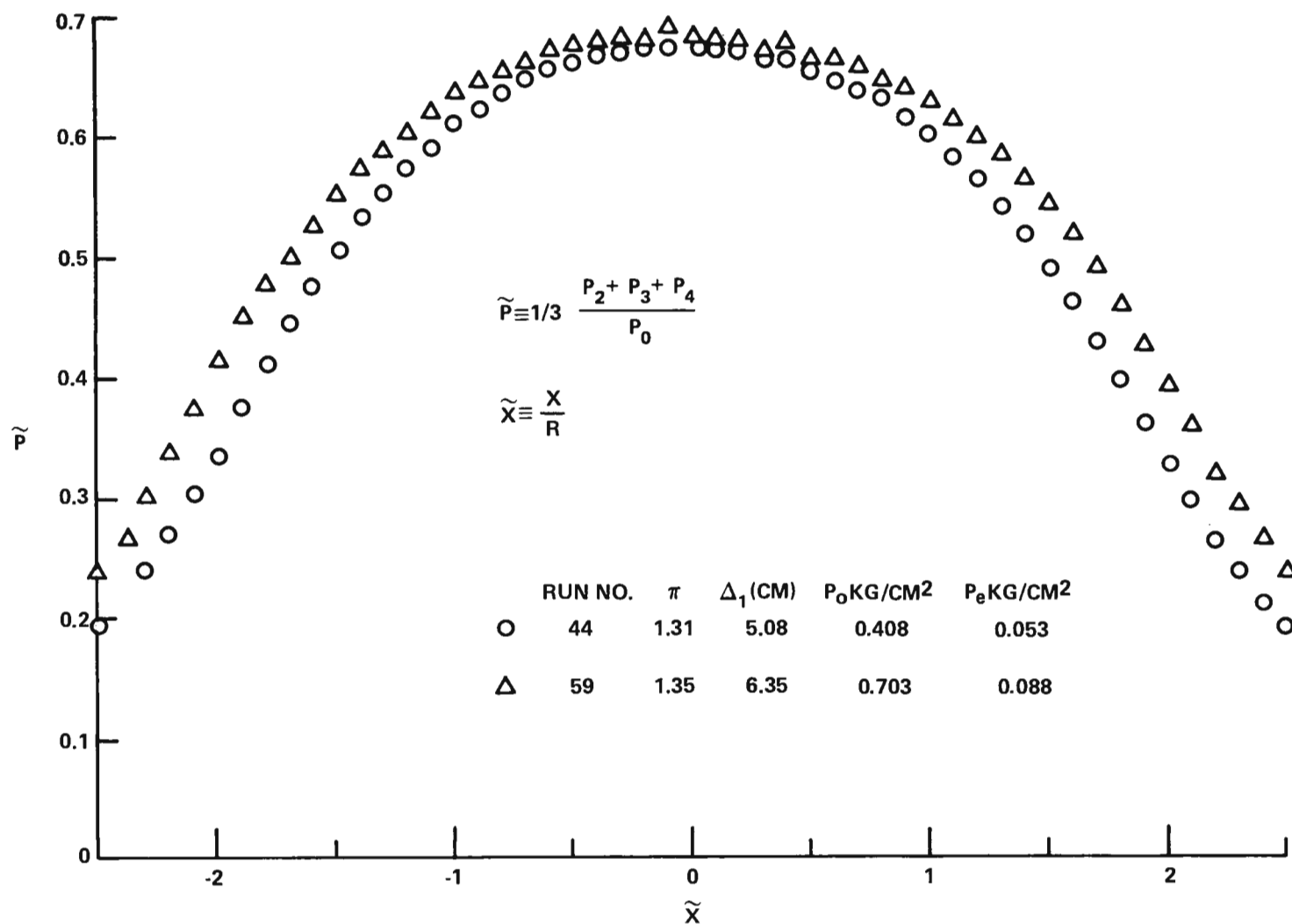
FIGURE 21 EFFECTS OF NOZZLE - PLATE DISTANCE ON SURFACE PRESSURE: UNDEREXPANDED JET (NOZZLE NO. 1)
