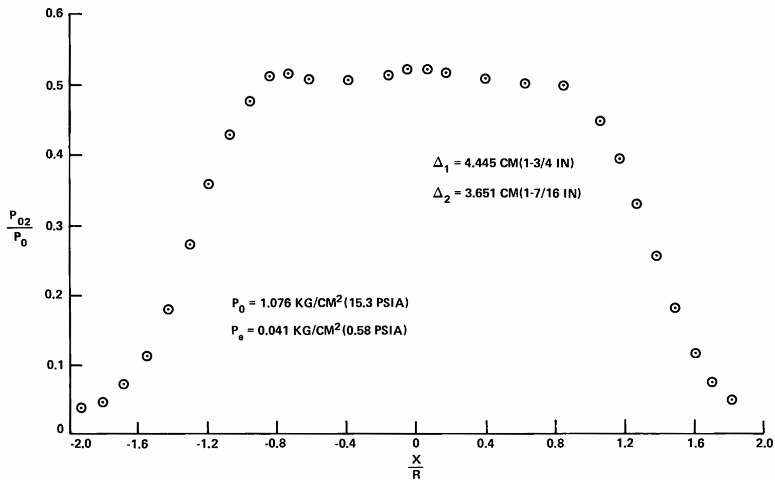
FIGURE 42 PITOT SURVEY – PITOT-PLATE CONFIGURATION – NOZZLE NO. 2 (RUN NO. 45)
