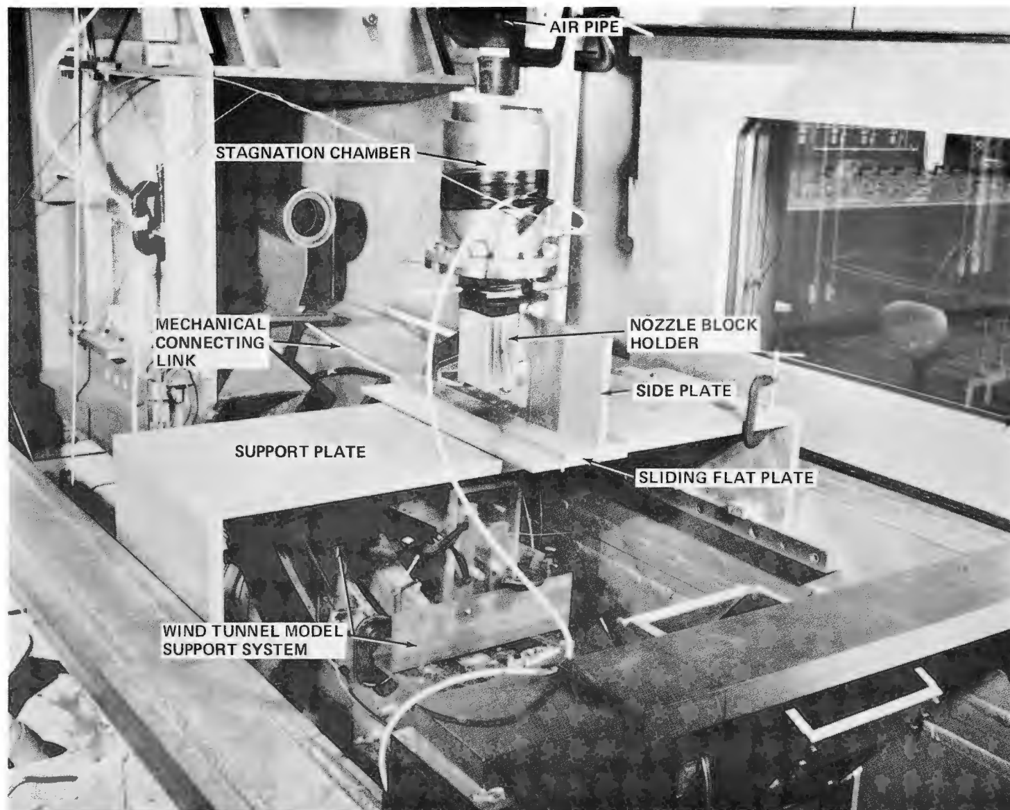
FIGURE 5 OVERVIEW OF THE JET IMPINGEMENT APPARATUS (LEFT SIDE PLATE REMOVED)
