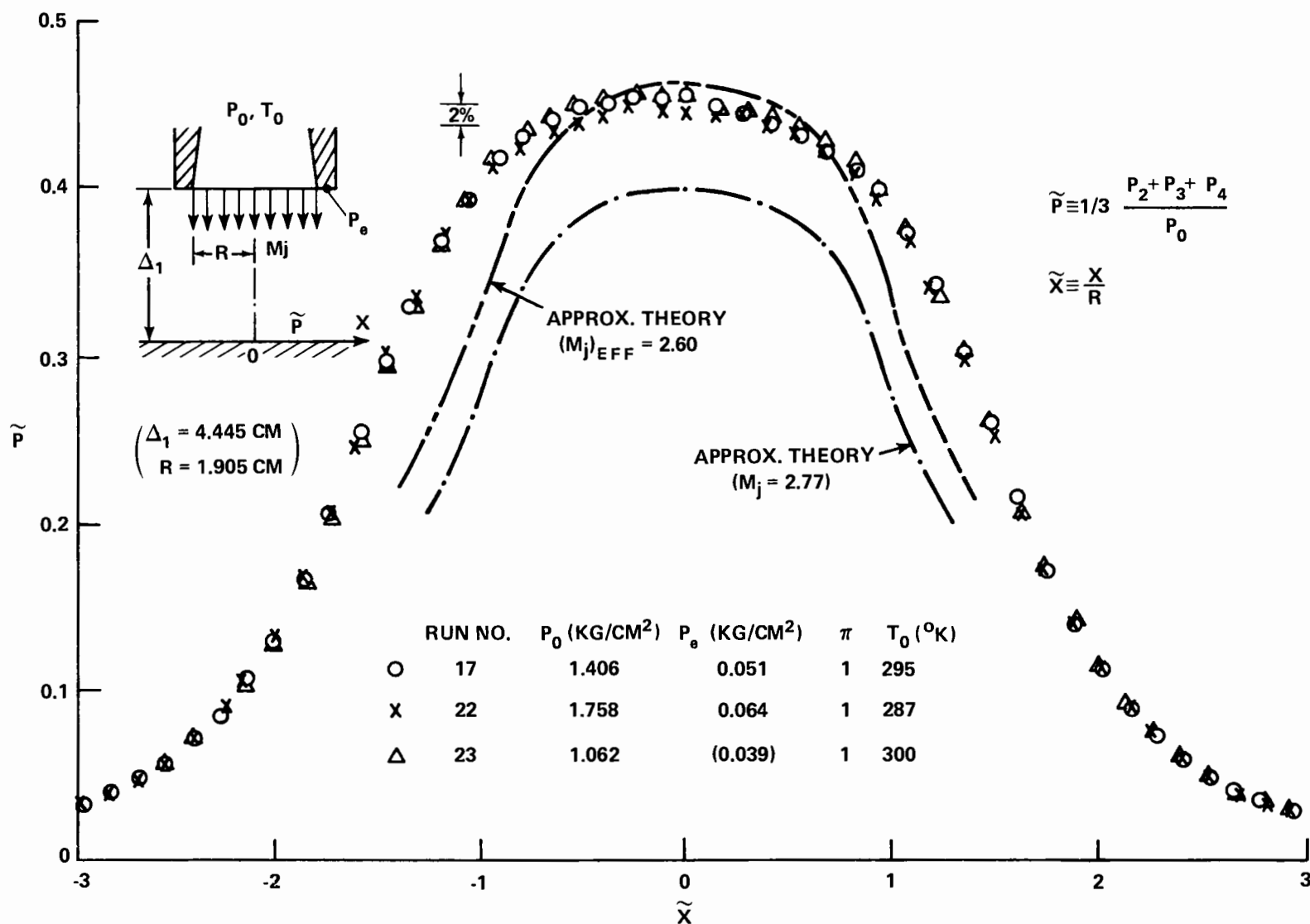
FIGURE 33 SURFACE PRESSURE RESULTS: NOZZLE NO. 2 (NEARLY ISENTROPIC JET)
