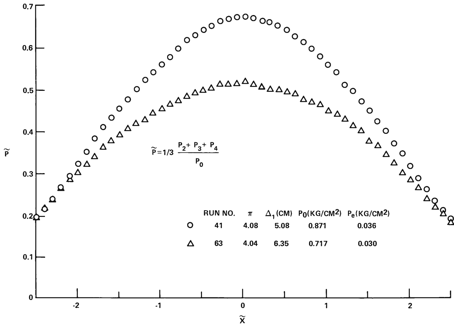
FIGURE 20 EFFECTS OF NOZZLE — PLATE DISTANCE ON SURFACE PRESSURE: UNDEREXPANDED JET (NOZZLE NO. 1)
