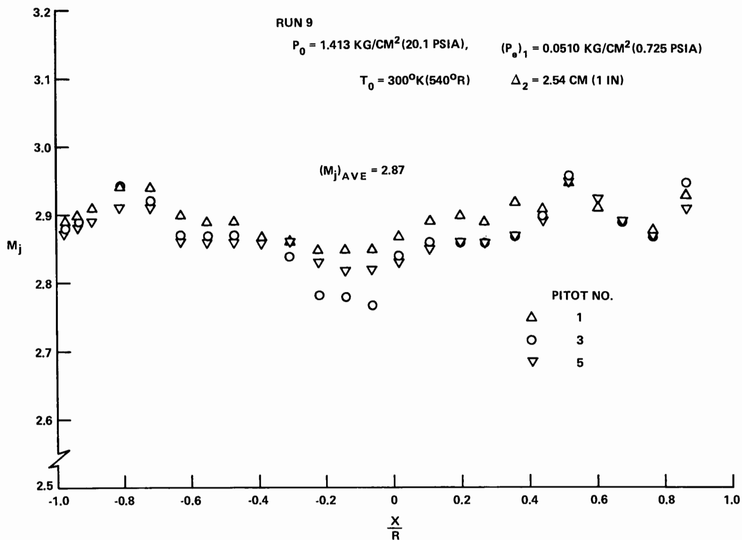
FIGURE 27 FREE JET MACH NO. - NOZZLE NO. 2 (PITOT SURVEY)
