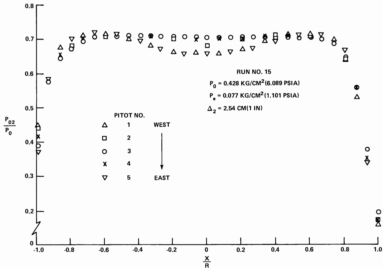
FIGURE 7 PITOT SURVEY – NOZZLE NO. 1
