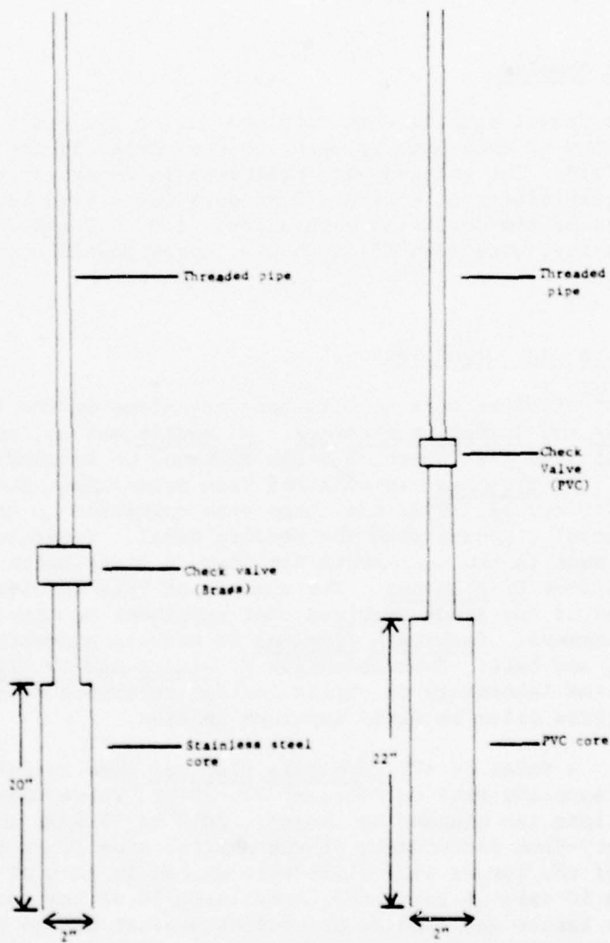
FIGURE 5-4. COLLECTION APPARATUS FOR SETTLING PARTICULATES
