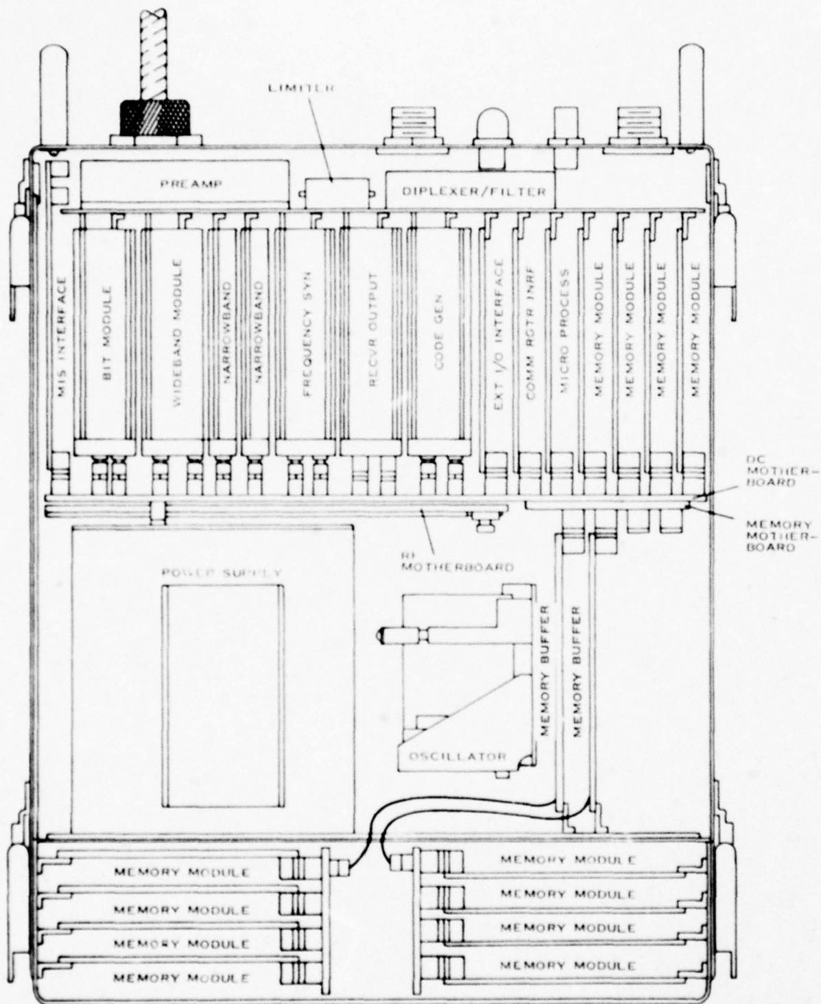
Figure 4.1.10-1. RAM Receiver/Processor
