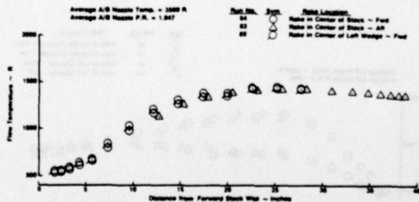
FIGURE 47: EXIT FLOW VELOCITY, MACH NUMBER AND TEMPERATURE PROFILE - SHORT EXHAUST STACK WITH DUAL WEDGE CONFIGURATION
