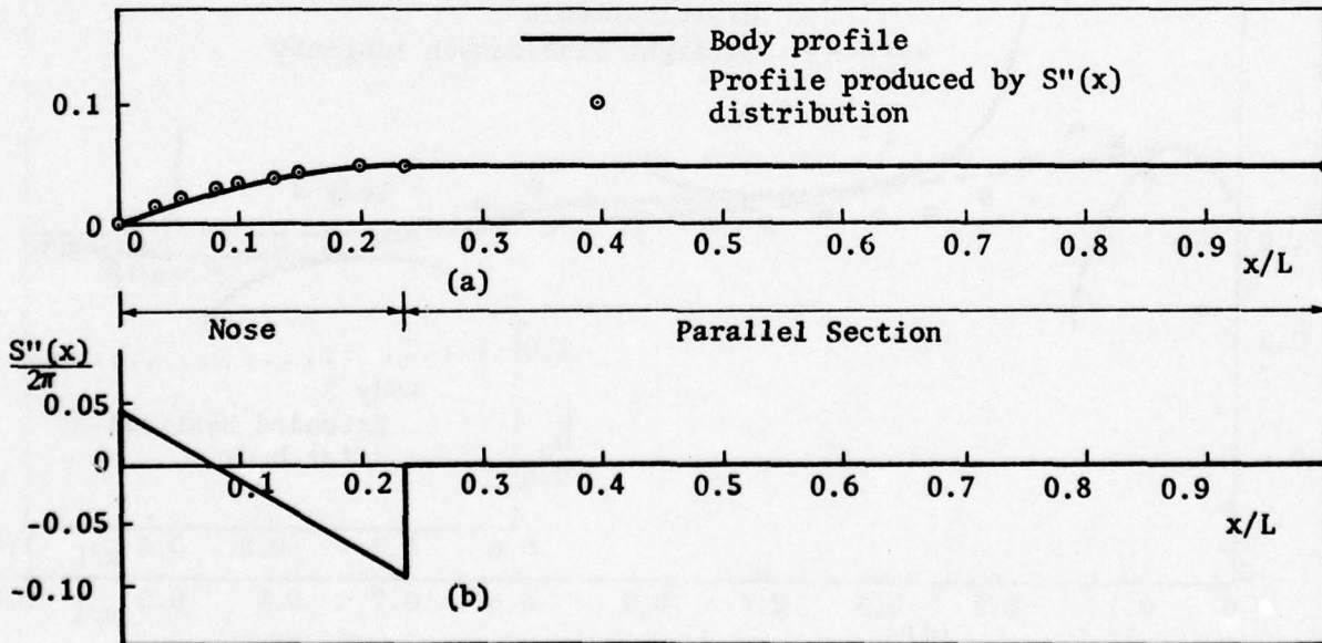
(a) Body profile (b) S''(x) distribution
