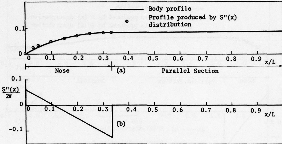
(a) Body profile (b) S''(x) distribution
