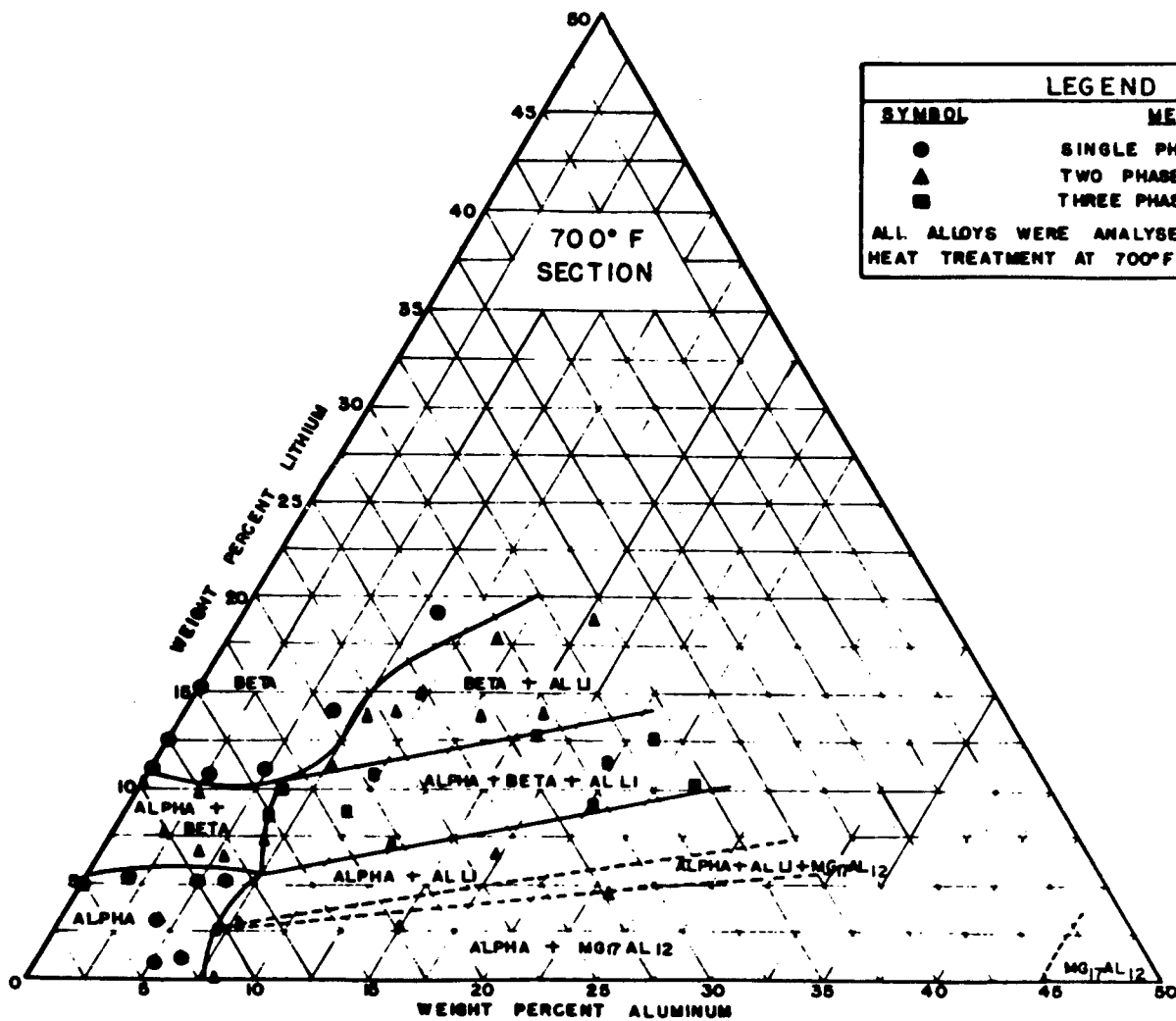
FIGURE 16 PHASE BOUNDARIES IN THE MAGNESIUM CORNER OF THE MAGNESIUM-LITHIUM-ALUMINUM SYSTEM AT 700° F
